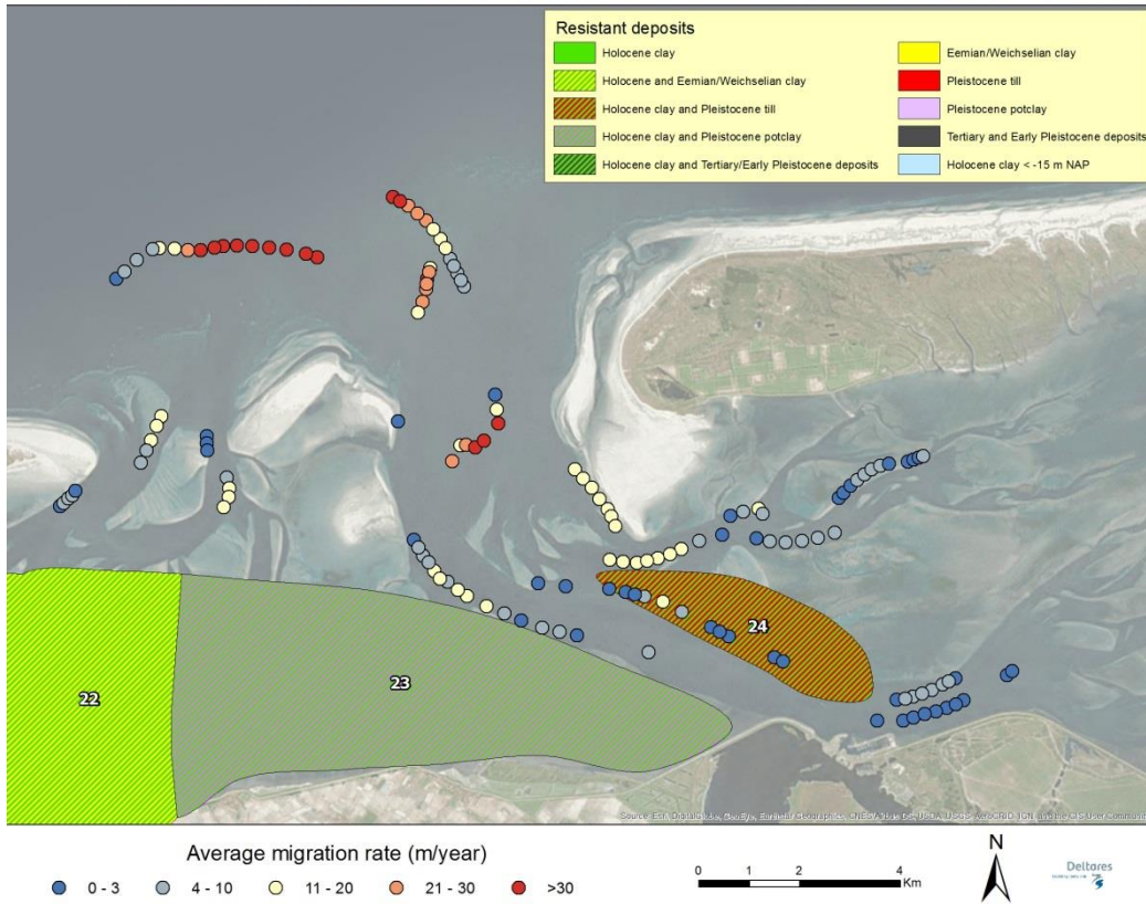
Average migration rate (m/year) of the -15 m NAP contourline and the distribution of resistant deposits
