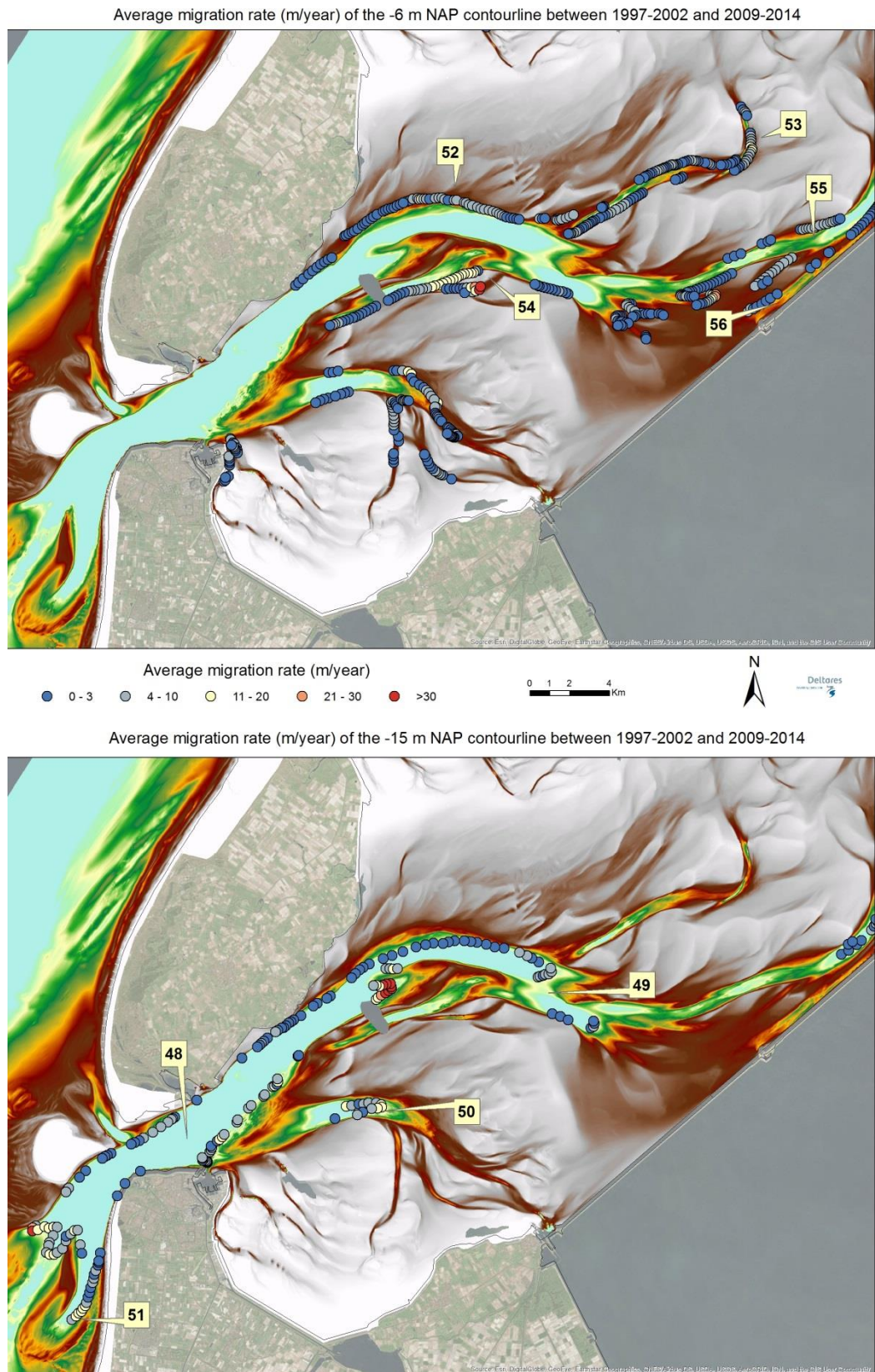
Figure 4.10 Average migration rates for the Texel inlet between 1997-2002 and 2009-2014.
