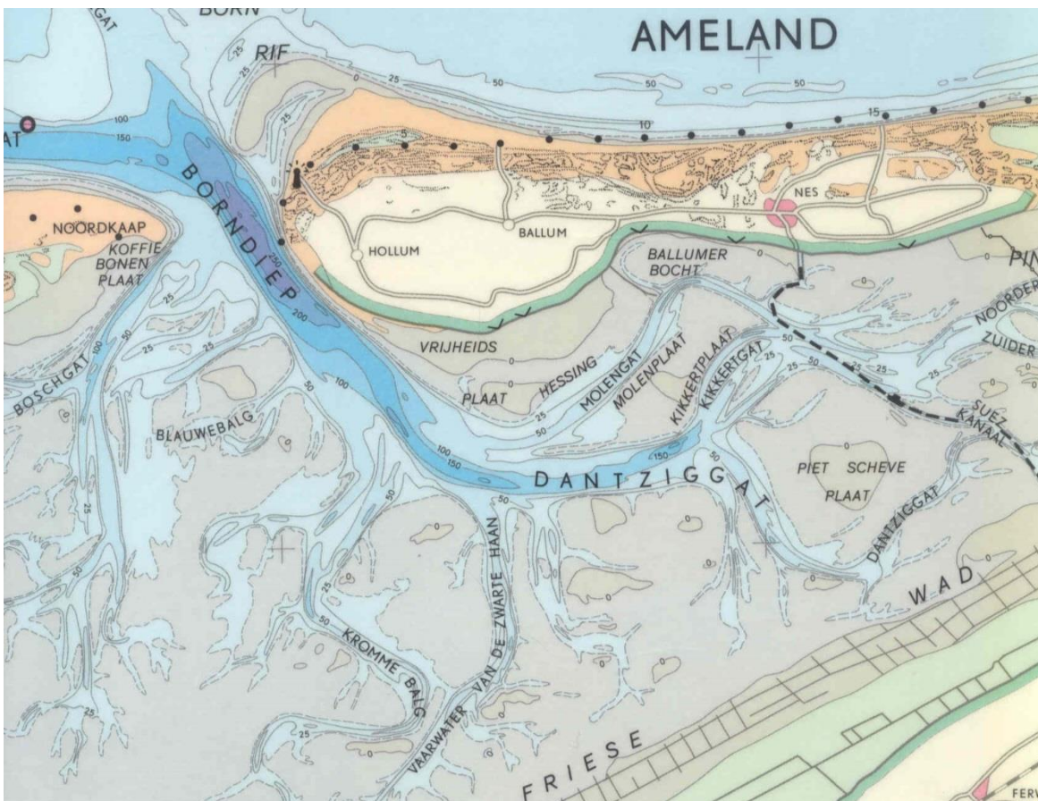
Figure 4.4 Map of the Borndiep inlet.
