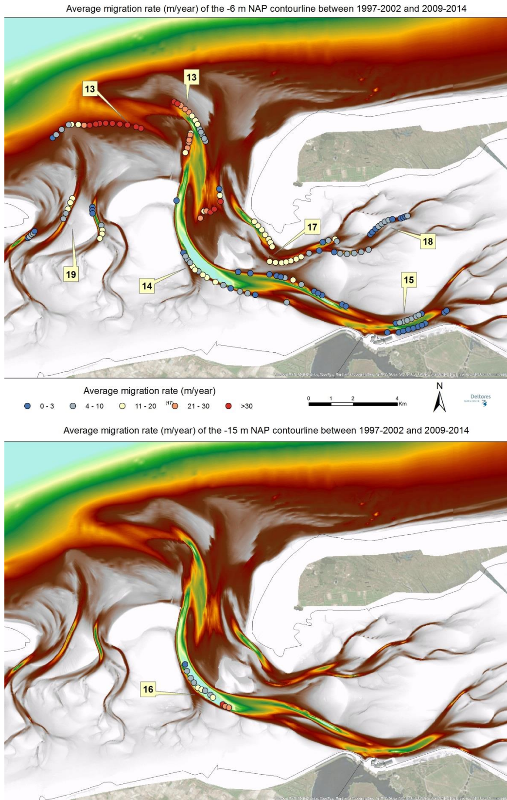
Figure 4.5 Average migration rates for the Friesche Zeegat between 1997-2002 and 2009-2014.
