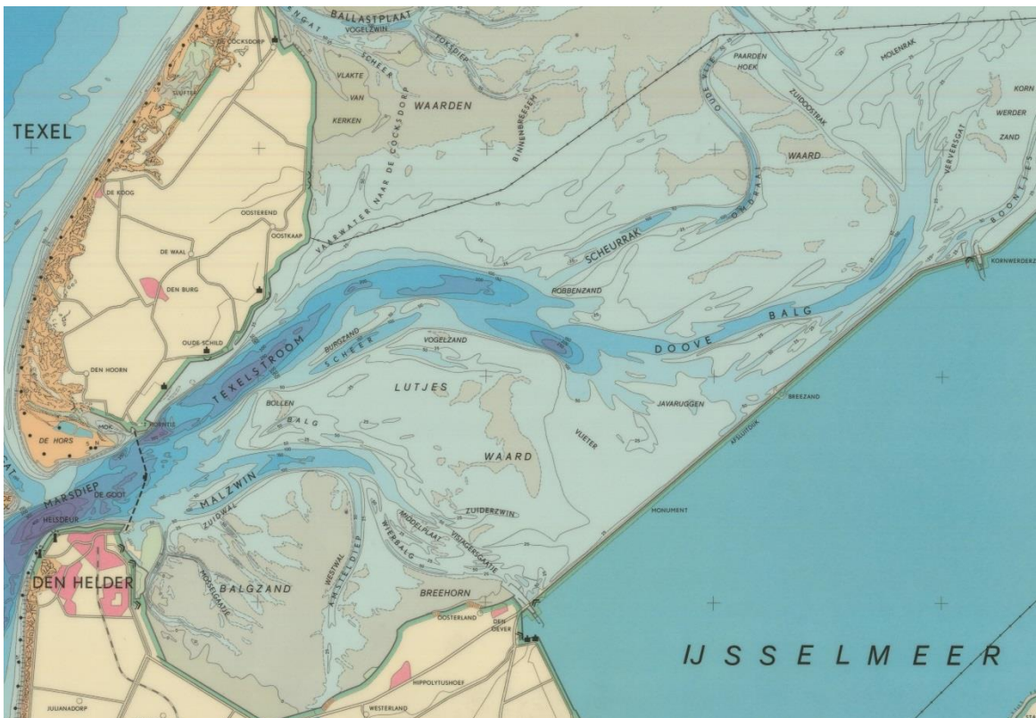
Figure 4.9 Map of the Texel inlet
