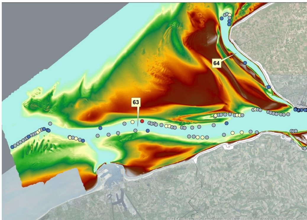
Figure 4.12 Average migration rates for the mouth of the Westerschelde between 1997-2002 and 2009-2014.
