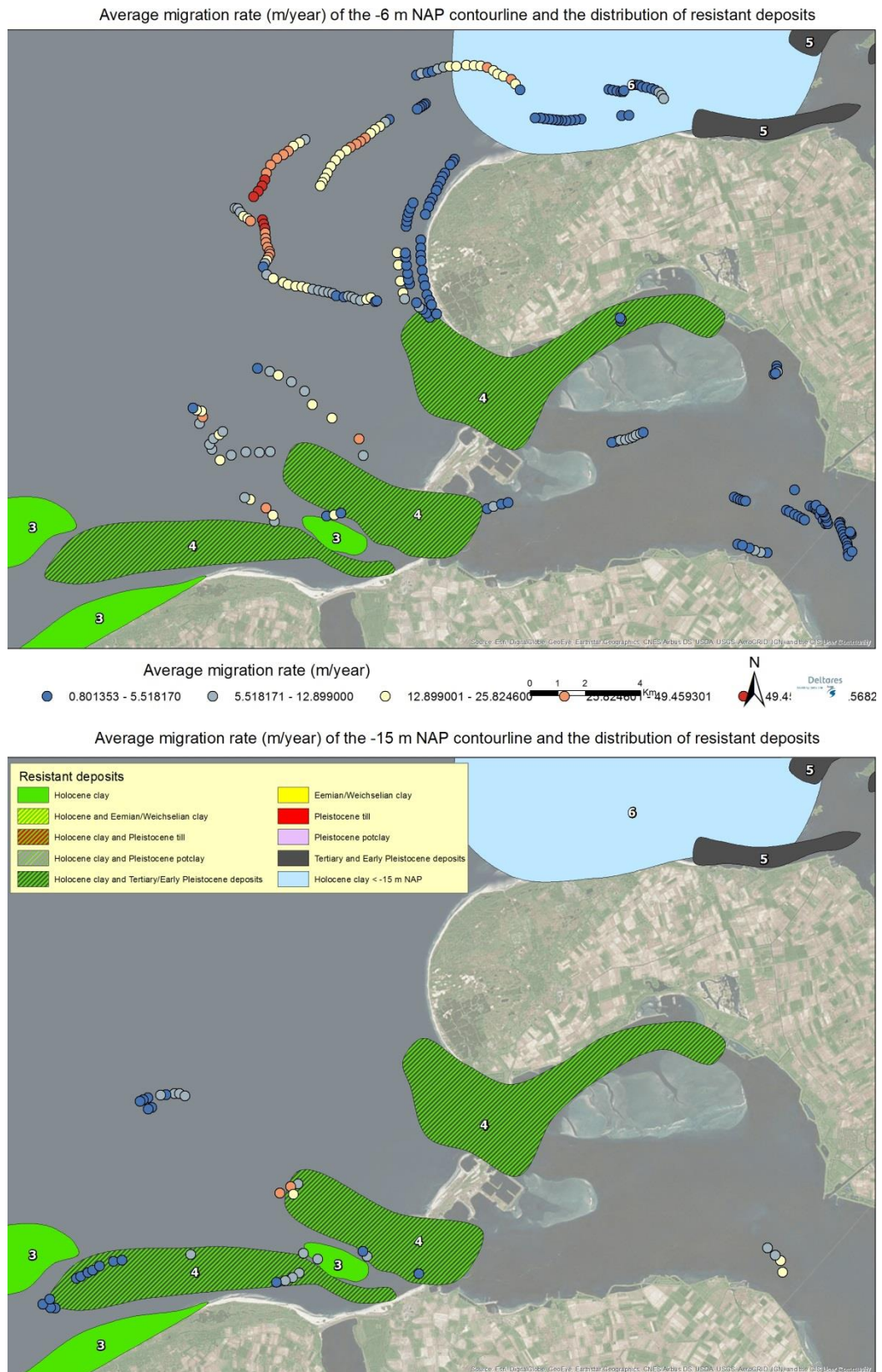
Figure 5.9 Average migration rates for the Oosterschelde-Grevelingen region and the distribution of resistant deposits.
