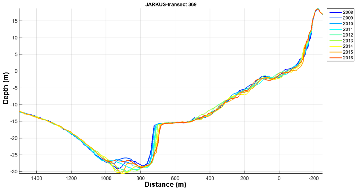
Figure 2.2 Channel profiles through time along a transect across the Nieuwe Schulpengat. On one side of the channel a clear staircase-profile is visible (see Figure 2.2, Panel B) that is attributed to the presence of erosion-resistant deposits.
