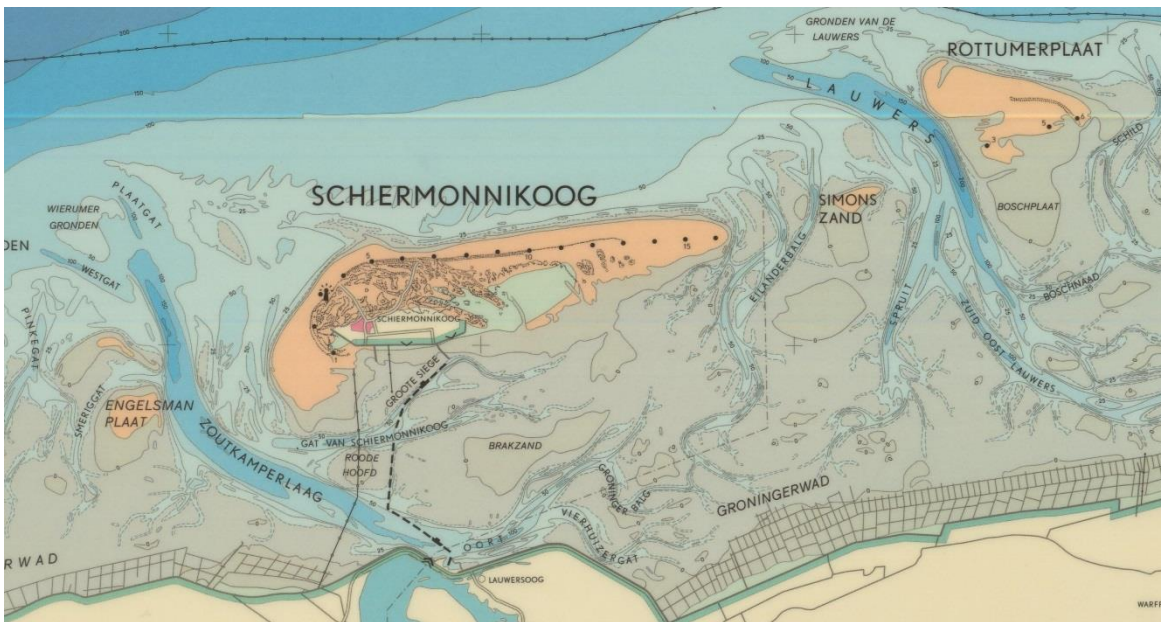
Figure 4.3 Map of the Friesche Zeegat and the Groninger Wad.
