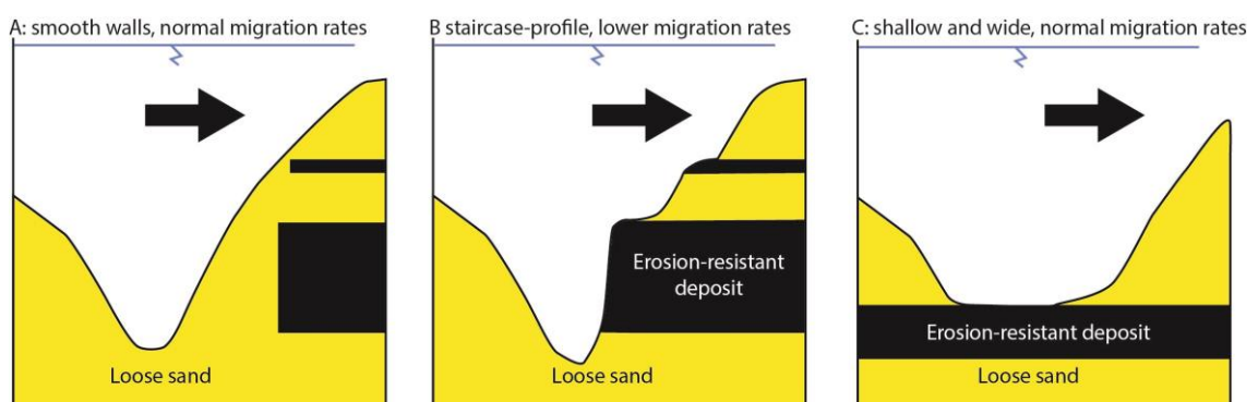
Figure 2.1 Conceptual model of the influence of erosion-resistant deposits on the shape of the channel profile.
