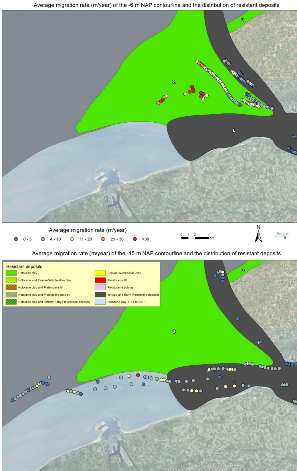
Figure 5.10 Average migration rates for the mouth of the Westerschelde and the distribution of resistant deposits.
