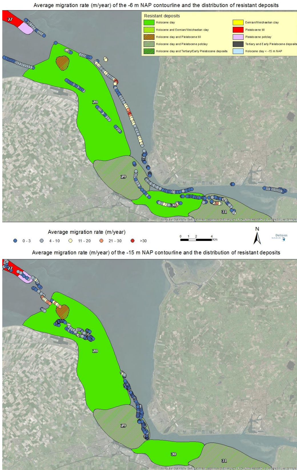
Figure 5.1 Average migration rates for the southern Eems-Dollard region and the distribution of resistant deposits.
