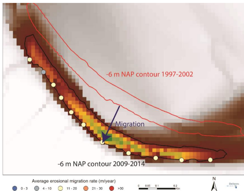
Figure 3.1 Example of the method used. Two contour lines are displayed: one from the period 1997-2002 (red) and one from the period 2009-2014 (black). On the 2009-2014 contour line points are created and the distance between the points and the 1997-2002 contour line is calculated ( 220 \pm 9.9 m in this case). The average migration rate is then calculated by dividing the distance by the elapsed time ( 12 \pm 0.5 years in this case), resulting in an average migration rate of 18 \pm 0.8 m/year.
