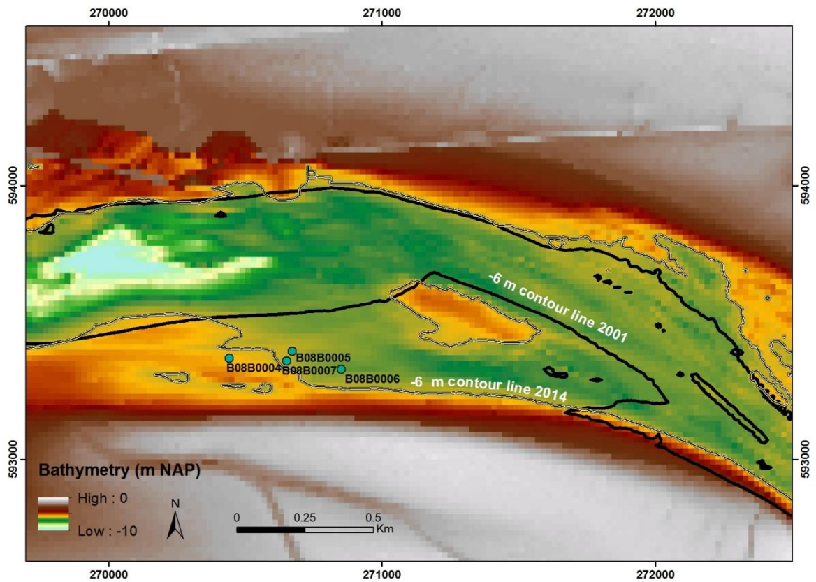
Figure 5.2 Close-up of the Mond van de Dollard-Groote Gat region with the two analysed contour lines from 2001 and 2014. In 13 years the contour line shifted more than 400 m in the central part of the figure, while to the west and east the rate of migration is low or sedimentation occurred.
