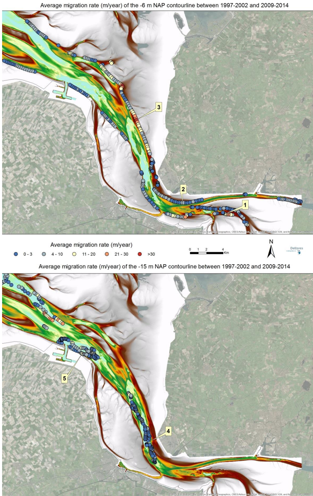
Figure 4.1 Average migration rates for the southern Eems-Dollard region between 1997-2002 and 2009-2014.
