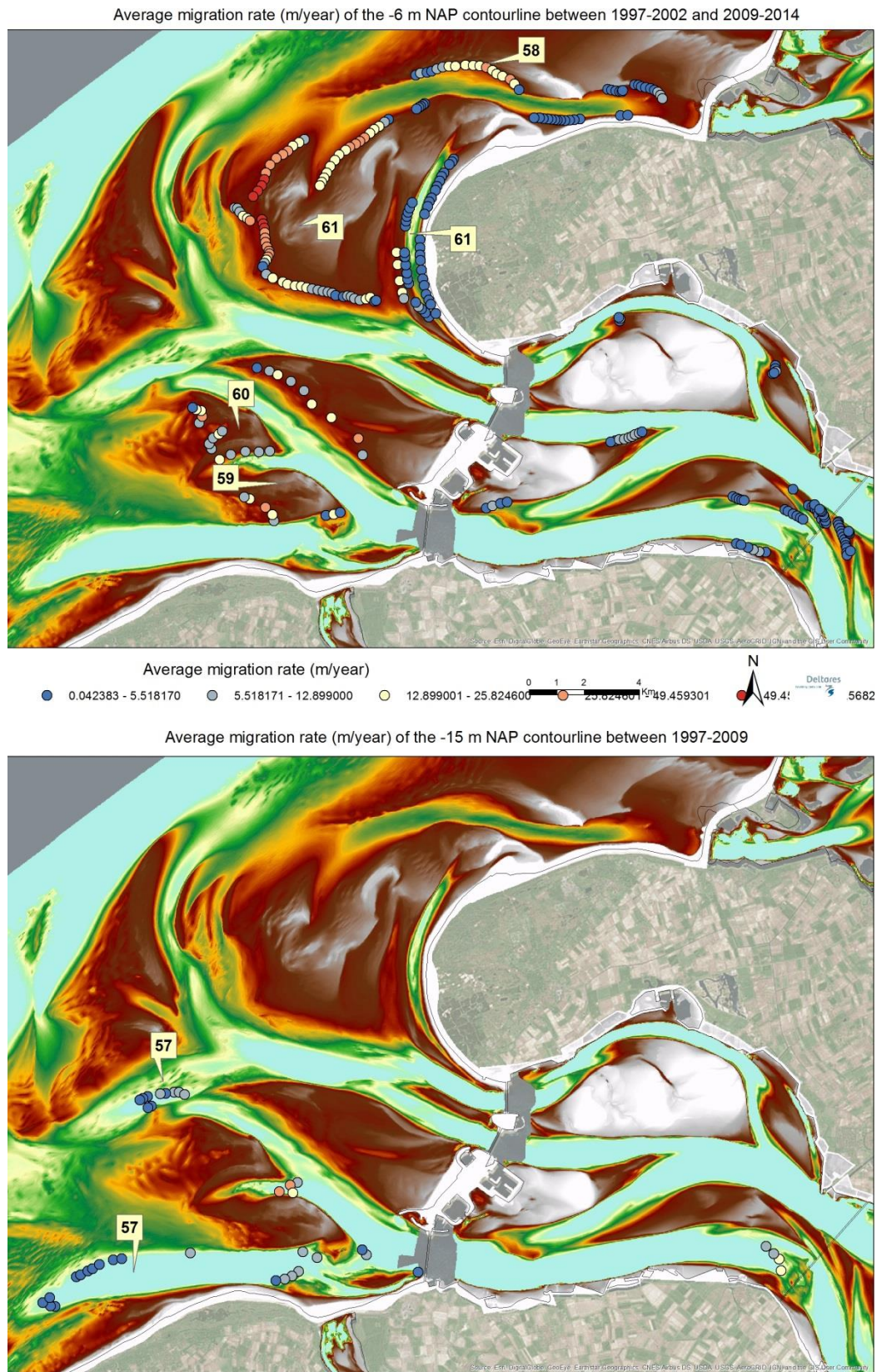
Figure 4.11 Average migration rates for the Oosterschelde-Grevelingen region between 1997-2002 and 2009-2014.
