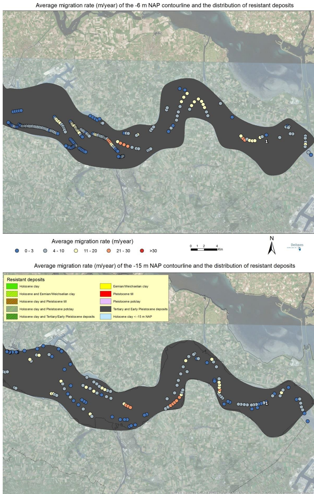
Figure 5.11 Average migration rates for the Westerschelde estuary and the distribution of resistant deposits.
