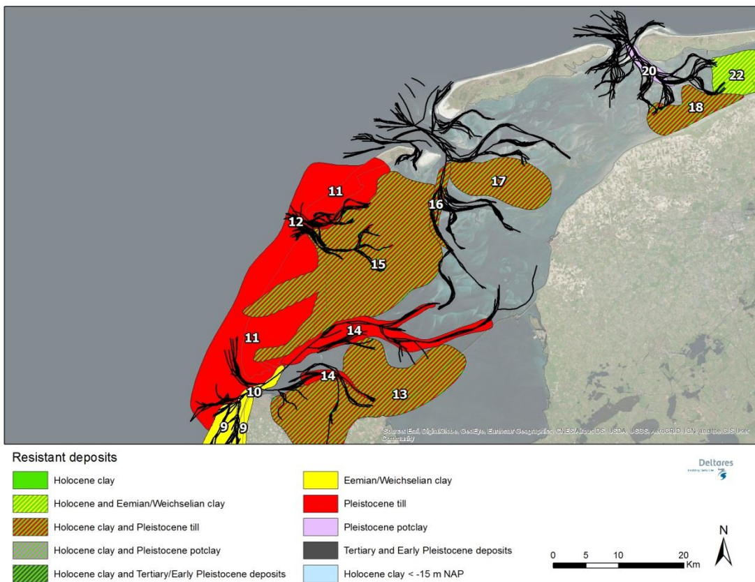
Figure 5.13 Mapped thalwegs over several decades in the western Wadden Sea (Cleveringa en Geleynse, 2017) plotted with the areas with erosion-resistant deposits (Hijma, 2017a).
