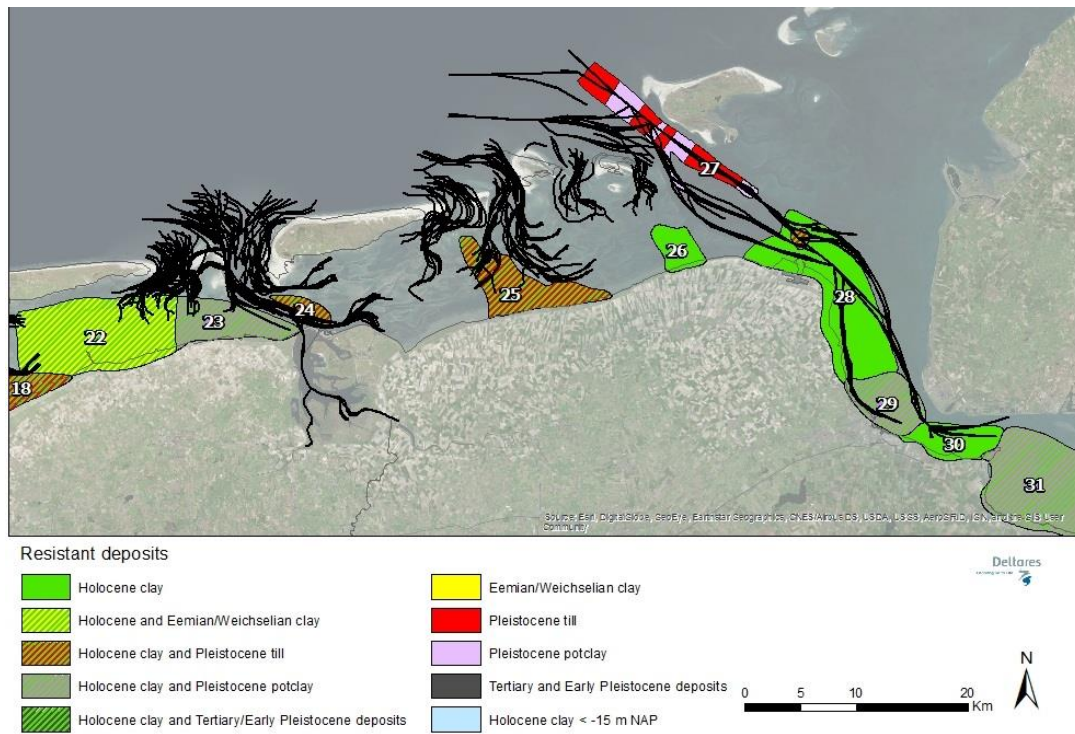
Figure 5.12 Mapped thalwegs over several decades in the eastern Wadden Sea (Cleveringa en Geleynse, 2017) plotted with the areas with erosion-resistant deposits (Hijma, 2017a).
