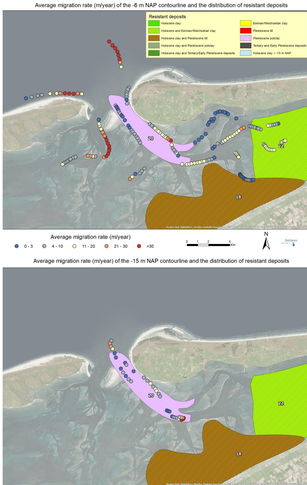
Figure 5.6 Average migration rates for the Borndiep inlet and the distribution of resistant deposits.
