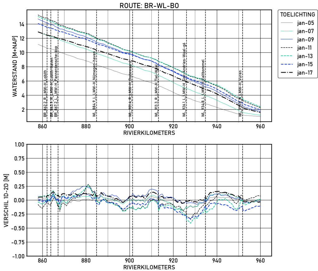
Figure 1.45 BR-WL-B0 | figures | Validatie | D_8000 | Langsprofiel
