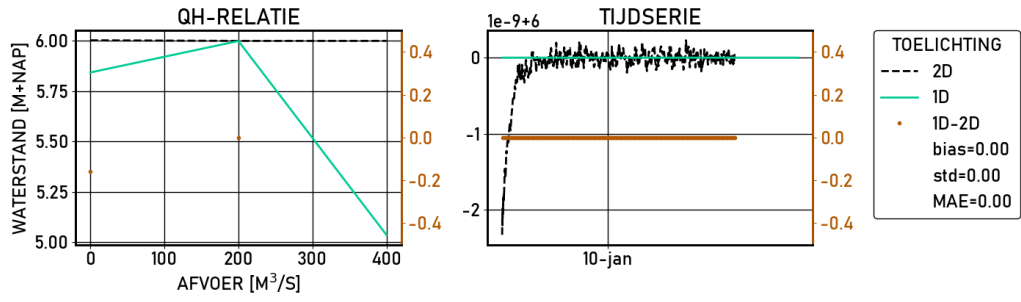
Figure 2.460 Amerongen-boven | figures | Validatie | S_2000 | stations
