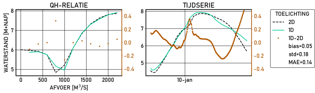
Figure 2.451 Amerongen-boven | figures | Validatie | D10000 | stations
