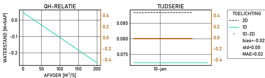
Figure 2.287 Kamperhoek-g6 | figures | Validatie | S_8000 | stations
