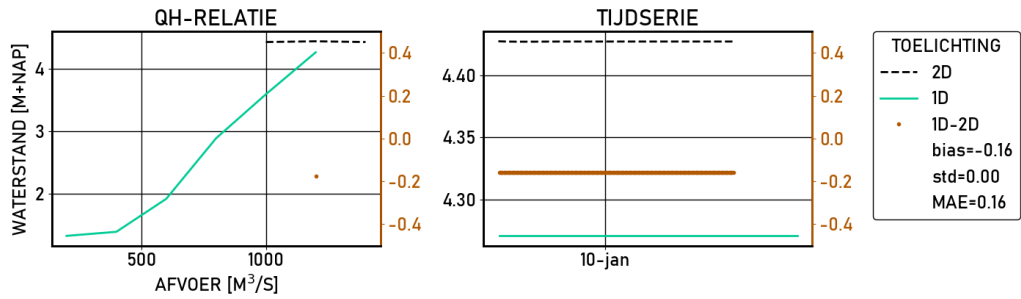
Figure 2.239 Wijhe | figures | Validatie | S_8000 | stations
