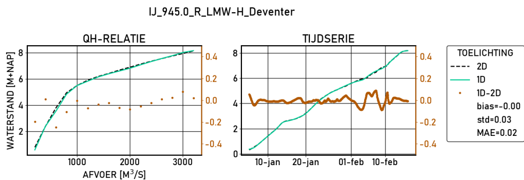
Figure 2.194 Deventer | figures | Kalibratie | stations
