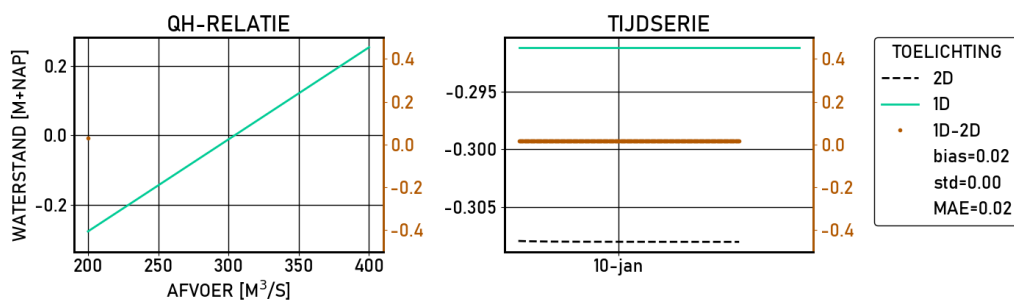
Figure 2.256 Katerveer | figures | Validatie | S__600 | stations
