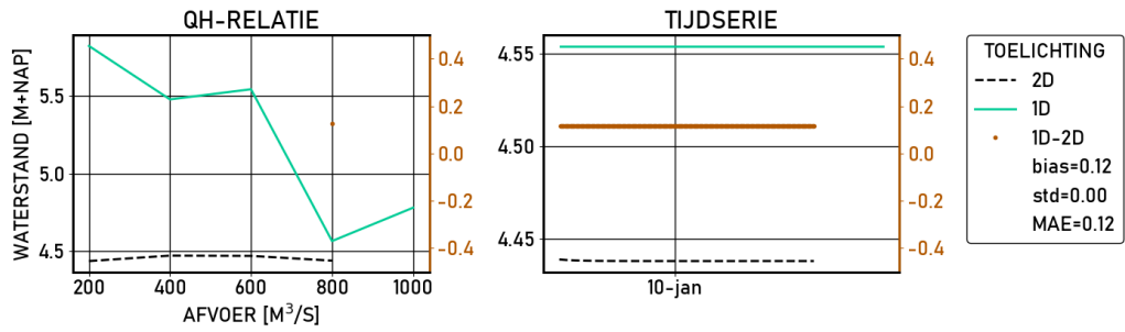
Figure 2.461 Amerongen-boven | figures | Validatie | S_4000 | stations
