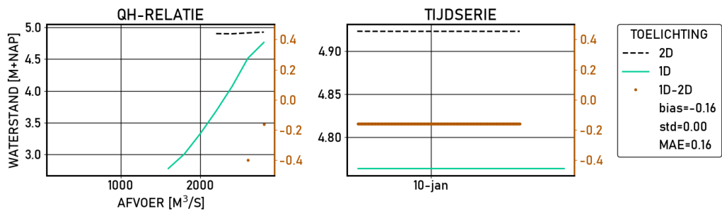
Figure 2.605 Sint-Andries-Waal-g6 | figures | Validatie | S_4000 | stations
