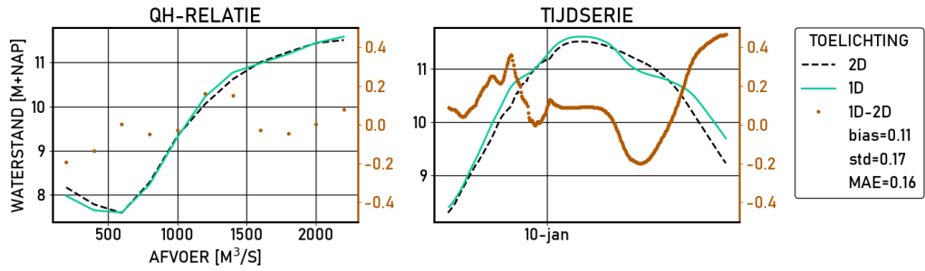
Figure 2.403 Driel-boven | figures | Validatie | D10000 | stations
