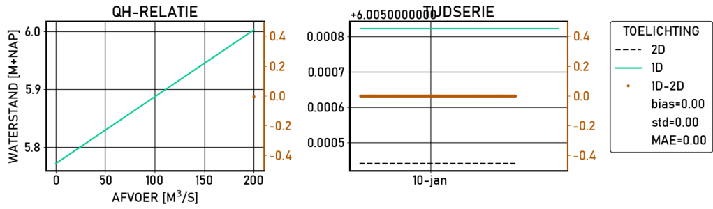
Figure 2.427 Driel-beneden | figures | Validatie | S_1020 | stations
