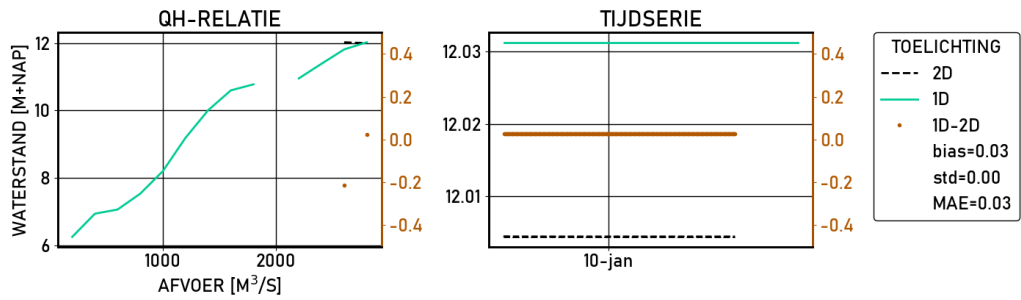
Figure 2.425 Driel-beneden | figures | Validatie | S13000 | stations
