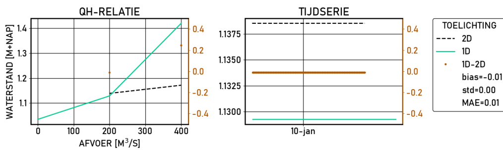
Figure 2.364 Hagestein-beneden | figures | Validatie | S_2000 | stations
