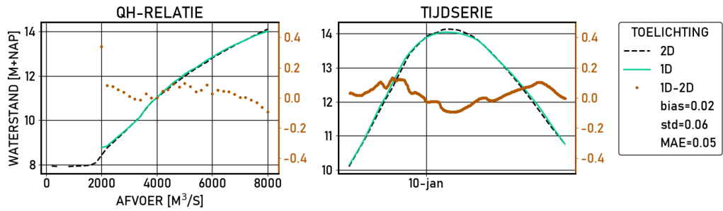
Figure 2.71 Pannerdensche-kop | figures | Validatie | D_8000 | stations
