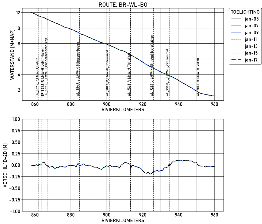
Figure 1.57 BR-WL-B0 | figures | Validatie | S_4000 | Langsprofiel
