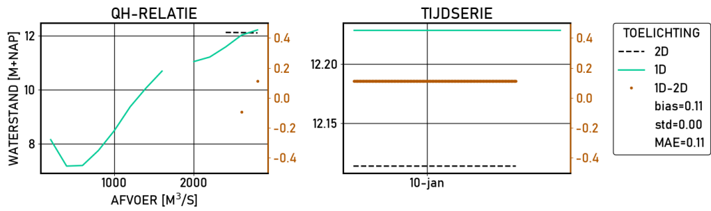
Figure 2.409 Driel-boven | figures | Validatie | S13000 | stations
