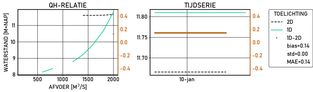
Figure 2.542 IJsselkop | figures | Validatie | S_6000 | stations
