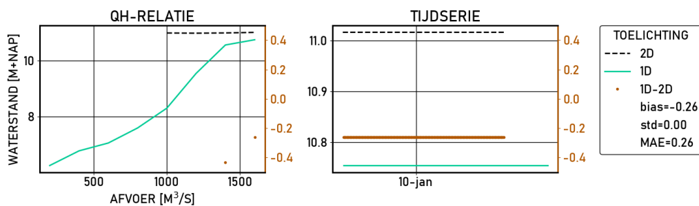
Figure 2.431 Driel-beneden | figures | Validatie | S_8000 | stations
