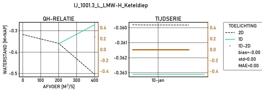
Figure 2.96 Keteldiep | figures | Validatie | S__600 | stations
