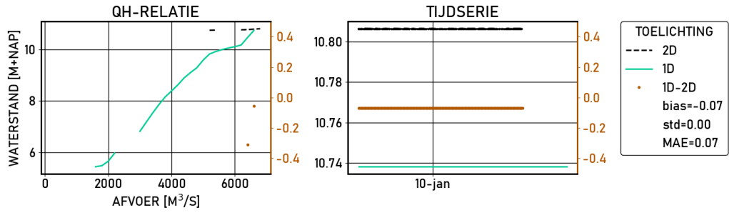
Figure 2.568 Dodewaard | figures | Validatie | S10000 | stations
