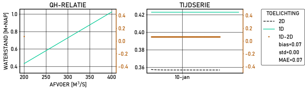
Figure 2.235 Wijhe | figures | Validatie | S_1020 | stations
