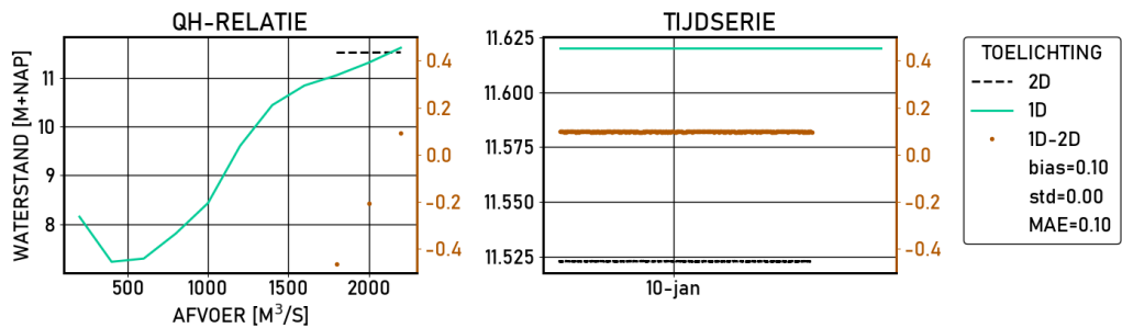
Figure 2.408 Driel-boven | figures | Validatie | S10000 | stations
