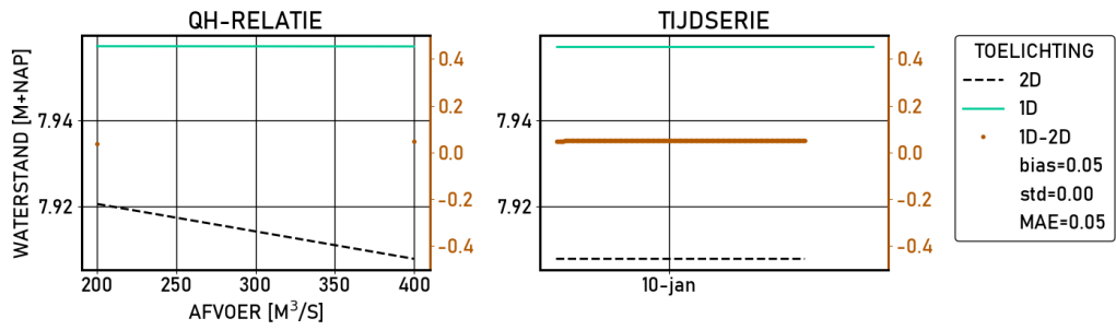
Figure 2.124 Westervoort-IJsseldijke | figures | Validatie | S_2000 | stations
