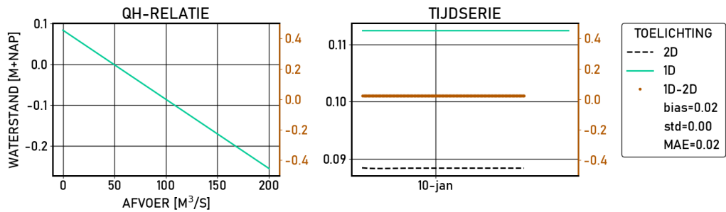
Figure 2.303 Ketelhaven | figures | Validatie | S_8000 | stations
