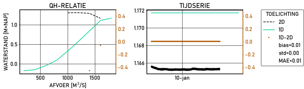
Figure 2.264 Kampen-bovenhaven | figures | Validatie | S10000 | stations
