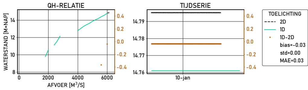
Figure 2.538 IJsselkop | figures | Validatie | S16000 | stations
