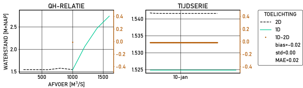
Figure 2.603 Sint-Andries-Waal-g6 | figures | Validatie | S_1020 | stations
