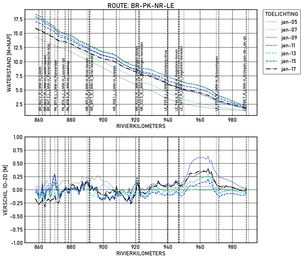
Figure 1.73 BR-PK-NR-LE | figures | Validatie | D16000 | Langsprofiel
