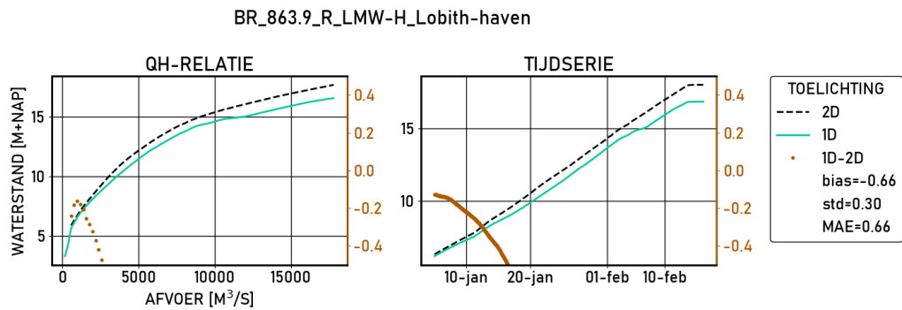
Figure 2.49 Lobith-haven | figures | Ongekalibreerd | stations
