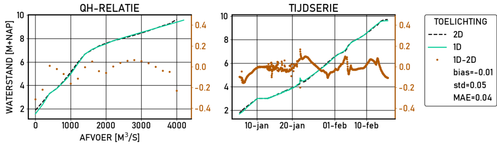
Figure 2.466 Amerongen-beneden | figures | Kalibratie | stations
