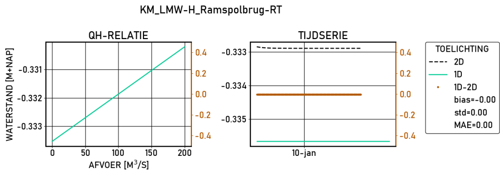
Figure 2.315 Ramspolbrug-RT | figures | Validatie | S_1020 | stations
