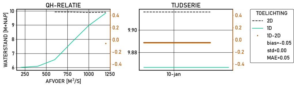
Figure 2.159 Doesburg-brug | figures | Validatie | S_8000 | stations
