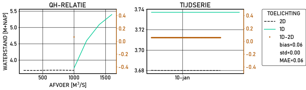
Figure 2.571 Dodewaard | figures | Validatie | S_1020 | stations
