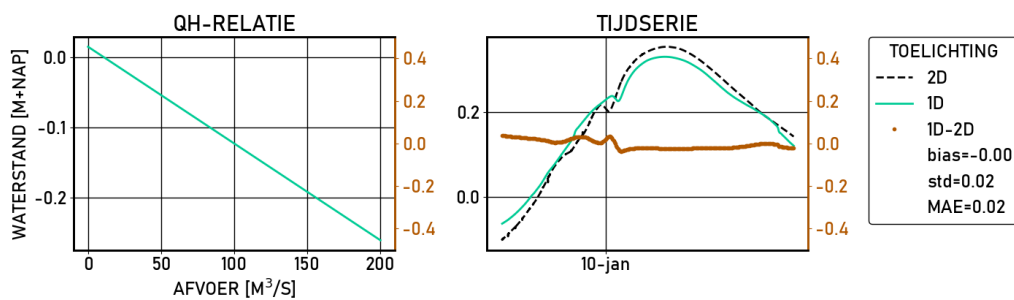
Figure 2.277 Kamperhoek-g6 | figures | Validatie | D16000 | stations
