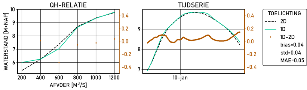
Figure 2.151 Doesburg-brug | figures | Validatie | D_8000 | stations
