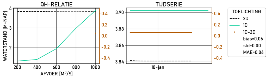
Figure 2.238 Wijhe | figures | Validatie | S_6000 | stations
