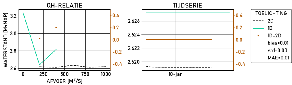
Figure 2.587 Tiel-Waal | figures | Validatie | S_1020 | stations
