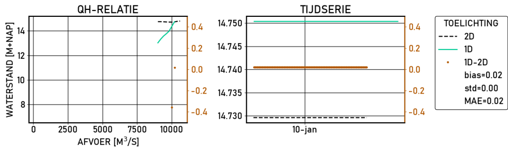
Figure 2.554 Nijmegen-haven | figures | Validatie | S16000 | stations
