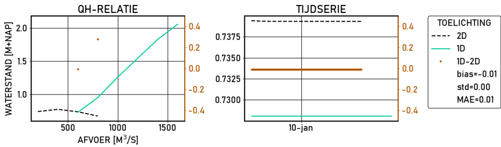
Figure 2.624 Zaltbommel | figures | Validatie | S_600 | stations
