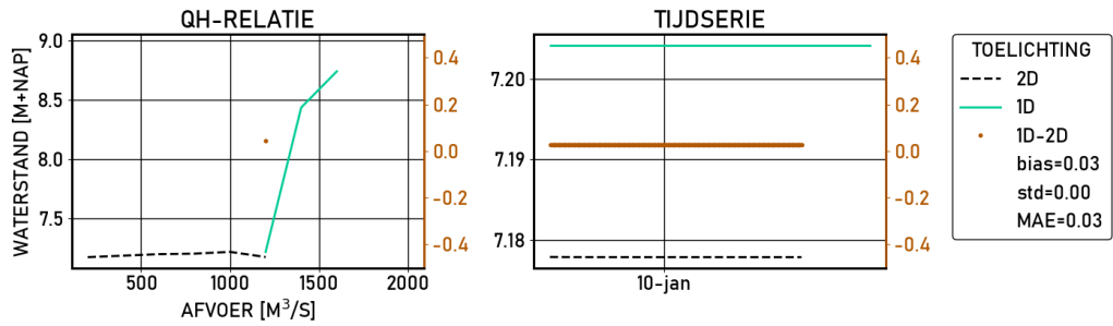
Figure 2.59 Lobith-haven | figures | Validatie | S_1020 | stations
