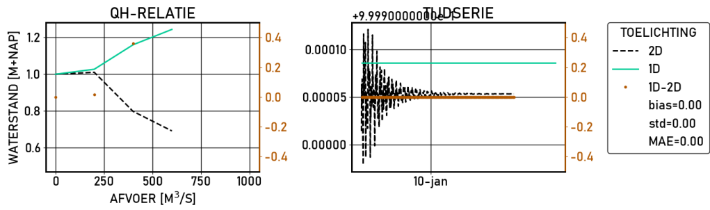
Figure 2.379 Schoonhoven | figures | Validatie | S_1020 | stations
