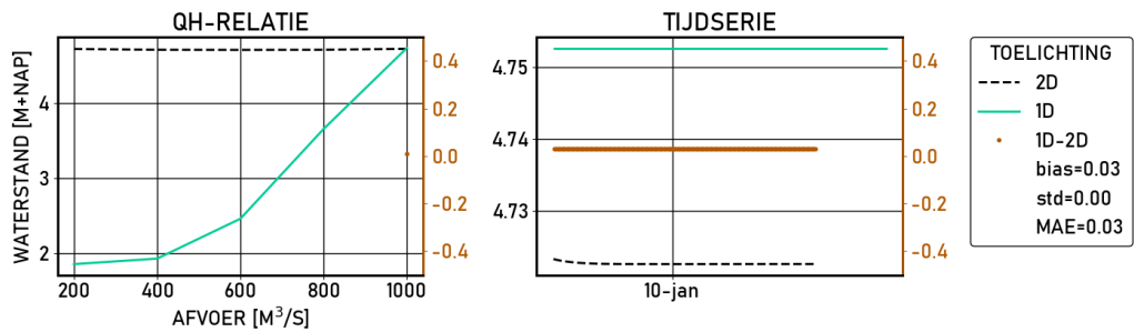
Figure 2.222 Olst | figures | Validatie | S_6000 | stations
