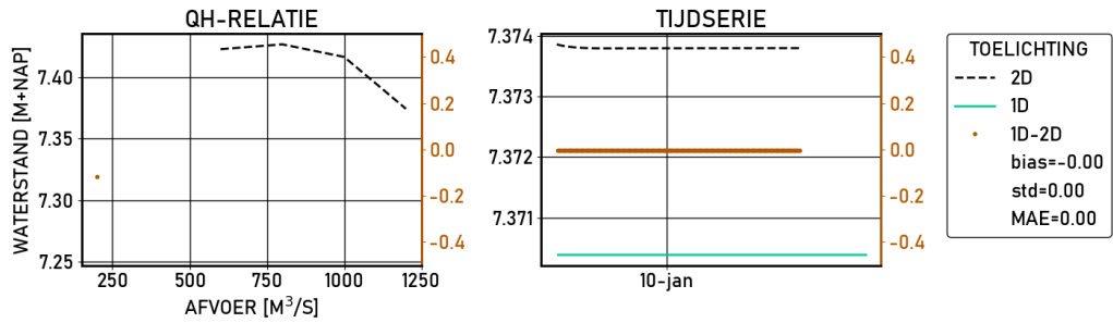
Figure 2.191 Eefde-beneden | figures | Validatie | S_8000 | stations
