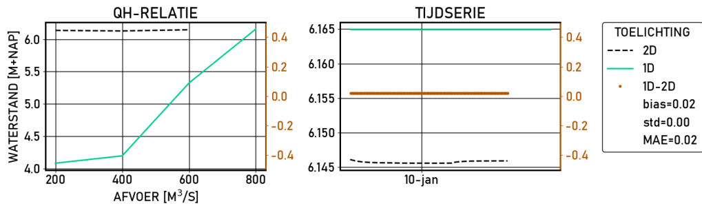
Figure 2.173 Zutphen-noord | figures | Validatie | S_4000 | stations
