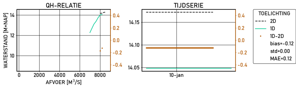
Figure 2.79 Pannerdensche-kop | figures | Validatie | S_8000 | stations
