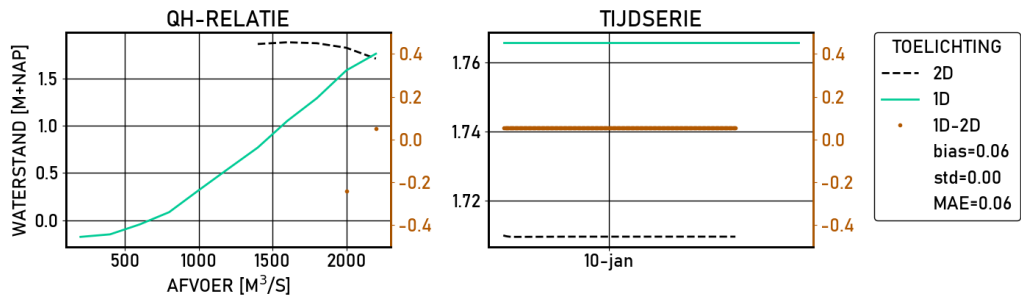
Figure 2.265 Kampen-bovenhaven | figures | Validatie | S13000 | stations
