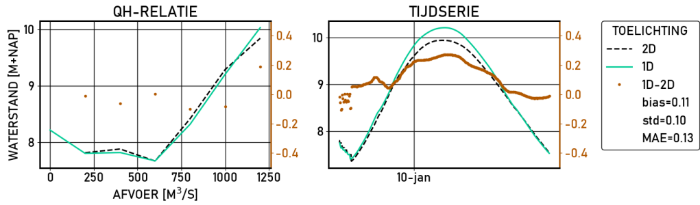
Figure 2.406 Driel-boven | figures | Validatie | D_6000 | stations
