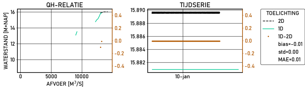
Figure 2.73 Pannerdensche-kop | figures | Validatie | S13000 | stations
