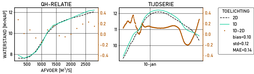
Figure 2.404 Driel-boven | figures | Validatie | D13000 | stations
