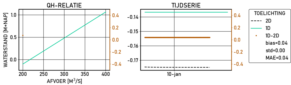
Figure 2.240 Wijhe | figures | Validatie | S__600 | stations
