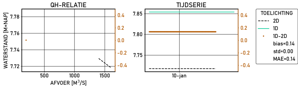
Figure 2.184 Eefde-beneden | figures | Validatie | S10000 | stations
