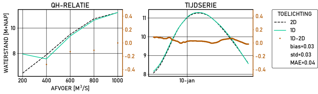
Figure 2.118 Westervoort-IJsseldijke | figures | Validatie | D_6000 | stations
