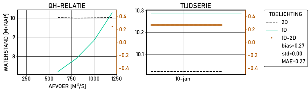
Figure 2.414 Driel-boven | figures | Validatie | S_6000 | stations
