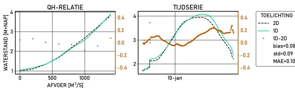
Figure 2.359 Hagestein-beneden | figures | Validatie | D_8000 | stations
