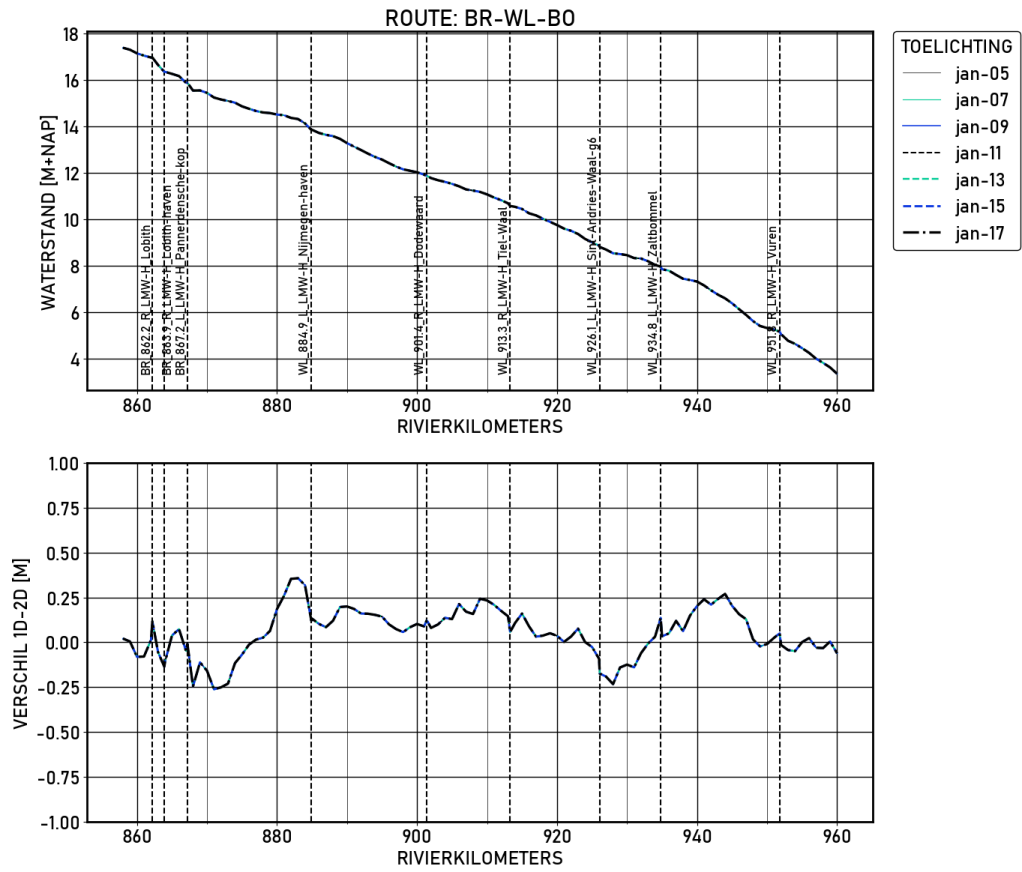
Figure 1.49 BR-WL-BO | figures | Validatie | S13000 | Langsprofiel
