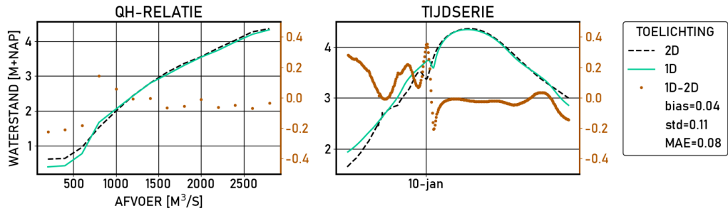
Figure 2.245 Katerveer | figures | Validatie | D16000 | stations
