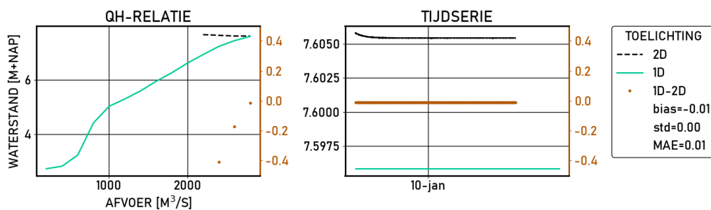
Figure 2.202 Deventer | figures | Validatie | S16000 | stations
