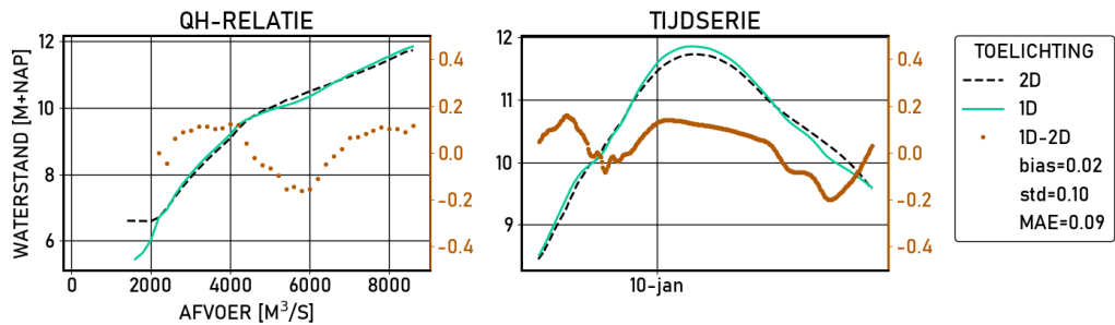
Figure 2.564 Dodewaard | figures | Validatie | D13000 | stations
