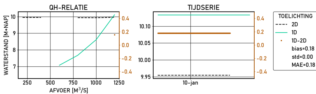
Figure 2.430 Driel-beneden | figures | Validatie | S_6000 | stations
