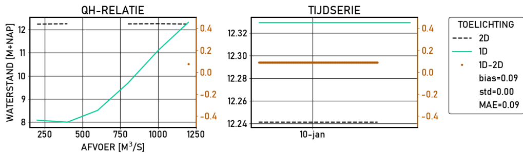
Figure 2.111 Hondsbroeksche-Pleij-IJ | figures | Validatie | S_8000 | stations
