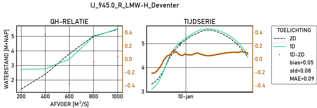
Figure 2.198 Deventer | figures | Validatie | D_6000 | stations
