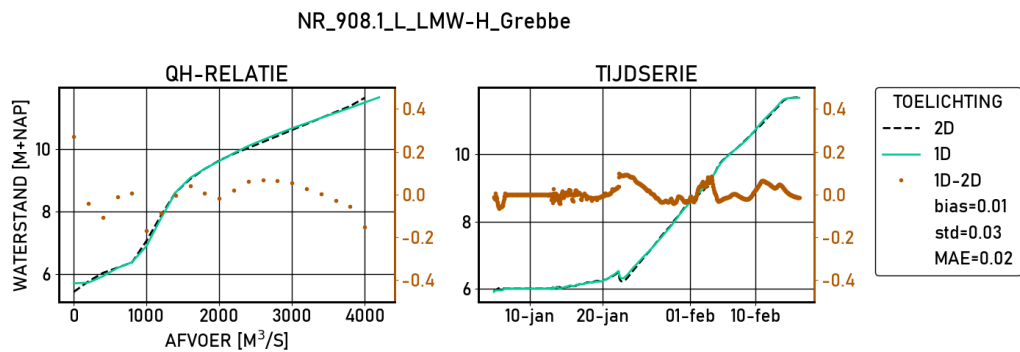
Figure 2.434 Grebbe | figures | Kalibratie | stations
