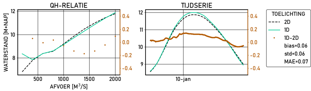
Figure 2.518 Looweer-g6 | figures | Validatie | D_6000 | stations
