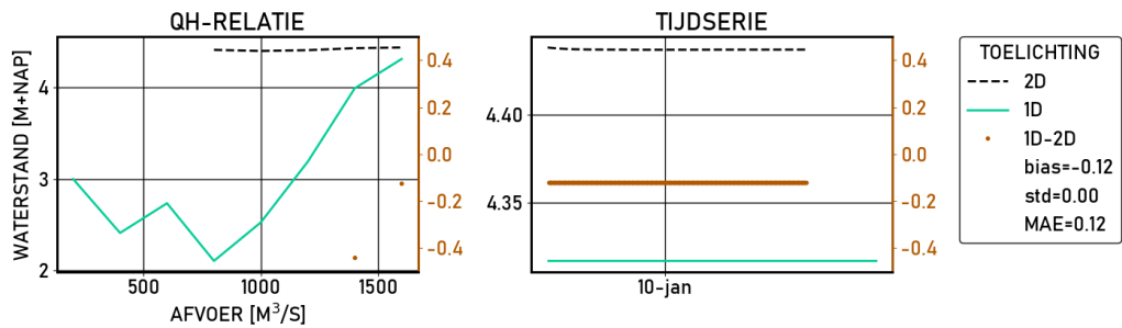
Figure 2.351 Hagestein-boven | figures | Validatie | S_8000 | stations
