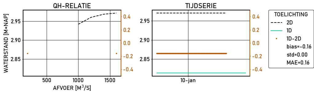
Figure 2.604 Sint-Andries-Waal-g6 | figures | Validatie | S_2000 | stations
