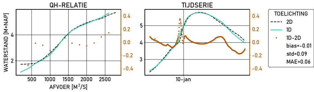
Figure 2.356 Hagestein-beneden | figures | Validatie | D13000 | stations
