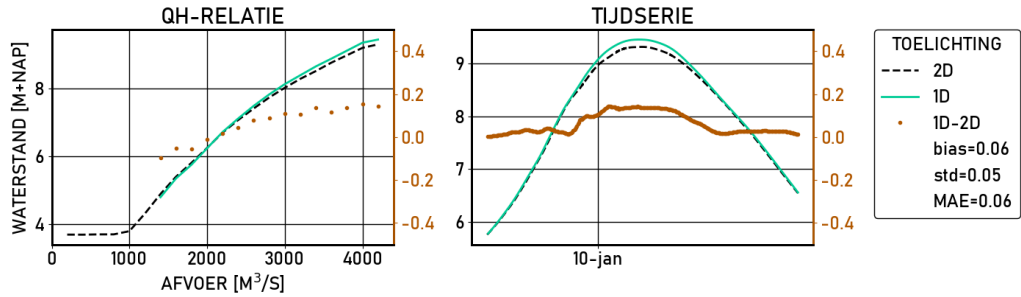
Figure 2.566 Dodewaard | figures | Validatie | D_6000 | stations
