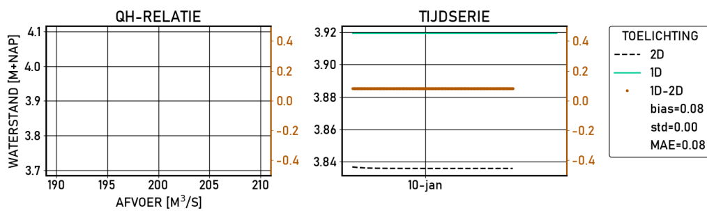
Figure 2.13 Tiel-Kanaal | figures | Validatie | S_4000 | stations
