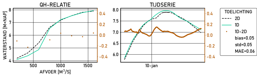
Figure 2.163 Zutphen-noord | figures | Validatie | D10000 | stations
