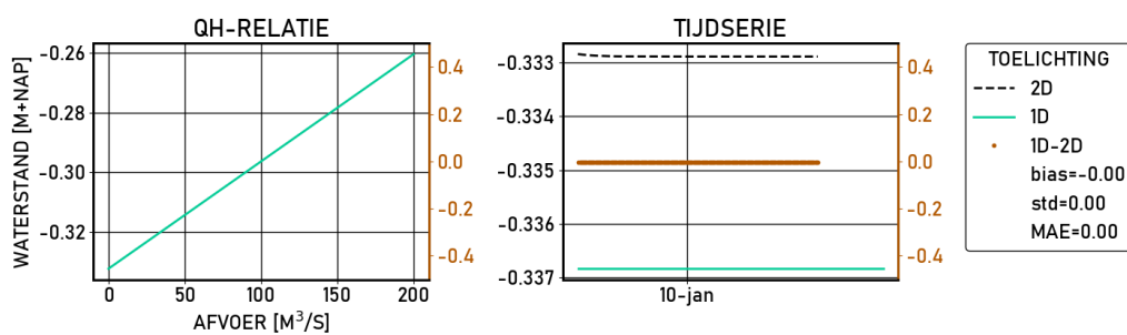
Figure 2.283 Kamperhoek-g6 | figures | Validatie | S_1020 | stations
