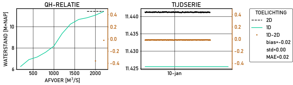
Figure 2.424 Driel-beneden | figures | Validatie | S10000 | stations
