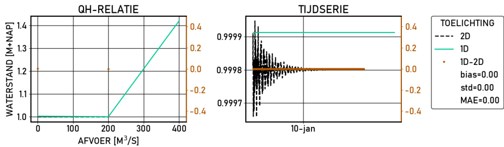
Figure 2.363 Hagestein-beneden | figures | Validatie | S_1020 | stations
