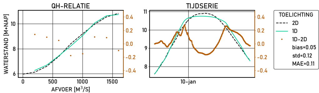
Figure 2.423 Driel-beneden | figures | Validatie | D_8000 | stations
