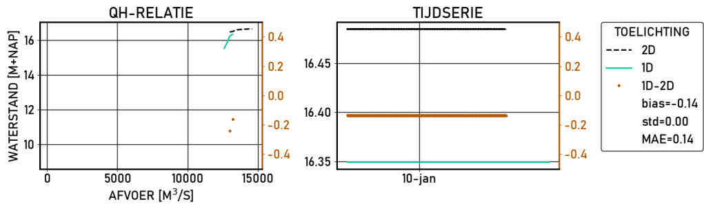
Figure 2.57 Lobith-haven | figures | Validatie | S13000 | stations
