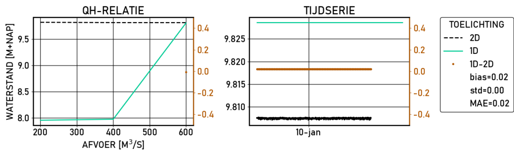
Figure 2.125 Westervoort-IJsseldijke | figures | Validatie | S_4000 | stations
