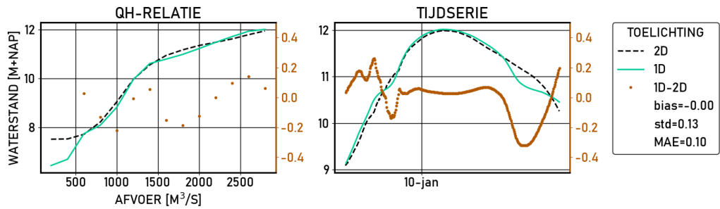
Figure 2.420 Driel-beneden | figures | Validatie | D13000 | stations
