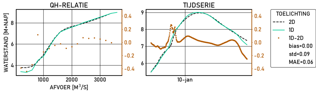
Figure 2.469 Amerongen-beneden | figures | Validatie | D16000 | stations
