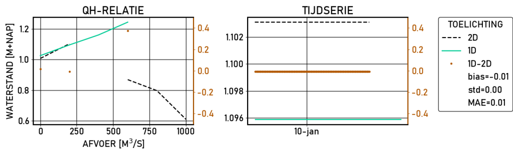
Figure 2.380 Schoonhoven | figures | Validatie | S_2000 | stations
