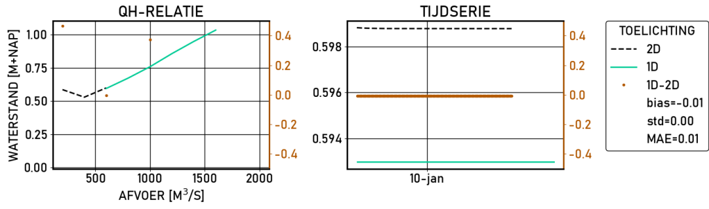
Figure 2.640 Vuren | figures | Validatie | S__600 | stations
