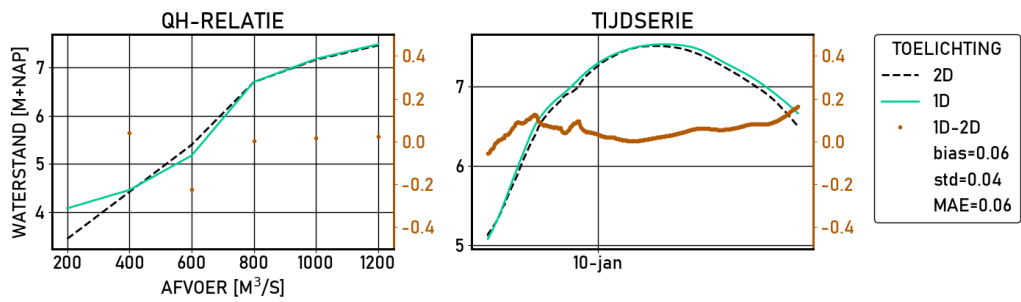
Figure 2.167 Zutphen-noord | figures | Validatie | D_8000 | stations
