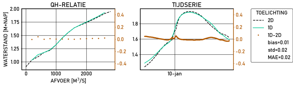
Figure 2.388 Krimpen-aan-de-Lek-g6 | figures | Validatie | D13000 | stations
