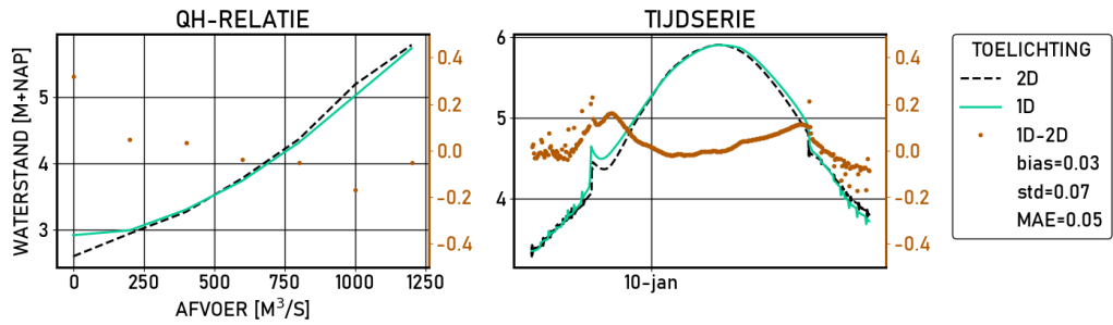
Figure 2.470 Amerongen-beneden | figures | Validatie | D_6000 | stations
