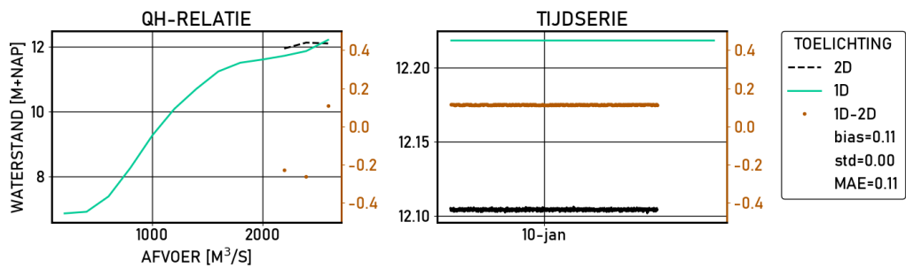
Figure 2.138 De-Steeg | figures | Validatie | S16000 | stations
