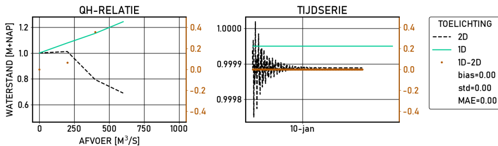
Figure 2.384 Schoonhoven | figures | Validatie | S_600 | stations
