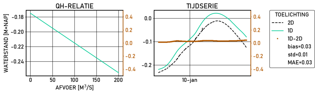
Figure 2.294 Ketelhaven | figures | Validatie | D_6000 | stations
