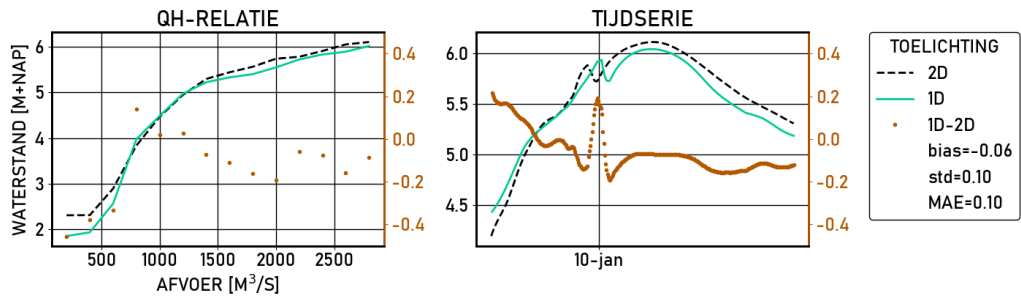
Figure 2.213 Olst | figures | Validatie | D16000 | stations
