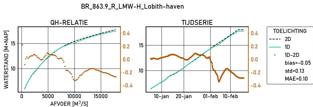
Figure 2.50 Lobith-haven | figures | Kalibratie | stations
