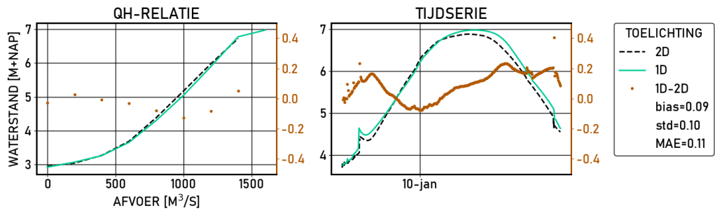
Figure 2.471 Amerongen-beneden | figures | Validatie | D_8000 | stations
