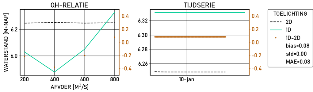
Figure 2.445 Grebbe | figures | Validatie | S_4000 | stations
