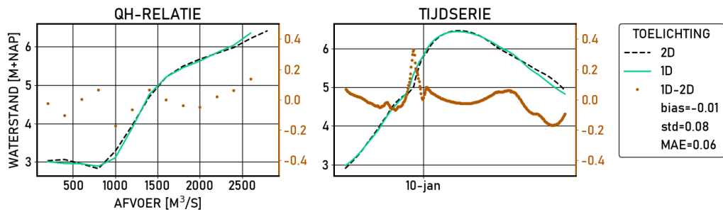
Figure 2.324 Culemborg-brug | figures | Validatie | D13000 | stations
