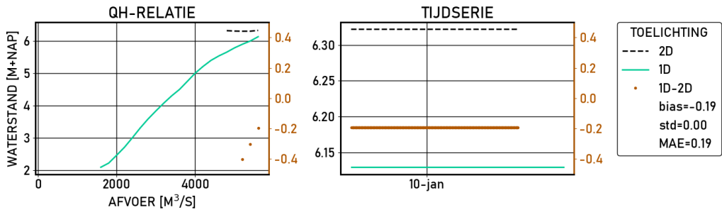
Figure 2.623 Zaltbommel | figures | Validatie | S_8000 | stations
