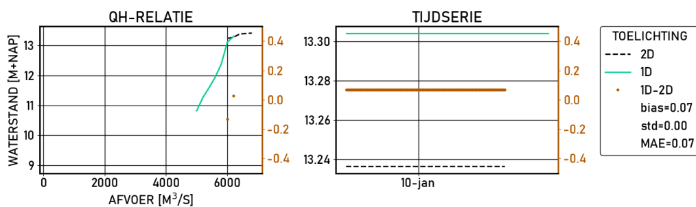
Figure 2.62 Lobith-haven | figures | Validatie | S_6000 | stations
