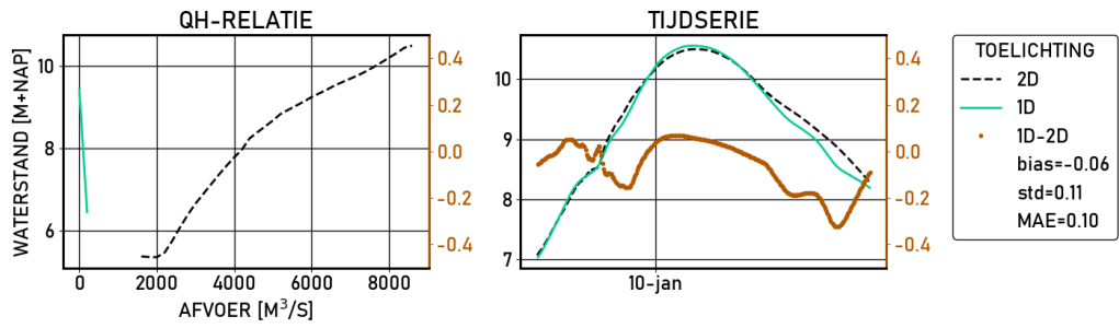
Figure 2.580 Tiel-Waal | figures | Validatie | D13000 | stations
