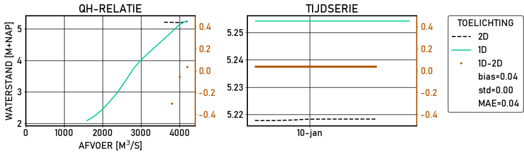
Figure 2.622 Zaltbommel | figures | Validatie | S_6000 | stations
