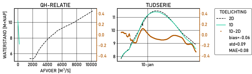
Figure 2.581 Tiel-Waal | figures | Validatie | D16000 | stations
