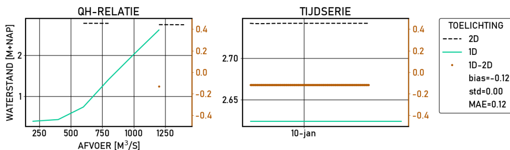
Figure 2.255 Katerveer | figures | Validatie | S_8000 | stations
