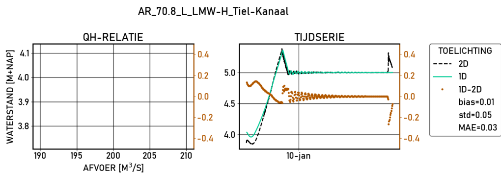
Figure 2.3 Tiel-Kanaal | figures | Validatie | D10000 | stations
