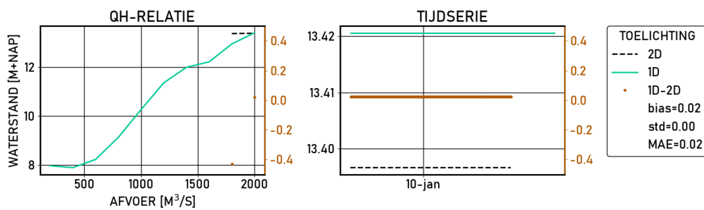
Figure 2.121 Westervoort-IJsseldijke | figures | Validatie | S13000 | stations
