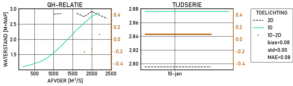
Figure 2.376 Schoonhoven | figures | Validatie | S10000 | stations
