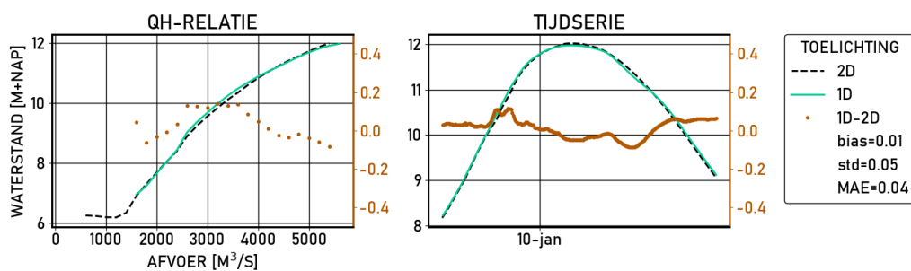
Figure 2.551 Nijmegen-haven | figures | Validatie | D_8000 | stations
