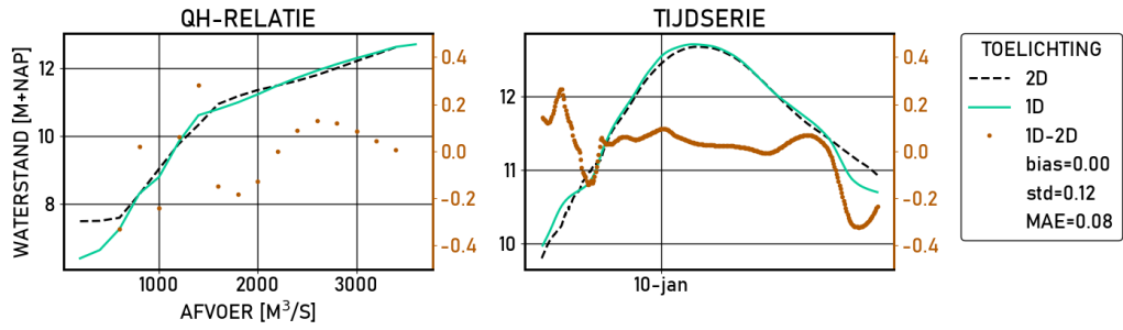
Figure 2.421 Driel-beneden | figures | Validatie | D16000 | stations
