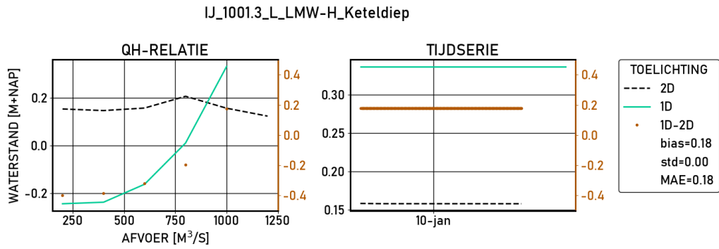
Figure 2.94 Keteldiep | figures | Validatie | S_6000 | stations
