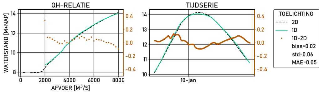
Figure 2.493 Pannerden | figures | Validatie | D_8000 | stations
