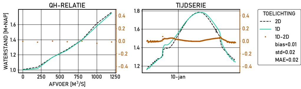
Figure 2.374 Schoonhoven | figures | Validatie | D_6000 | stations
