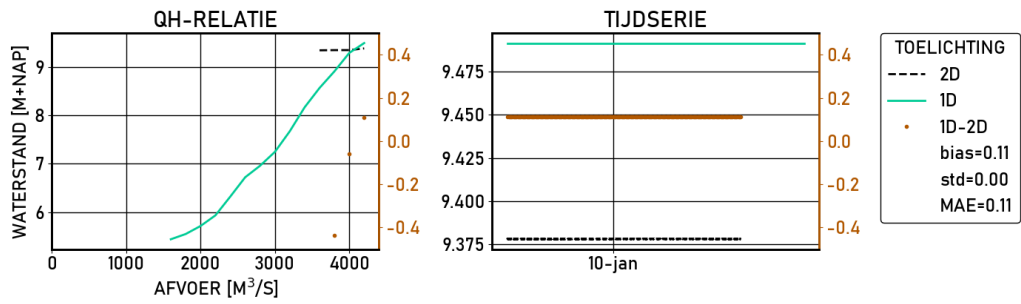
Figure 2.574 Dodewaard | figures | Validatie | S_6000 | stations
