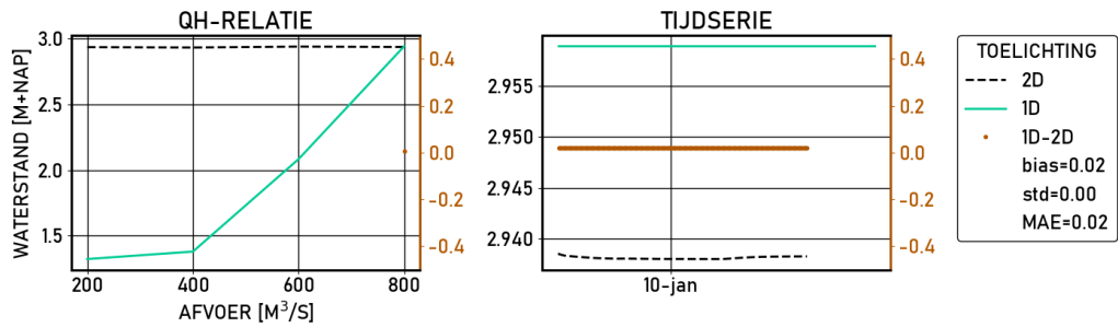
Figure 2.237 Wijhe | figures | Validatie | S_4000 | stations
