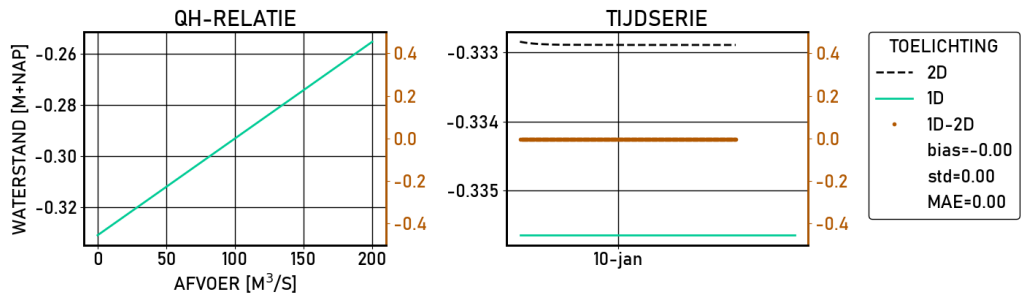
Figure 2.299 Ketelhaven | figures | Validatie | S_1020 | stations
