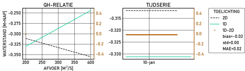
Figure 2.267 Kampen-bovenhaven | figures | Validatie | S_1020 | stations
