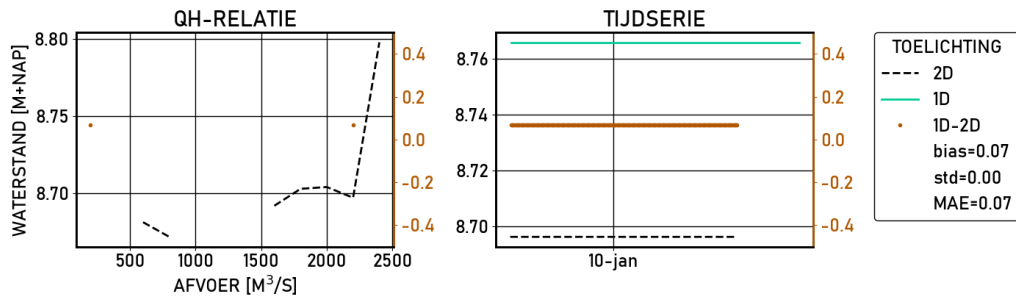
Figure 2.76 Pannerdensche-kop | figures | Validatie | S_2000 | stations
