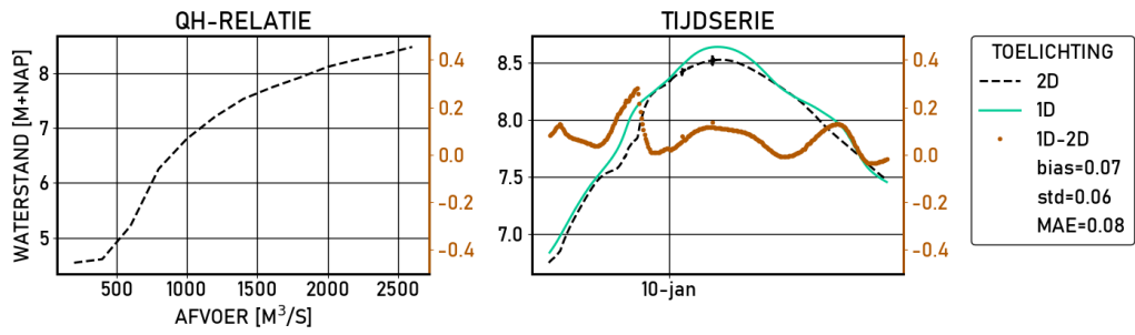
Figure 2.181 Eefde-beneden | figures | Validatie | D16000 | stations
