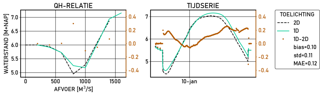
Figure 2.455 Amerongen-boven | figures | Validatie | D_8000 | stations
