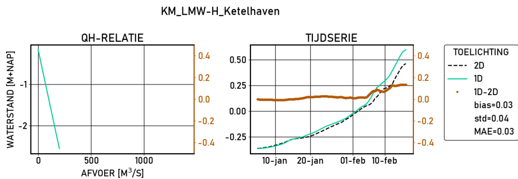
Figure 2.290 Ketelhaven | figures | Kalibratie | stations
