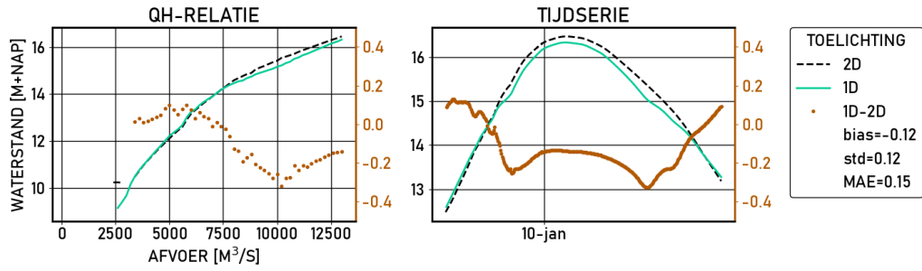
Figure 2.52 Lobith-haven | figures | Validatie | D13000 | stations
