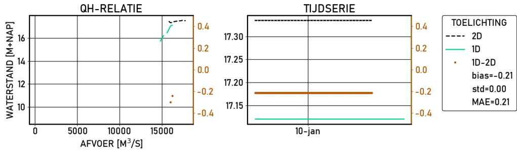
Figure 2.58 Lobith-haven | figures | Validatie | S16000 | stations
