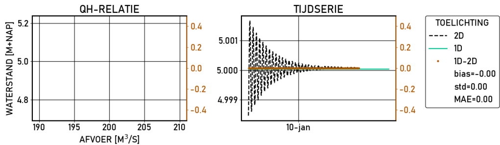
Figure 2.9 Tiel-Kanaal | figures | Validatie | S13000 | stations
