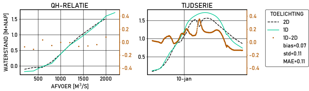
Figure 2.260 Kampen-bovenhaven | figures | Validatie | D13000 | stations
