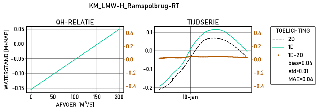
Figure 2.311 Ramspolbrug-RT | figures | Validatie | D_8000 | stations
