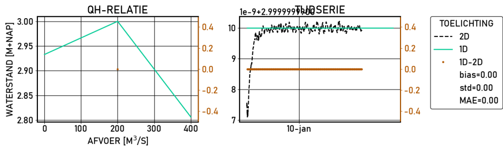
Figure 2.348 Hagestein-boven | figures | Validatie | S_2000 | stations
