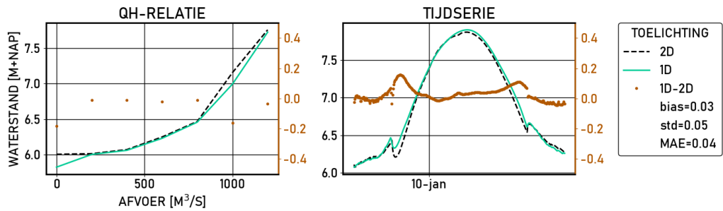
Figure 2.438 Grebbe | figures | Validatie | D_6000 | stations
