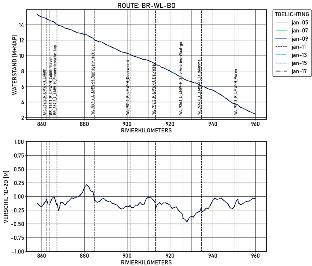
Figure 1.61 BR-WL-B0 | figures | Validatie | S_8000 | Langsprofiel
