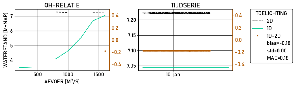
Figure 2.479 Amerongen-beneden | figures | Validatie | S_8000 | stations
