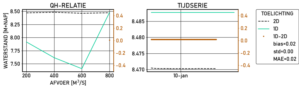
Figure 2.413 Driel-boven | figures | Validatie | S_4000 | stations
