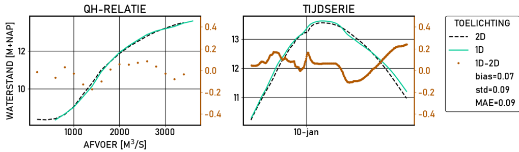
Figure 2.515 Looweer-g6 | figures | Validatie | D10000 | stations
