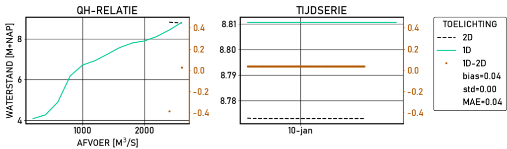
Figure 2.170 Zutphen-noord | figures | Validatie | S16000 | stations
