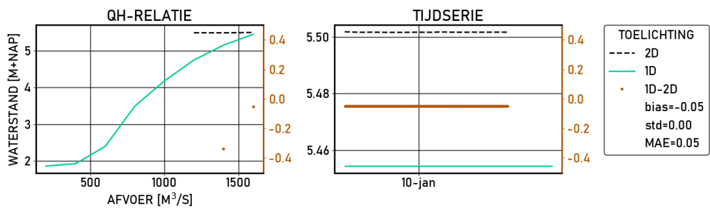
Figure 2.216 Olst | figures | Validatie | S10000 | stations
