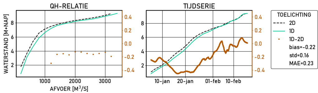
Figure 2.161 Zutphen-noord | figures | Ongekalibreerd | stations
