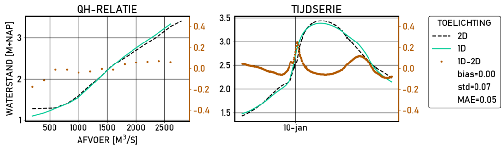
Figure 2.372 Schoonhoven | figures | Validatie | D13000 | stations
