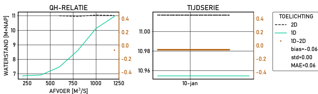
Figure 2.143 De-Steeg | figures | Validatie | S_8000 | stations
