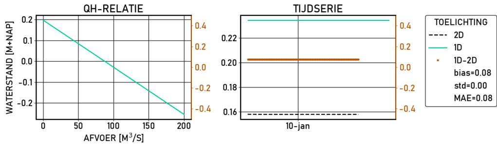
Figure 2.296 Ketelhaven | figures | Validatie | S10000 | stations
