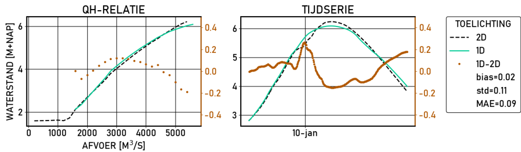
Figure 2.615 Zaltbommel | figures | Validatie | D_8000 | stations
