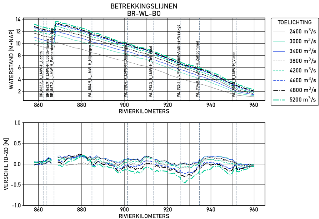
Figure 1.46 BR-WL-B0 | figures | Validatie | D_8000 | Langsprofiel
