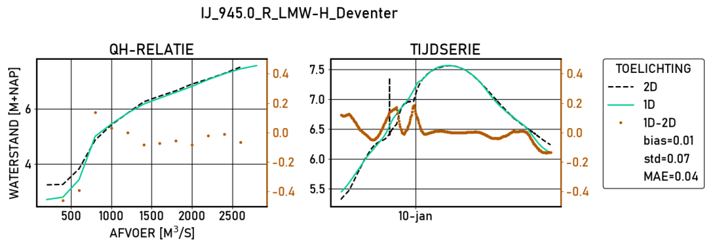
Figure 2.197 Deventer | figures | Validatie | D16000 | stations
