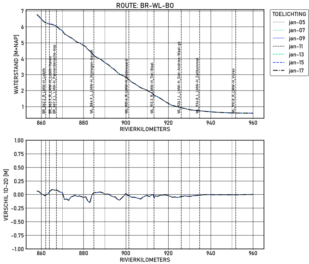
Figure 1.63 BR-WL-B0 | figures | Validatie | S_600 | Langsprofiel
