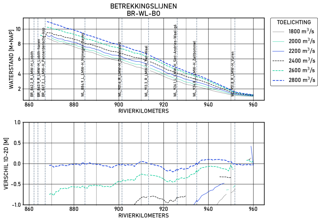
Figure 1.58 BR-WL-B0 | figures | Validatie | S_4000 | Langsprofiel
