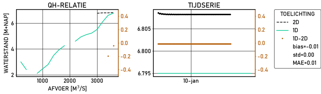
Figure 2.346 Hagestein-boven | figures | Validatie | S16000 | stations
