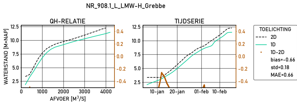
Figure 2.433 Grebbe | figures | Ongekalibreerd | stations
