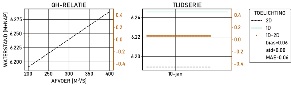
Figure 2.428 Driel-beneden | figures | Validatie | S_2000 | stations
