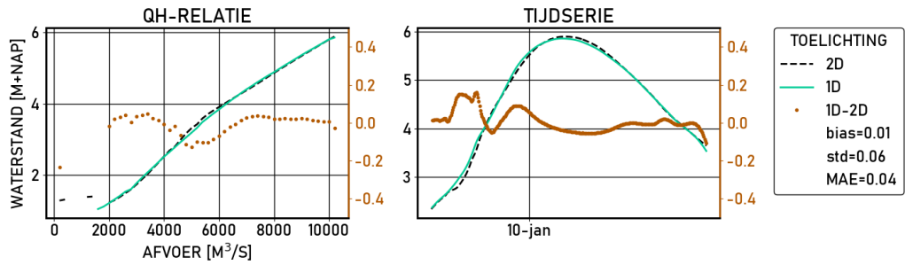
Figure 2.629 Vuren | figures | Validatie | D16000 | stations
