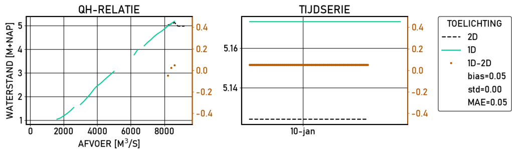
Figure 2.633 Vuren | figures | Validatie | S13000 | stations
