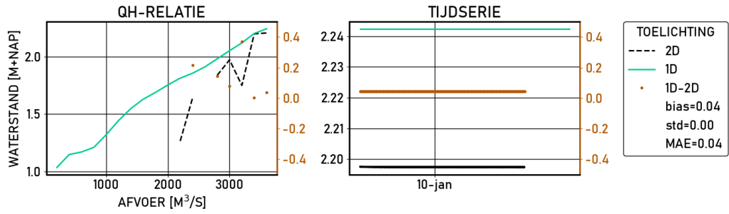
Figure 2.394 Krimpen-aan-de-Lek-g6 | figures | Validatie | S16000 | stations
