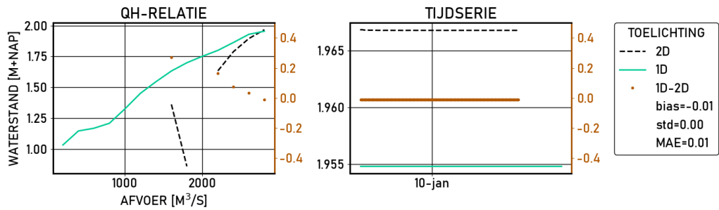
Figure 2.393 Krimpen-aan-de-Lek-g6 | figures | Validatie | S13000 | stations
