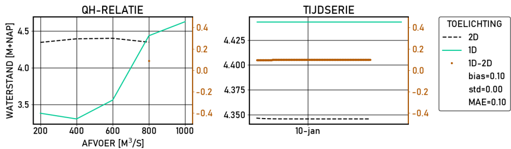
Figure 2.477 Amerongen-beneden | figures | Validatie | S_4000 | stations
