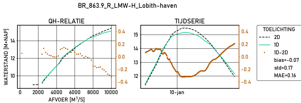
Figure 2.51 Lobith-haven | figures | Validatie | D10000 | stations
