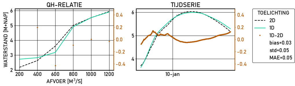
Figure 2.199 Deventer | figures | Validatie | D_8000 | stations
