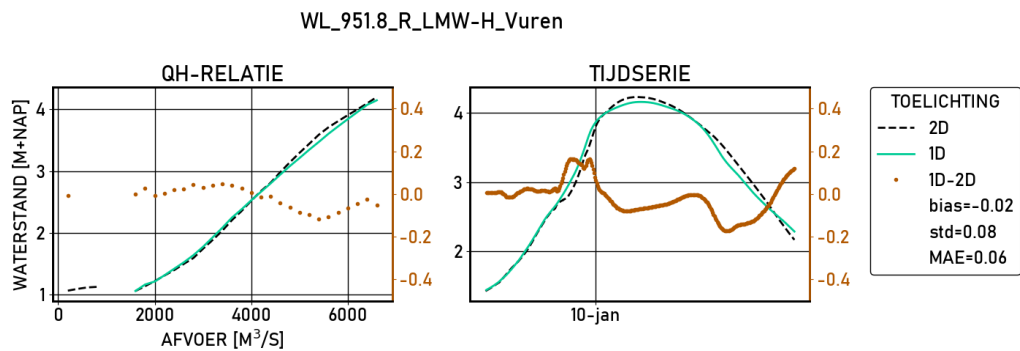
Figure 2.627 Vuren | figures | Validatie | D10000 | stations
