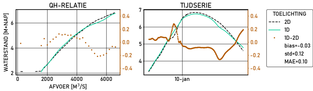
Figure 2.611 Zaltbommel | figures | Validatie | D10000 | stations
