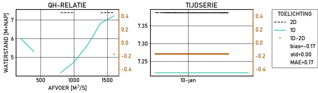
Figure 2.463 Amerongen-boven | figures | Validatie | S_8000 | stations
