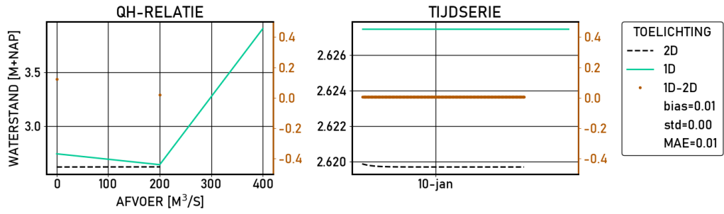
Figure 2.475 Amerongen-beneden | figures | Validatie | S_1020 | stations
