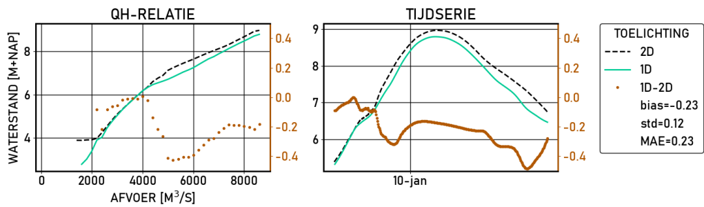
Figure 2.596 Sint-Andries-Waal-g6 | figures | Validatie | D13000 | stations
