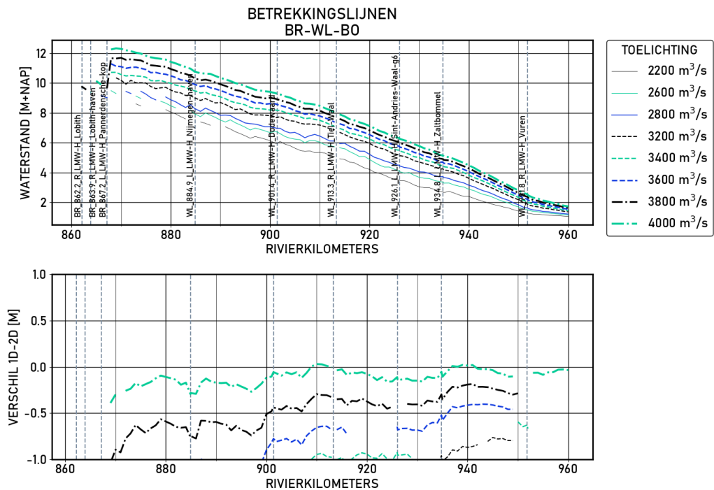
Figure 1.60 BR-WL-B0 | figures | Validatie | S_6000 | Langsprofiel
