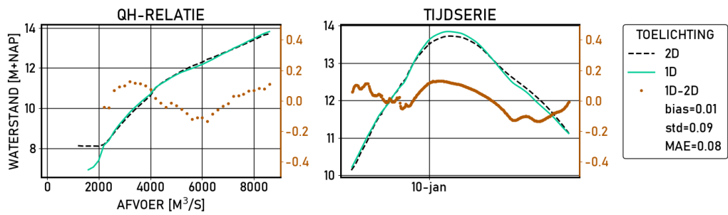
Figure 2.548 Nijmegen-haven | figures | Validatie | D13000 | stations
