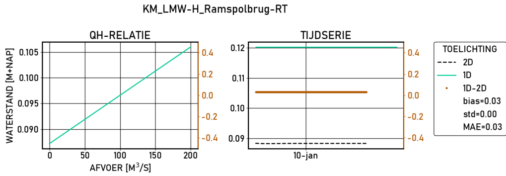
Figure 2.319 Ramspolbrug-RT | figures | Validatie | S_8000 | stations
