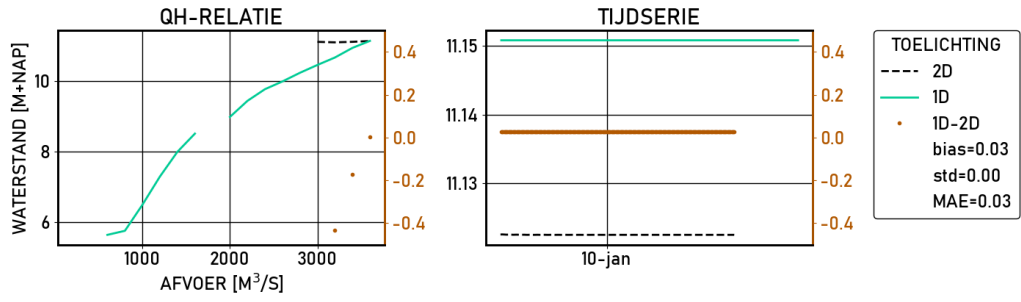
Figure 2.442 Grebbe | figures | Validatie | S16000 | stations
