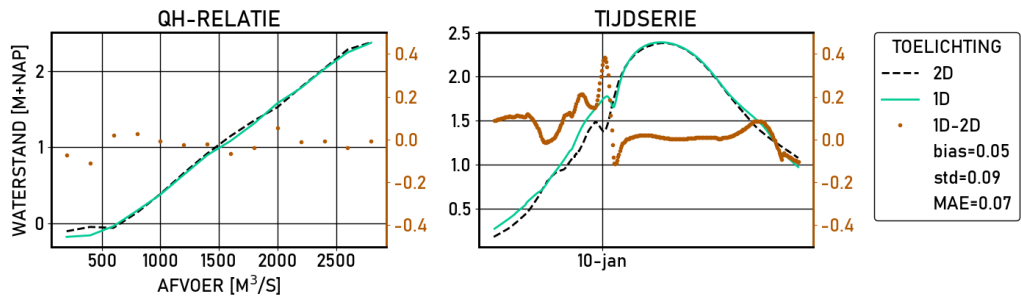
Figure 2.261 Kampen-bovenhaven | figures | Validatie | D16000 | stations
