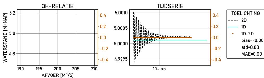
Figure 2.15 Tiel-Kanaal | figures | Validatie | S_8000 | stations
