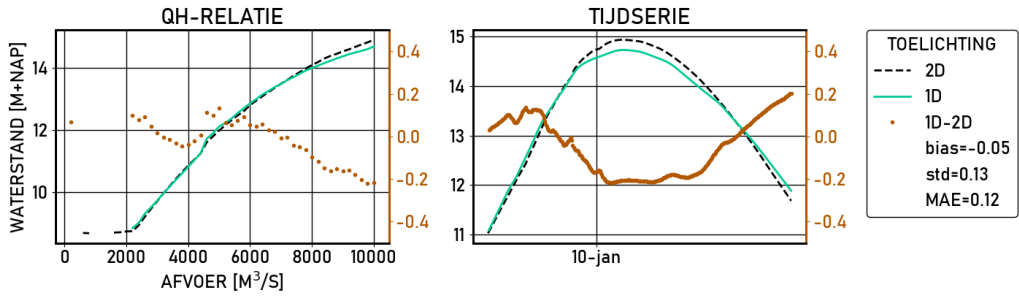
Figure 2.67 Pannerdensche-kop | figures | Validatie | D10000 | stations
