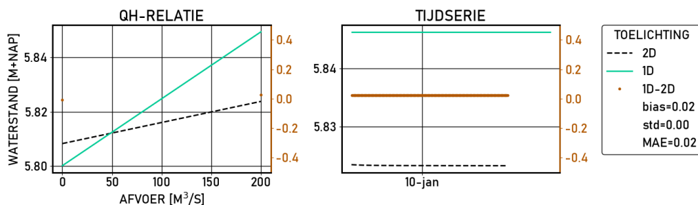
Figure 2.432 Driel-beneden | figures | Validatie | S__600 | stations
