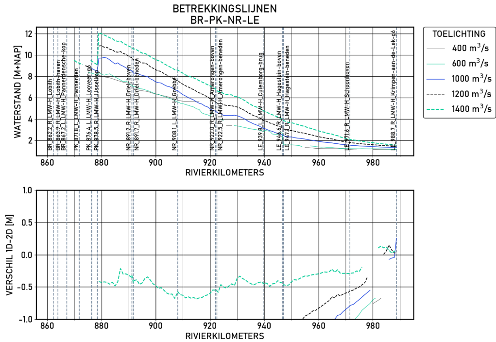
Figure 1.94 BR-PK-NR-LE | figures | Validatie | S_8000 | Langsprofiel
