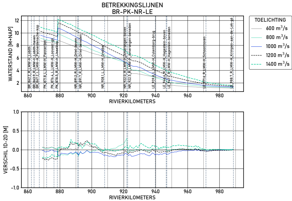
Figure 1.78 BR-PK-NR-LE | figures | Validatie | D_8000 | Langsprofiel
