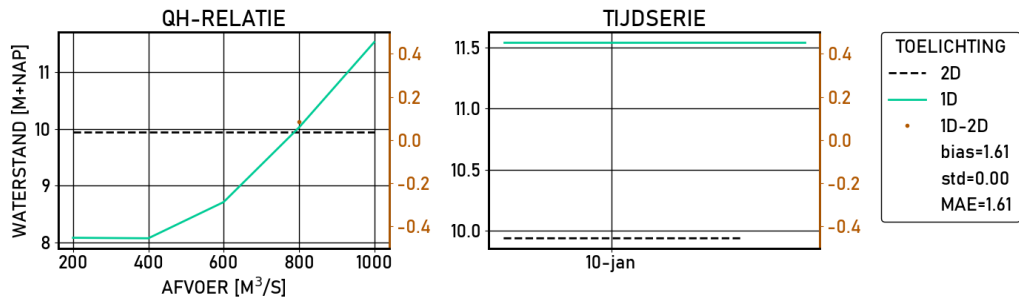
Figure 2.110 Hondsbroeksche-Pleij-IJ | figures | Validatie | S_6000 | stations
