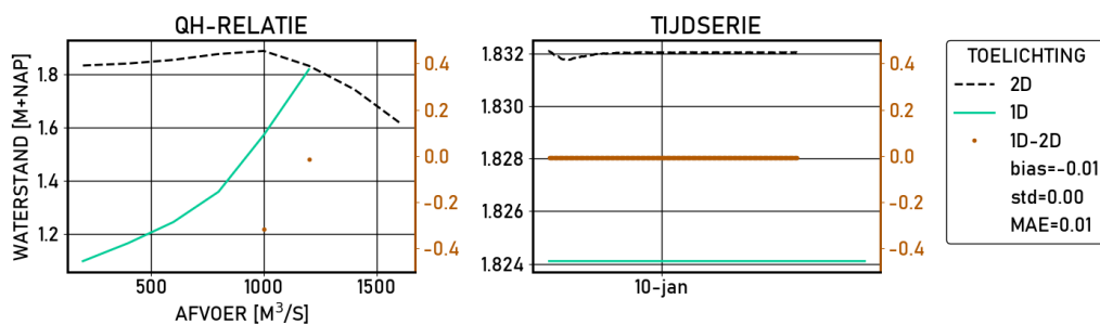
Figure 2.382 Schoonhoven | figures | Validatie | S_6000 | stations
