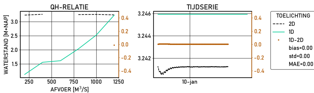
Figure 2.366 Hagestein-beneden | figures | Validatie | S_6000 | stations
