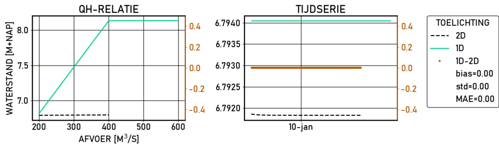
Figure 2.539 IJsselkop | figures | Validatie | S_1020 | stations
