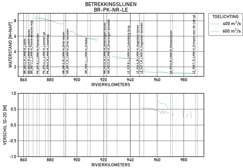
Figure 1.86 BR-PK-NR-LE | figures | Validatie | S_1020 | Langsprofiel
