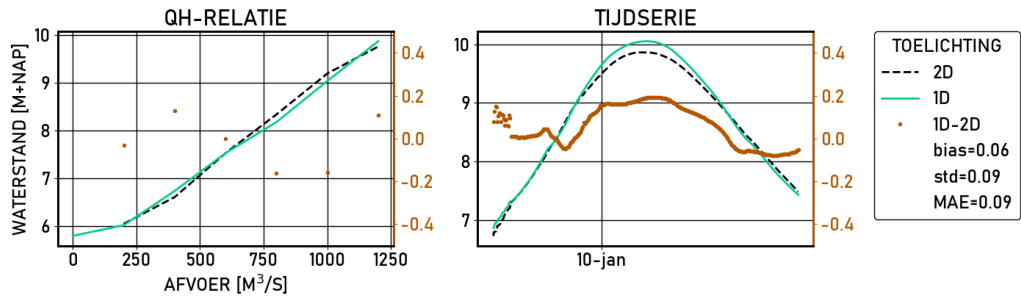
Figure 2.422 Driel-beneden | figures | Validatie | D_6000 | stations
