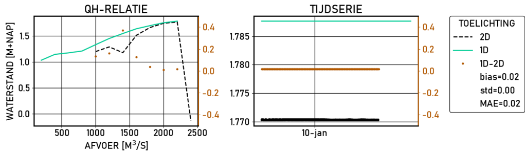
Figure 2.392 Krimpen-aan-de-Lek-g6 | figures | Validatie | S10000 | stations
