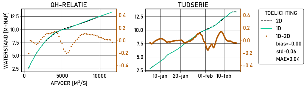
Figure 2.562 Dodewaard | figures | Kalibratie | stations
