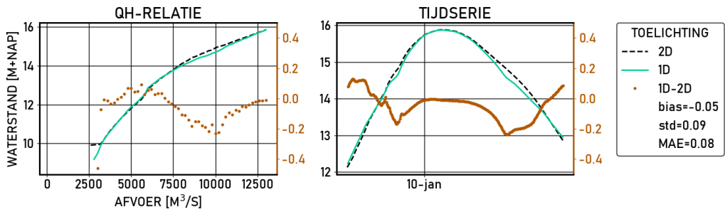
Figure 2.68 Pannerdensche-kop | figures | Validatie | D13000 | stations
