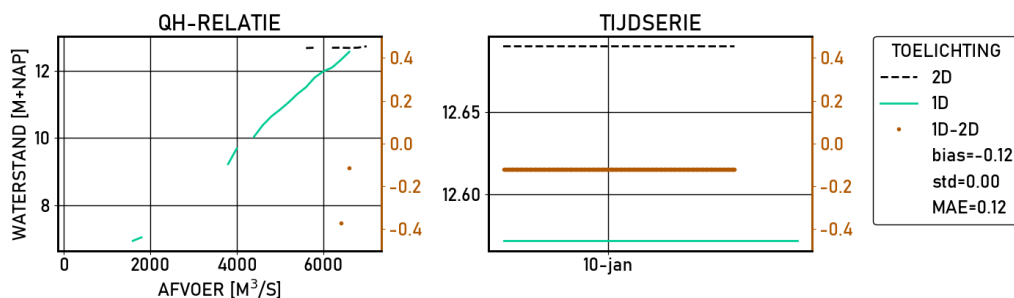
Figure 2.552 Nijmegen-haven | figures | Validatie | S10000 | stations
