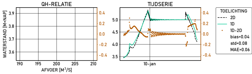
Figure 2.7 Tiel-Kanaal | figures | Validatie | D_8000 | stations
