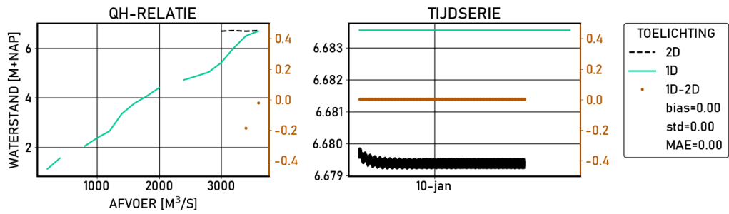
Figure 2.362 Hagestein-beneden | figures | Validatie | S16000 | stations
