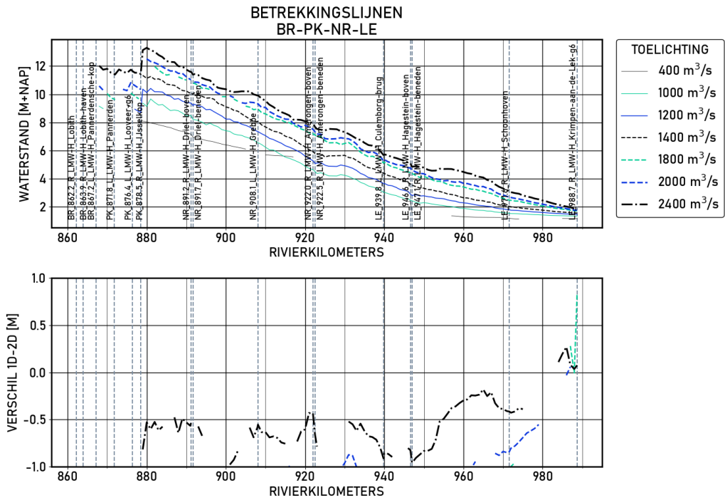
Figure 1.82 BR-PK-NR-LE | figures | Validatie | S13000 | Langsprofiel
