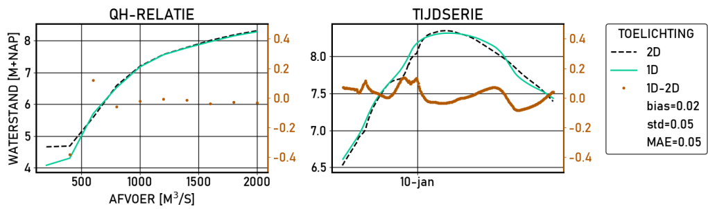
Figure 2.164 Zutphen-noord | figures | Validatie | D13000 | stations
