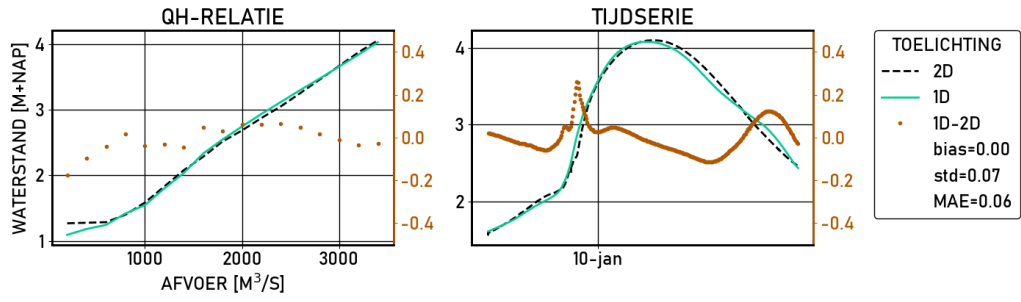
Figure 2.373 Schoonhoven | figures | Validatie | D16000 | stations
