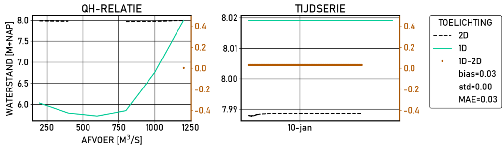
Figure 2.446 Grebbe | figures | Validatie | S_6000 | stations
