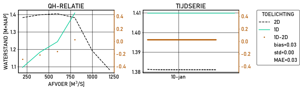
Figure 2.381 Schoonhoven | figures | Validatie | S_4000 | stations
