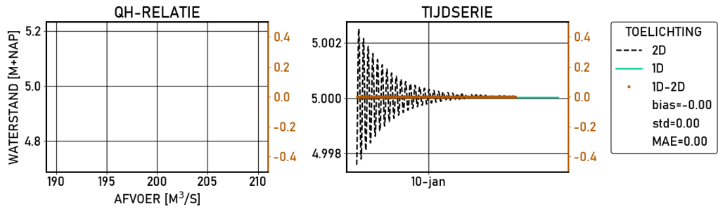
Figure 2.8 Tiel-Kanaal | figures | Validatie | S10000 | stations
