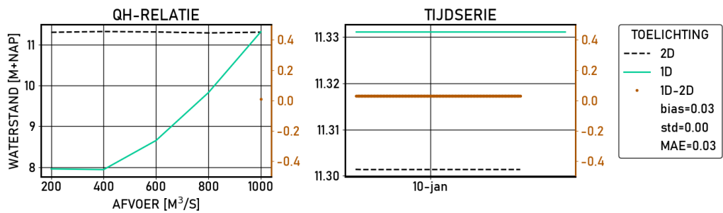
Figure 2.126 Westervoort-IJsseldijke | figures | Validatie | S_6000 | stations
