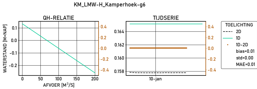
Figure 2.280 Kamperhoek-g6 | figures | Validatie | S10000 | stations
