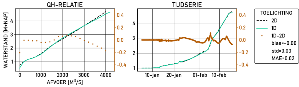
Figure 2.370 Schoonhoven | figures | Kalibratie | stations
