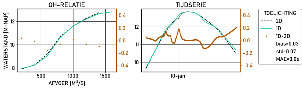
Figure 2.115 Westervoort-IJsseldijke | figures | Validatie | D10000 | stations
