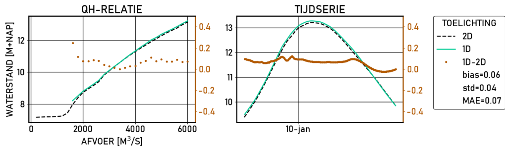
Figure 2.54 Lobith-haven | figures | Validatie | D_6000 | stations
