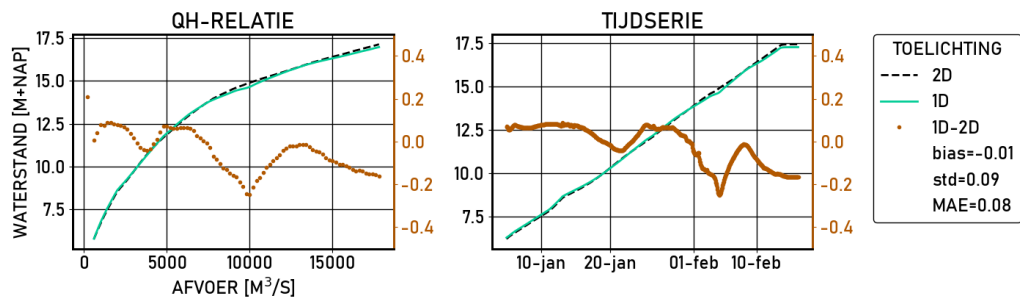
Figure 2.483 Pannerden | figures | Kalibratie | stations
