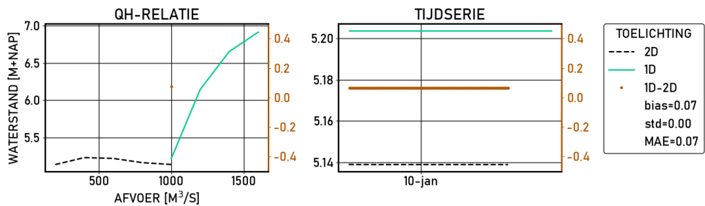
Figure 2.555 Nijmegen-haven | figures | Validatie | S_1020 | stations
