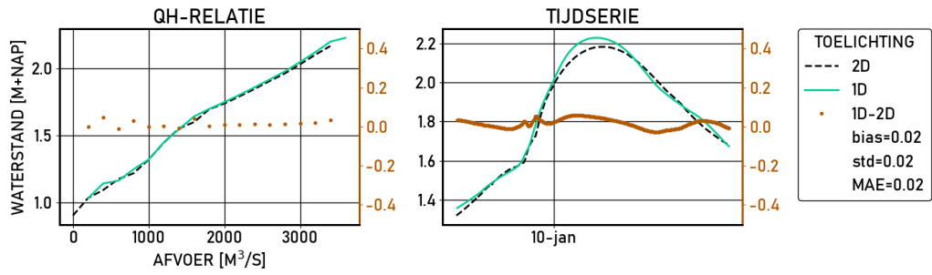
Figure 2.389 Krimpen-aan-de-Lek-g6 | figures | Validatie | D16000 | stations
