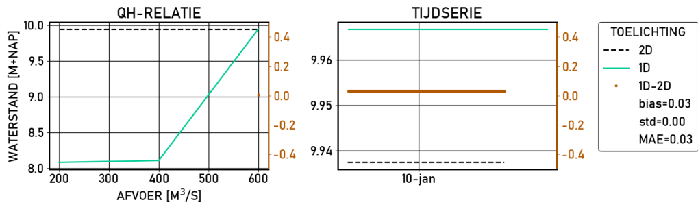
Figure 2.109 Hondsbroeksche-Pleij-IJ | figures | Validatie | S_4000 | stations
