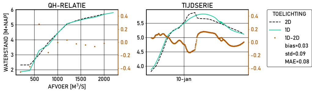
Figure 2.212 Olst | figures | Validatie | D13000 | stations
