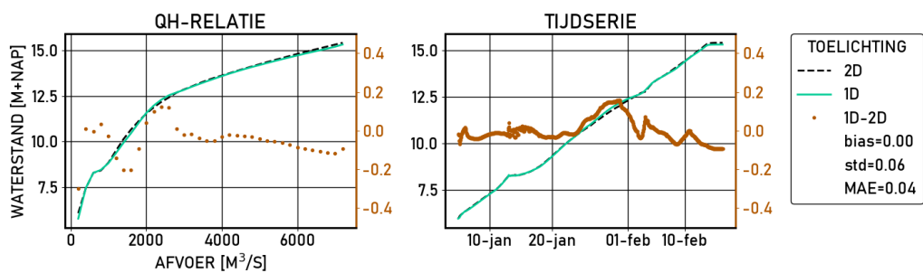
Figure 2.530 IJsselkop | figures | Kalibratie | stations
