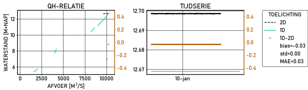
Figure 2.570 Dodewaard | figures | Validatie | S16000 | stations
