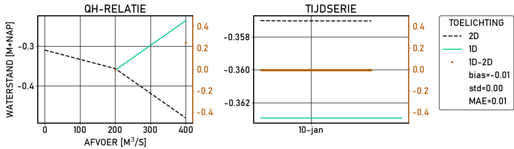
Figure 2.272 Kampen-bovenhaven | figures | Validatie | S_600 | stations
