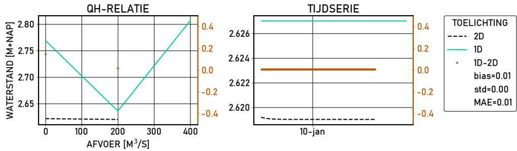
Figure 2.347 Hagestein-boven | figures | Validatie | S_1020 | stations
