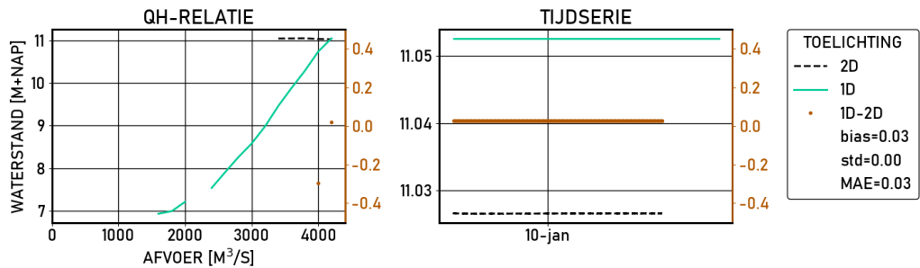
Figure 2.558 Nijmegen-haven | figures | Validatie | S_6000 | stations
