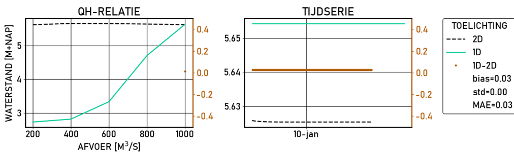
Figure 2.206 Deventer | figures | Validatie | S_6000 | stations
