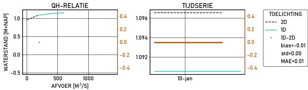
Figure 2.396 Krimpen-aan-de-Lek-g6 | figures | Validatie | S_2000 | stations
