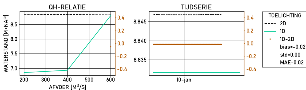
Figure 2.141 De-Steeg | figures | Validatie | S_4000 | stations
