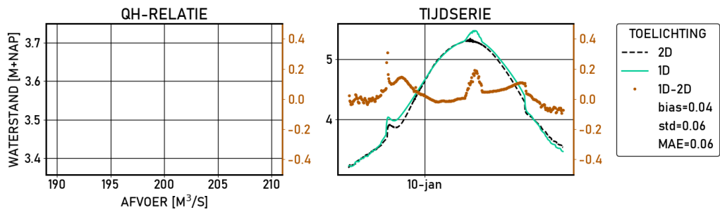
Figure 2.6 Tiel-Kanaal | figures | Validatie | D_6000 | stations
