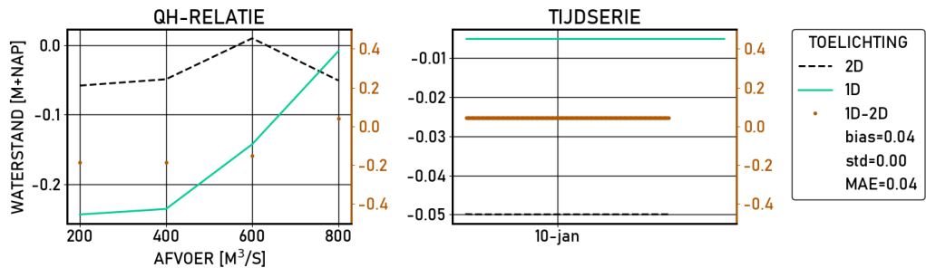
Figure 2.93 Keteldiep | figures | Validatie | S_4000 | stations
