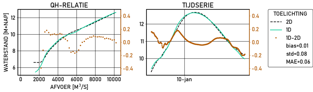
Figure 2.565 Dodewaard | figures | Validatie | D16000 | stations
