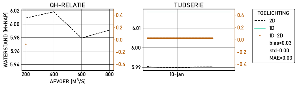
Figure 2.189 Eefde-beneden | figures | Validatie | S_4000 | stations
