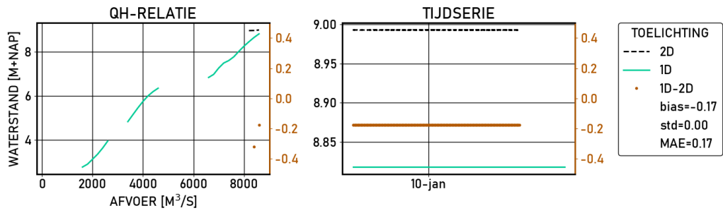
Figure 2.601 Sint-Andries-Waal-g6 | figures | Validatie | S13000 | stations
