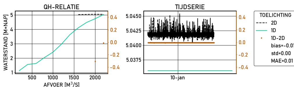
Figure 2.360 Hagestein-beneden | figures | Validatie | S10000 | stations
