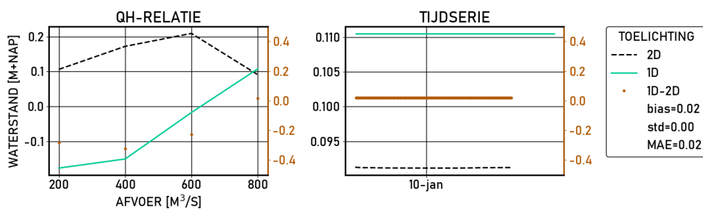
Figure 2.269 Kampen-bovenhaven | figures | Validatie | S_4000 | stations
