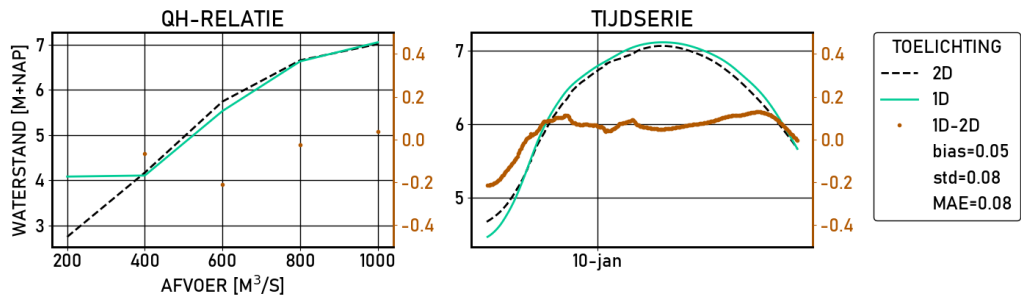
Figure 2.166 Zutphen-noord | figures | Validatie | D_6000 | stations
