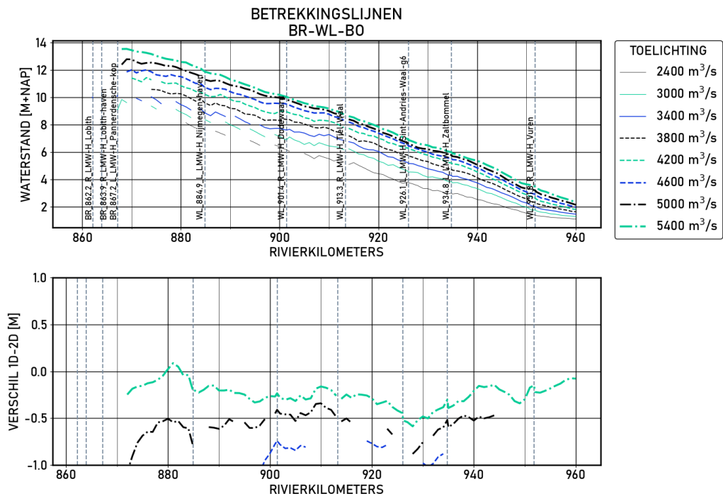
Figure 1.62 BR-WL-B0 | figures | Validatie | S_8000 | Langsprofiel
