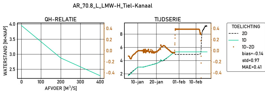
Figure 2.2 Tiel-Kanaal | figures | Kalibratie | stations
