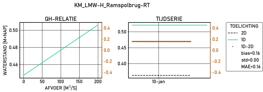
Figure 2.314 Ramspolbrug-RT | figures | Validatie | S16000 | stations
