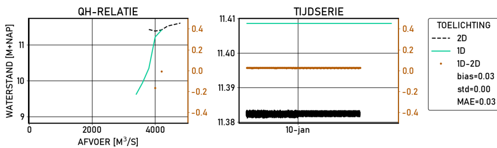
Figure 2.61 Lobith-haven | figures | Validatie | S_4000 | stations
