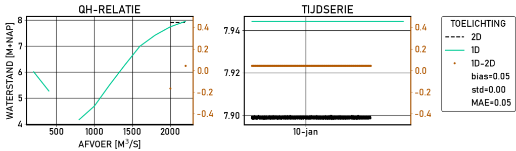
Figure 2.456 Amerongen-boven | figures | Validatie | S10000 | stations
