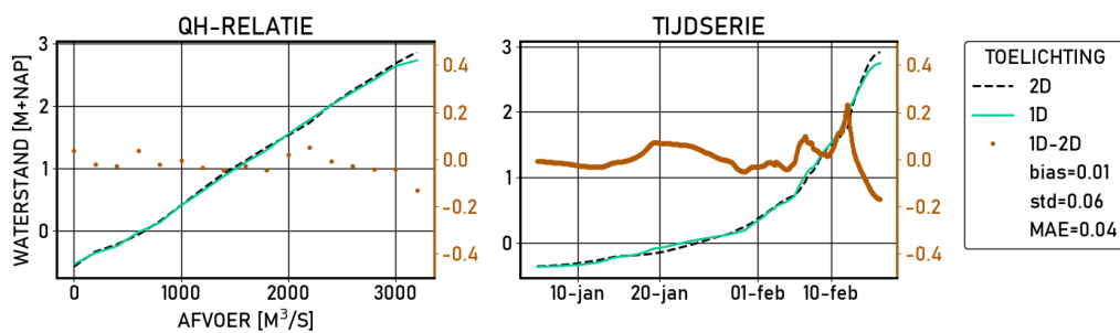
Figure 2.258 Kampen-bovenhaven | figures | Kalibratie | stations
