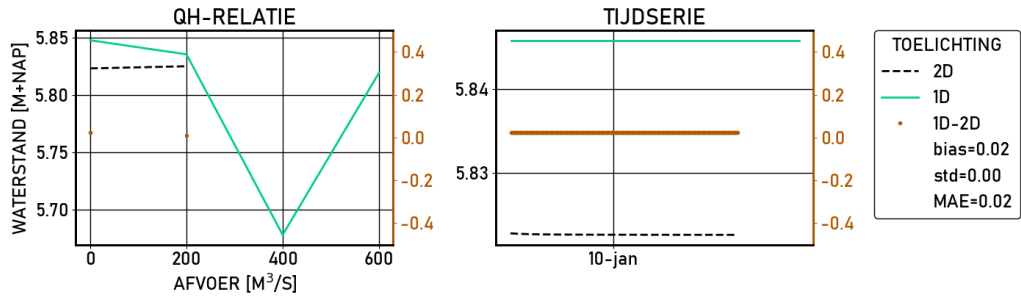
Figure 2.448 Grebbe | figures | Validatie | S__600 | stations
