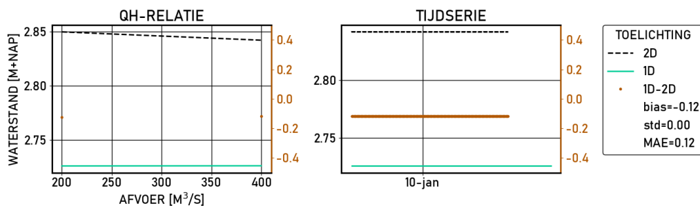
Figure 2.204 Deventer | figures | Validatie | S_2000 | stations
