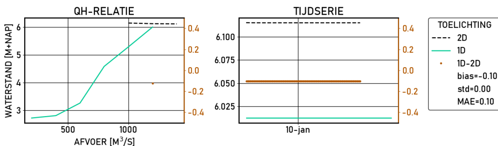
Figure 2.207 Deventer | figures | Validatie | S_8000 | stations
