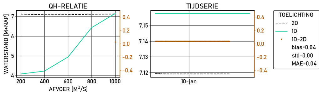
Figure 2.174 Zutphen-noord | figures | Validatie | S_6000 | stations
