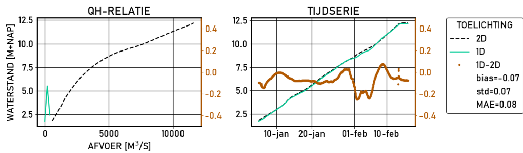
Figure 2.578 Tiel-Waal | figures | Kalibratie | stations
