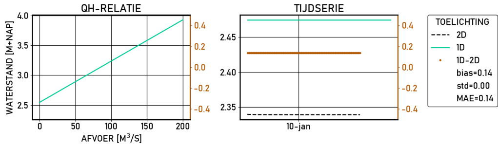
Figure 2.187 Eefde-beneden | figures | Validatie | S_1020 | stations
