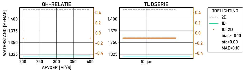
Figure 2.236 Wijhe | figures | Validatie | S_2000 | stations
