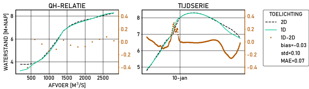
Figure 2.468 Amerongen-beneden | figures | Validatie | D13000 | stations
