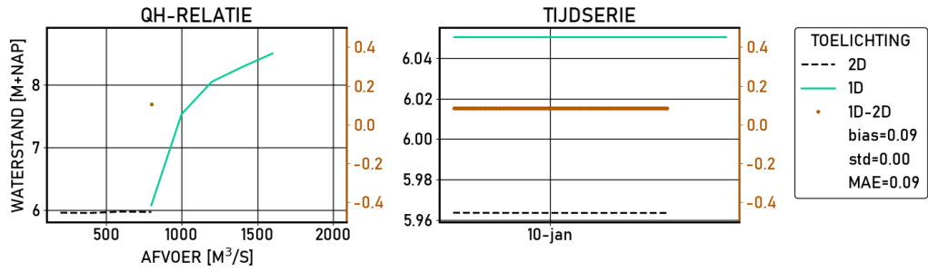
Figure 2.511 Pannerden | figures | Validatie | S__600 | stations
