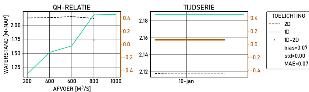
Figure 2.365 Hagestein-beneden | figures | Validatie | S_4000 | stations
