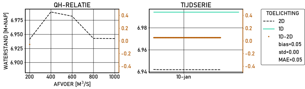
Figure 2.190 Eefde-beneden | figures | Validatie | S_6000 | stations
