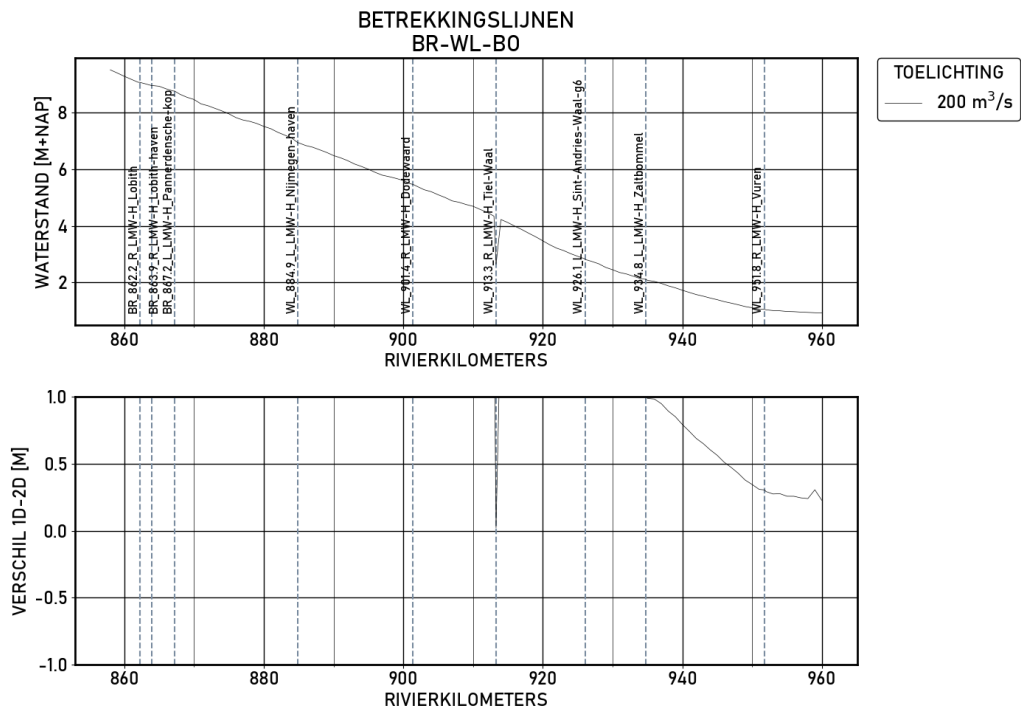
Figure 1.54 BR-WL-B0 | figures | Validatie | S_1020 | Langsprofiel
