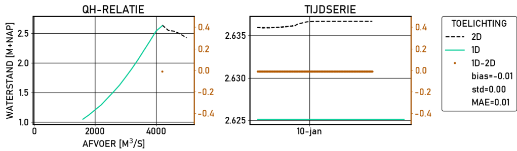
Figure 2.638 Vuren | figures | Validatie | S_6000 | stations
