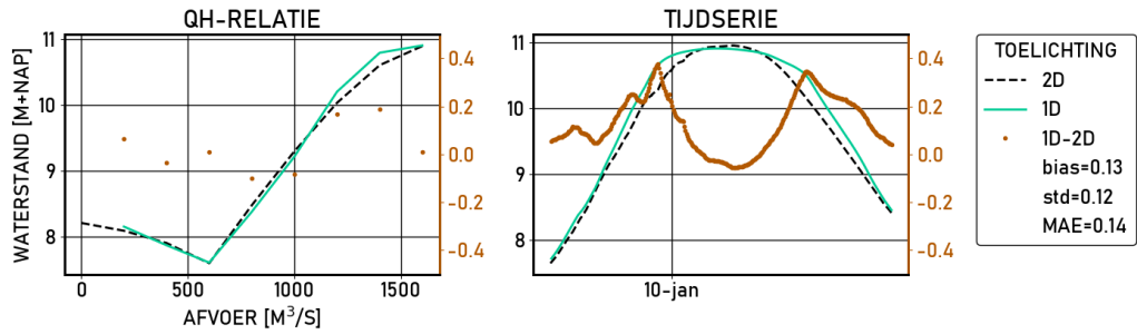
Figure 2.407 Driel-boven | figures | Validatie | D_8000 | stations
