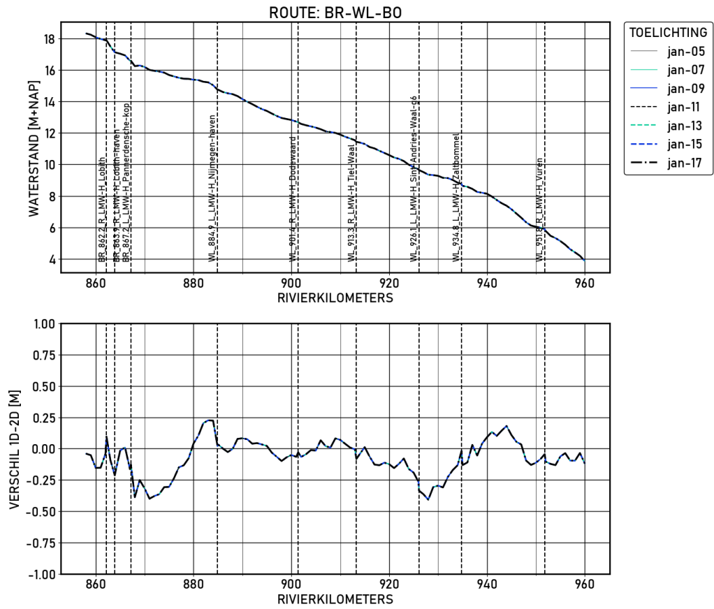
Figure 1.51 BR-WL-B0 | figures | Validatie | S16000 | Langsprofiel
