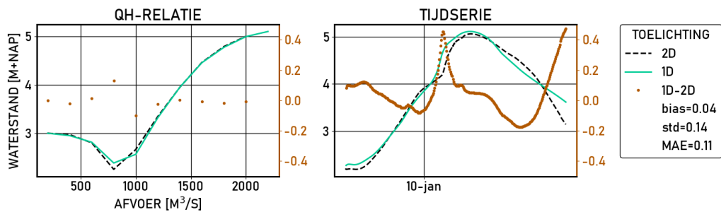
Figure 2.339 Hagestein-boven | figures | Validatie | D10000 | stations
