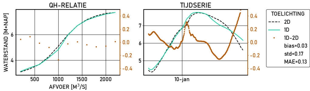
Figure 2.467 Amerongen-beneden | figures | Validatie | D10000 | stations
