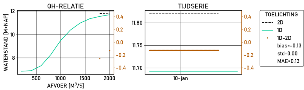
Figure 2.137 De-Steeg | figures | Validatie | S13000 | stations
