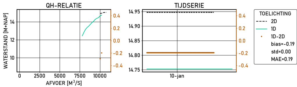
Figure 2.72 Pannerdensche-kop | figures | Validatie | S10000 | stations
