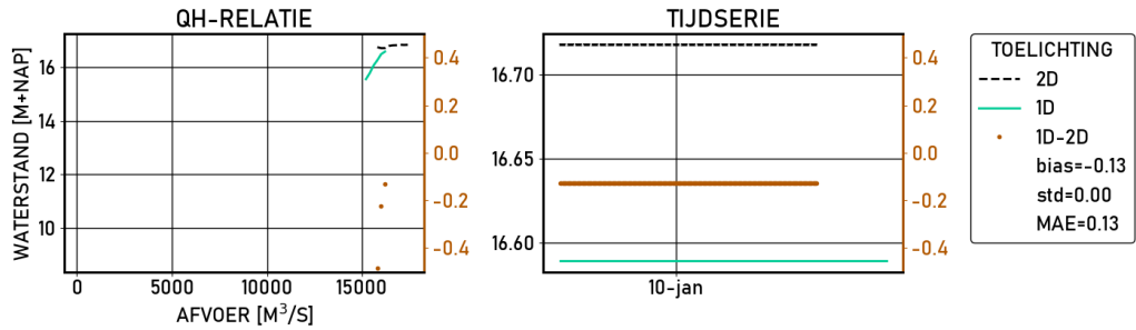
Figure 2.74 Pannerdensche-kop | figures | Validatie | S16000 | stations
