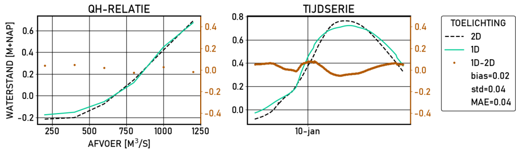
Figure 2.263 Kampen-bovenhaven | figures | Validatie | D_8000 | stations
