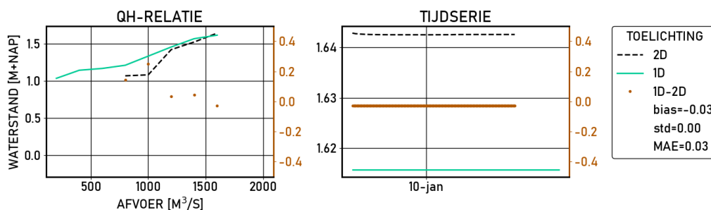
Figure 2.399 Krimpen-aan-de-Lek-g6 | figures | Validatie | S_8000 | stations
