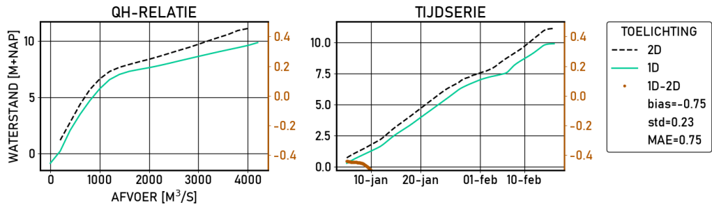
Figure 2.465 Amerongen-beneden | figures | Ongekalibreerd | stations
