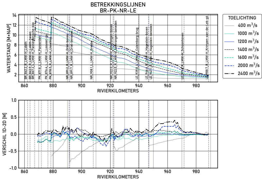
Figure 1.72 BR-PK-NR-LE | figures | Validatie | D13000 | Langsprofiel
