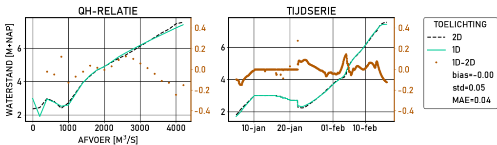
Figure 2.338 Hagestein-boven | figures | Kalibratie | stations
