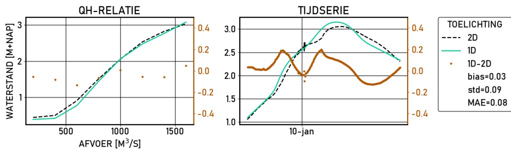
Figure 2.243 Katerveer | figures | Validatie | D10000 | stations
