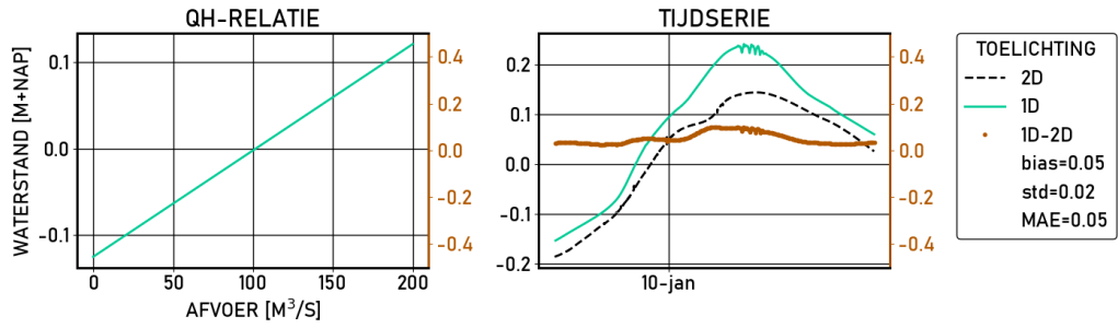
Figure 2.307 Ramspolbrug-RT | figures | Validatie | D10000 | stations
