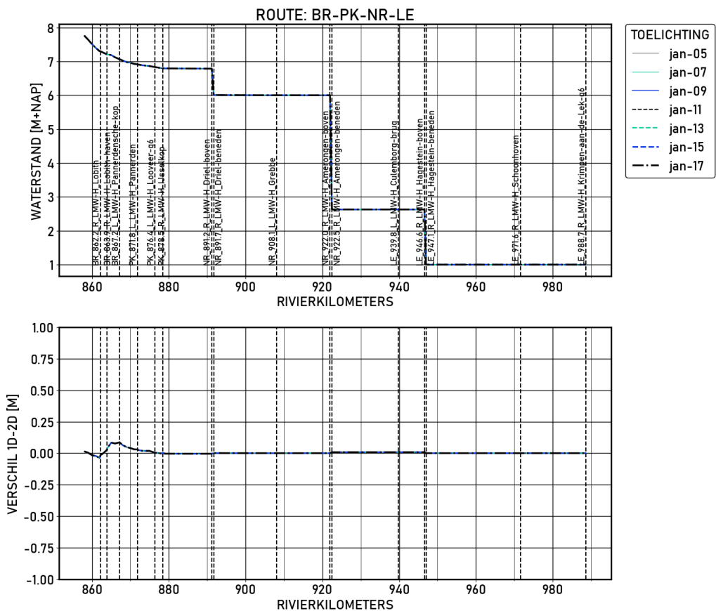
Figure 1.85 BR-PK-NR-LE | figures | Validatie | S_1020 | Langsprofiel
