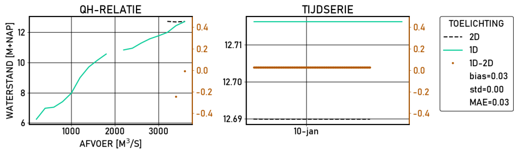
Figure 2.426 Driel-beneden | figures | Validatie | S16000 | stations
