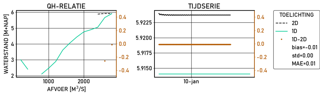
Figure 2.345 Hagestein-boven | figures | Validatie | S13000 | stations
