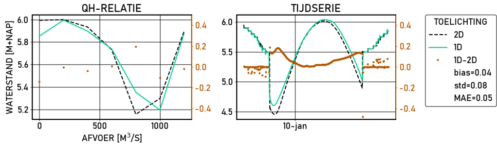
Figure 2.454 Amerongen-boven | figures | Validatie | D_6000 | stations
