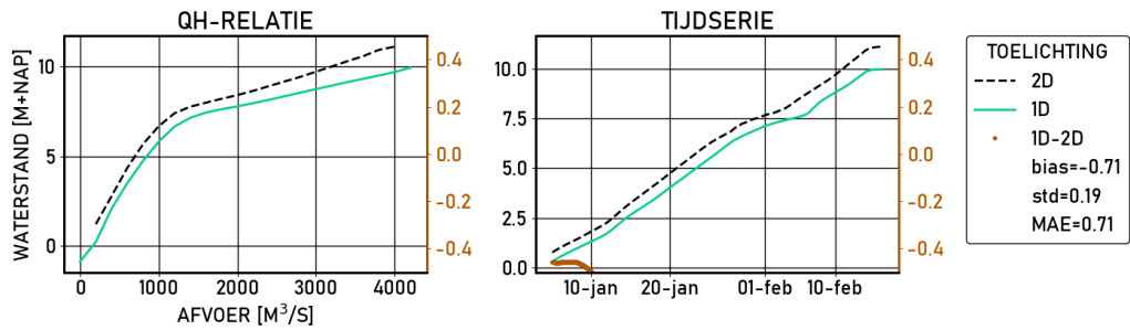
Figure 2.449 Amerongen-boven | figures | Ongekalibreerd | stations
