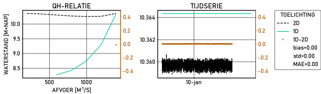
Figure 2.525 Looveer-g6 | figures | Validatie | S_4000 | stations
