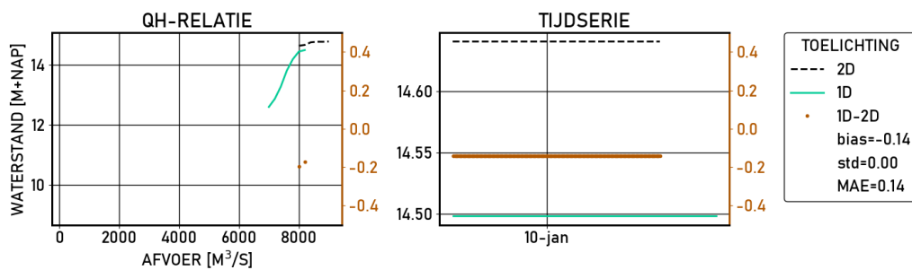
Figure 2.63 Lobith-haven | figures | Validatie | S_8000 | stations
