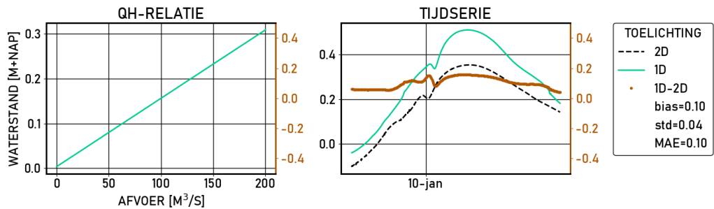
Figure 2.309 Ramspolbrug-RT | figures | Validatie | D16000 | stations
