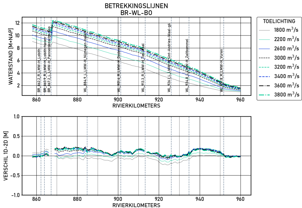
Figure 1.44 BR-WL-B0 | figures | Validatie | D_6000 | Langsprofiel
