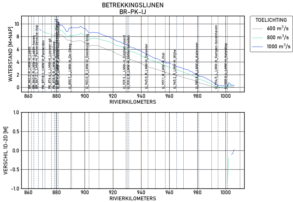
Figure 1.18 BR-PK-IJ | figures | Validatie | S13000 | Langsprofiel
