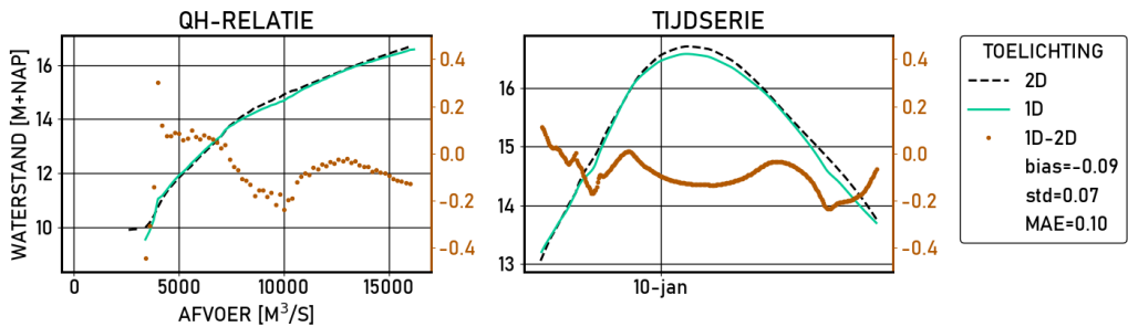
Figure 2.69 Pannerdensche-kop | figures | Validatie | D16000 | stations
