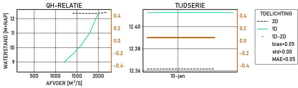
Figure 2.508 Pannerden | figures | Validatie | S_6000 | stations
