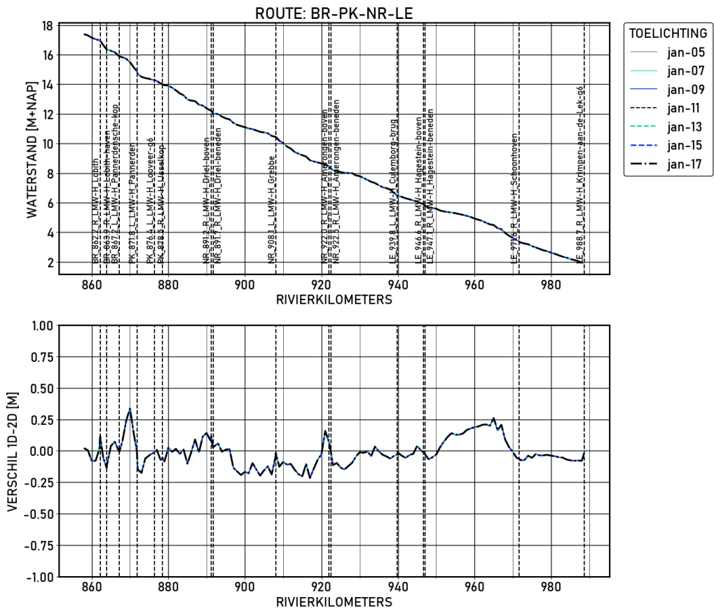
Figure 1.81 BR-PK-NR-LE | figures | Validatie | S13000 | Langsprofiel
