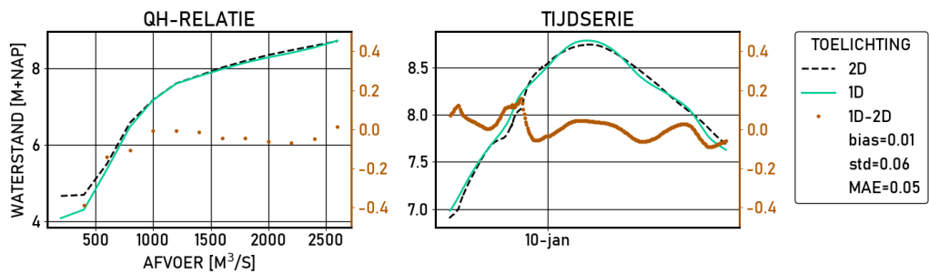
Figure 2.165 Zutphen-noord | figures | Validatie | D16000 | stations
