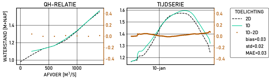
Figure 2.391 Krimpen-aan-de-Lek-g6 | figures | Validatie | D_8000 | stations
