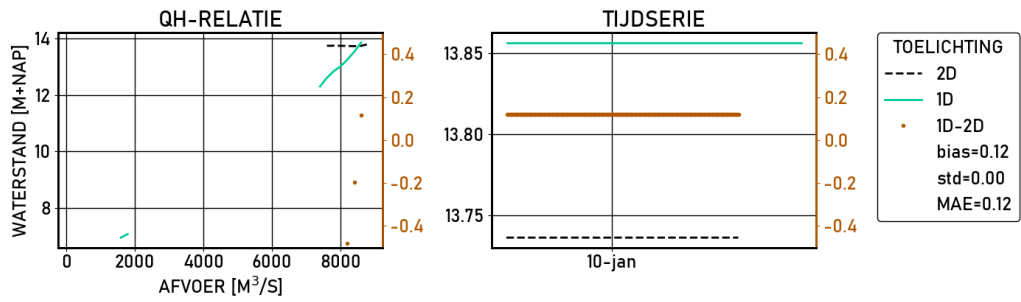
Figure 2.553 Nijmegen-haven | figures | Validatie | S13000 | stations
