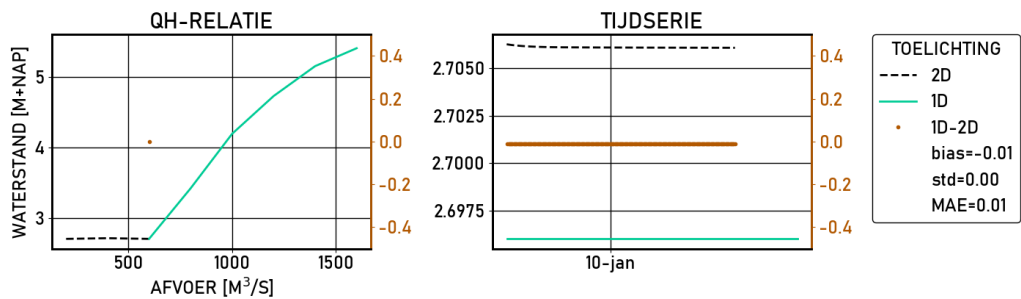
Figure 2.576 Dodewaard | figures | Validatie | S_600 | stations
