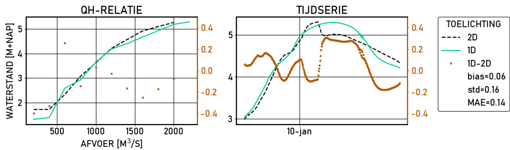
Figure 2.228 Wijhe | figures | Validatie | D13000 | stations
