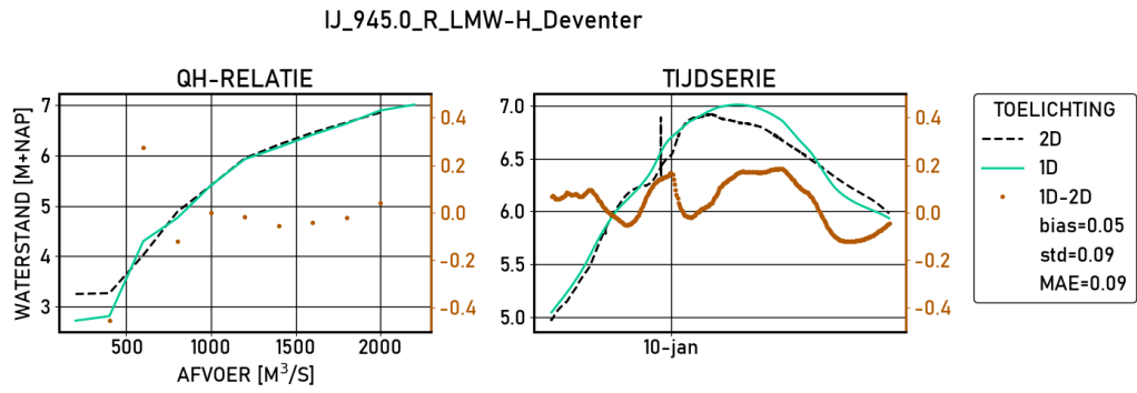
Figure 2.196 Deventer | figures | Validatie | D13000 | stations
