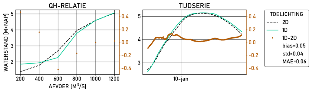
Figure 2.215 Olst | figures | Validatie | D_8000 | stations
