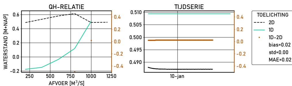
Figure 2.270 Kampen-bovenhaven | figures | Validatie | S_6000 | stations
