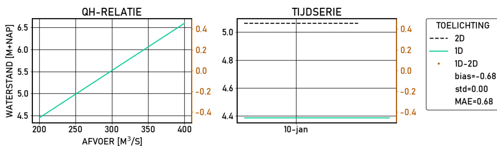
Figure 2.144 De-Steeg | figures | Validatie | S__600 | stations
