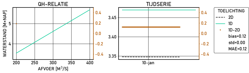
Figure 2.160 Doesburg-brug | figures | Validatie | S__600 | stations
