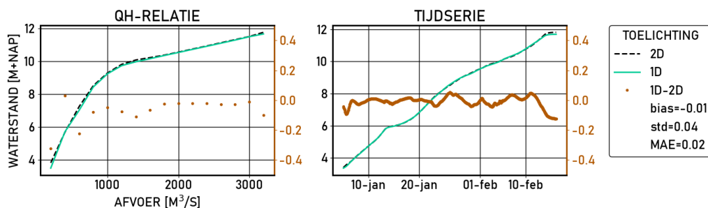
Figure 2.146 Doesburg-brug | figures | Kalibratie | stations
