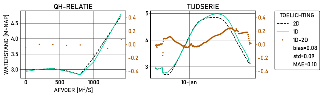
Figure 2.327 Culemborg-brug | figures | Validatie | D_8000 | stations
