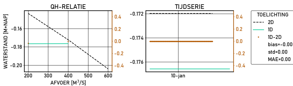
Figure 2.268 Kampen-bovenhaven | figures | Validatie | S_2000 | stations
