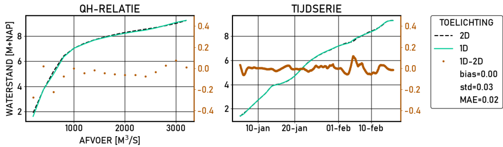
Figure 2.162 Zutphen-noord | figures | Kalibratie | stations
