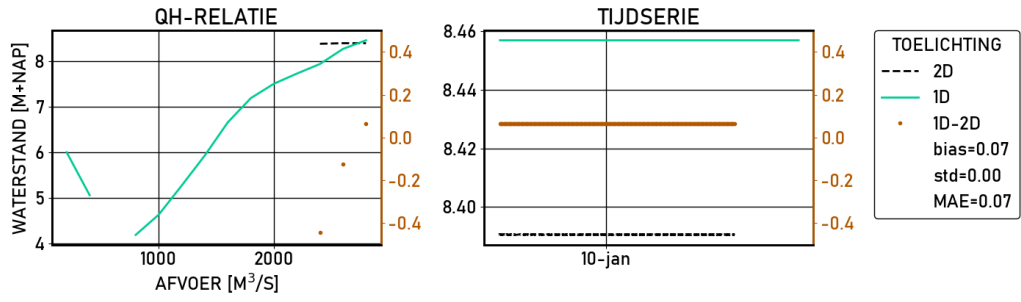
Figure 2.457 Amerongen-boven | figures | Validatie | S13000 | stations
