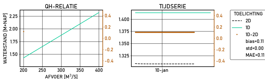
Figure 2.203 Deventer | figures | Validatie | S_1020 | stations
