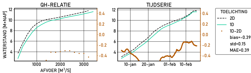
Figure 2.145 Doesburg-brug | figures | Ongekalibreerd | stations
