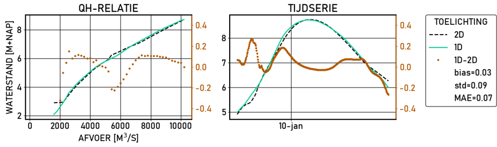
Figure 2.613 Zaltbommel | figures | Validatie | D16000 | stations
