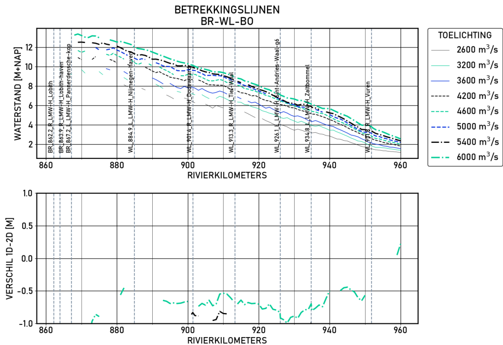
Figure 1.48 BR-WL-B0 | figures | Validatie | S10000 | Langsprofiel
