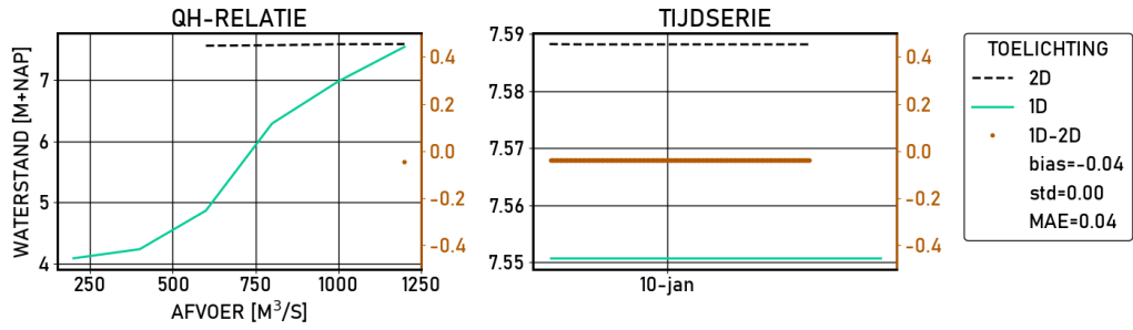
Figure 2.175 Zutphen-noord | figures | Validatie | S_8000 | stations
