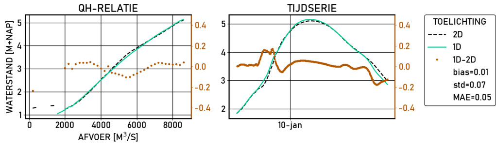
Figure 2.628 Vuren | figures | Validatie | D13000 | stations
