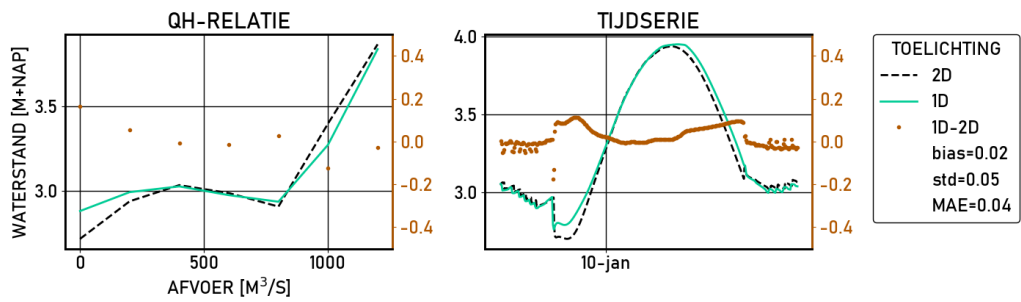
Figure 2.326 Culemborg-brug | figures | Validatie | D_6000 | stations
