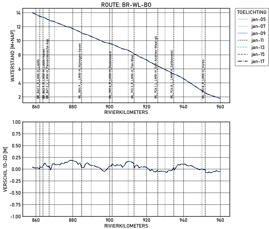
Figure 1.59 BR-WL-B0 | figures | Validatie | S_6000 | Langsprofiel
