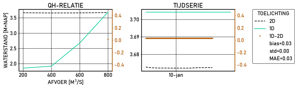
Figure 2.221 Olst | figures | Validatie | S_4000 | stations
