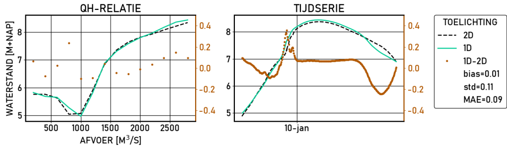
Figure 2.452 Amerongen-boven | figures | Validatie | D13000 | stations
