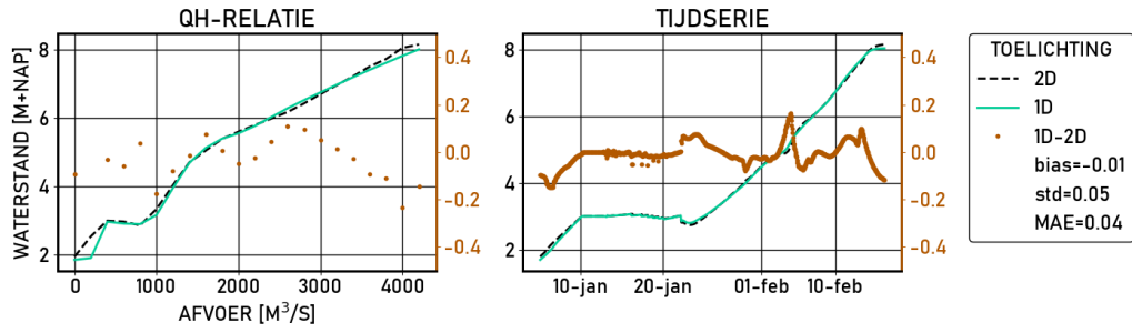
Figure 2.322 Culemborg-brug | figures | Kalibratie | stations
