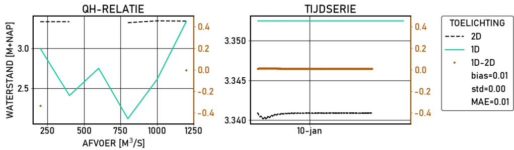
Figure 2.350 Hagestein-boven | figures | Validatie | S_6000 | stations
