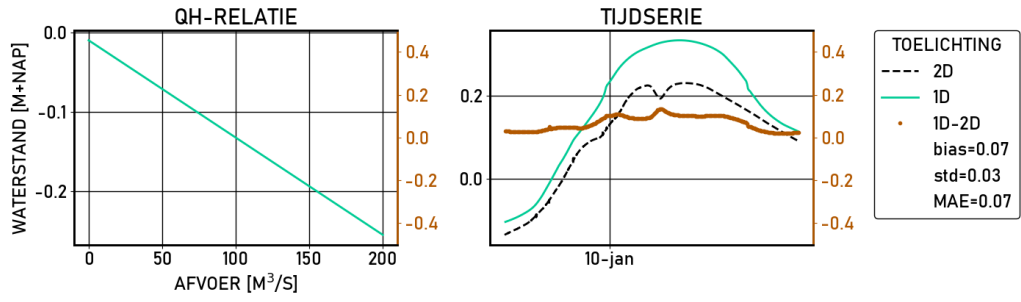
Figure 2.292 Ketelhaven | figures | Validatie | D13000 | stations
