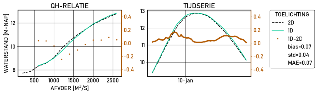
Figure 2.519 Looweer-g6 | figures | Validatie | D_8000 | stations
