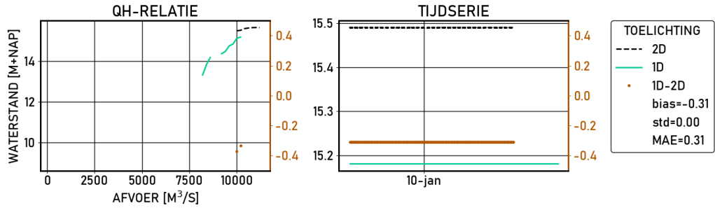
Figure 2.56 Lobith-haven | figures | Validatie | S10000 | stations
