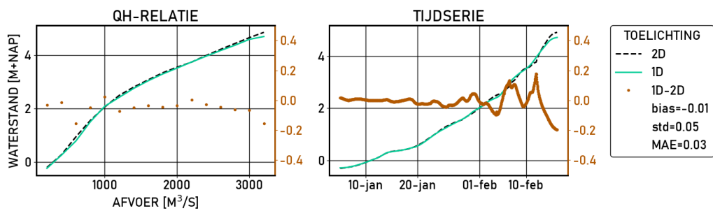
Figure 2.242 Katerveer | figures | Kalibratie | stations
