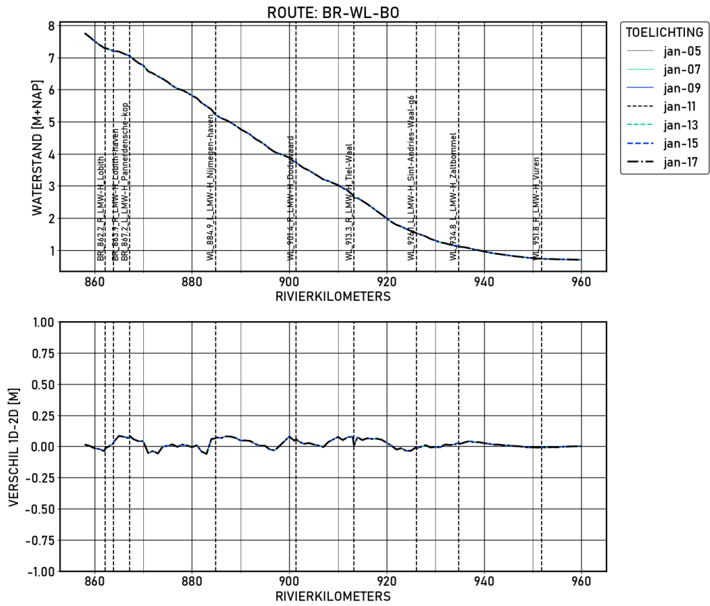
Figure 1.53 BR-WL-B0 | figures | Validatie | S_1020 | Langsprofiel
