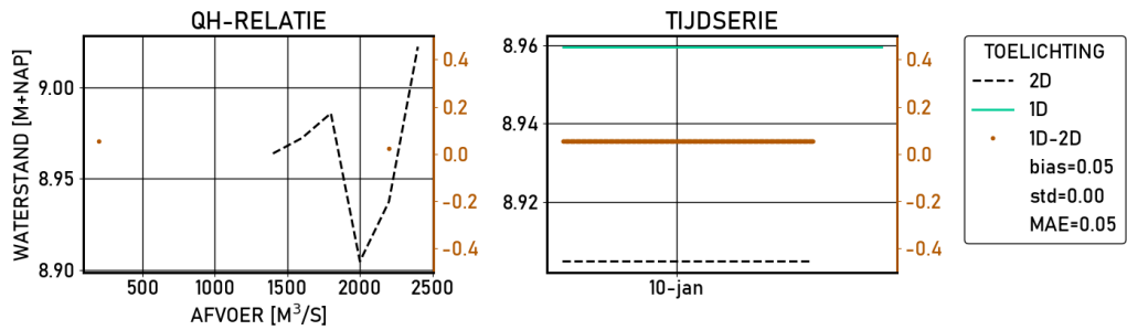
Figure 2.60 Lobith-haven | figures | Validatie | S_2000 | stations
