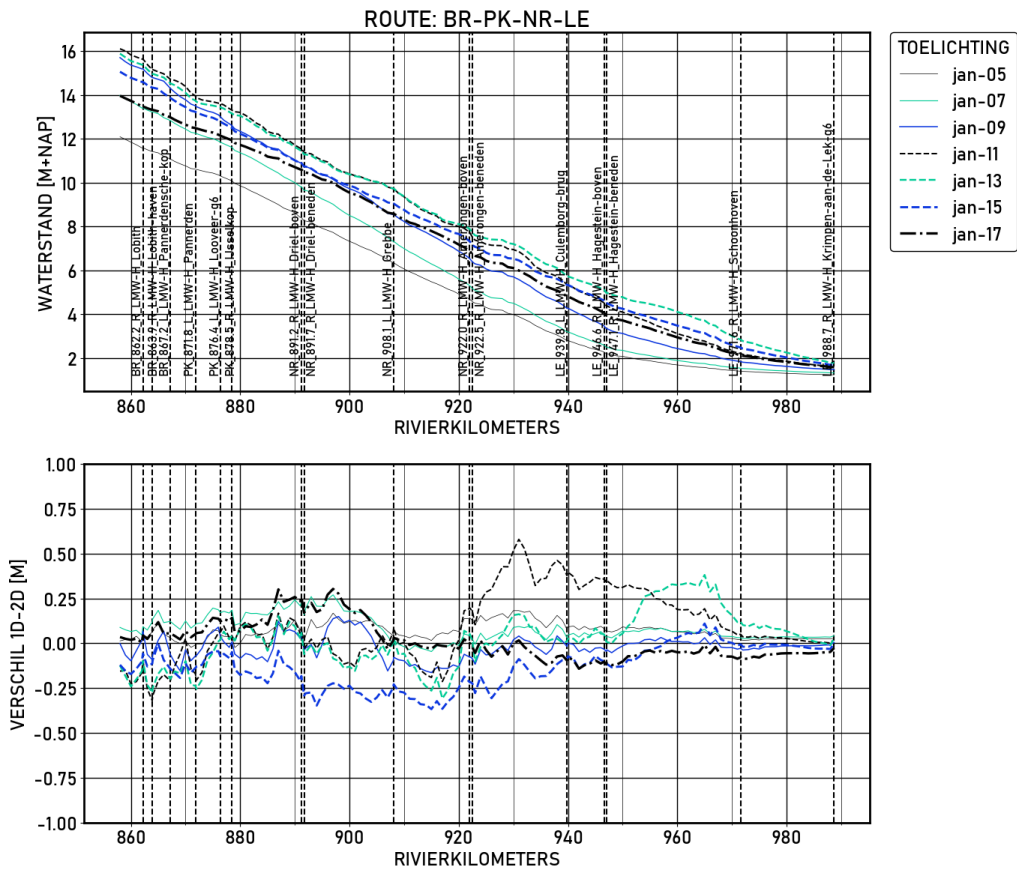
Figure 1.69 BR-PK-NR-LE | figures | Validatie | D10000 | Langsprofiel
