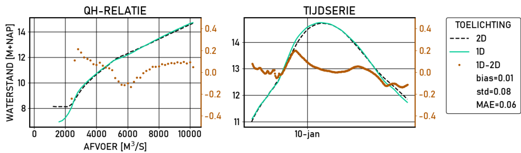
Figure 2.549 Nijmegen-haven | figures | Validatie | D16000 | stations
