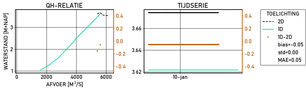
Figure 2.639 Vuren | figures | Validatie | S_8000 | stations
