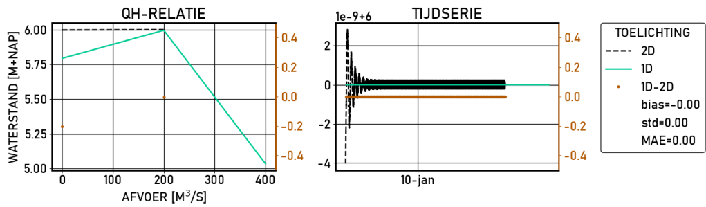
Figure 2.459 Amerongen-boven | figures | Validatie | S_1020 | stations
