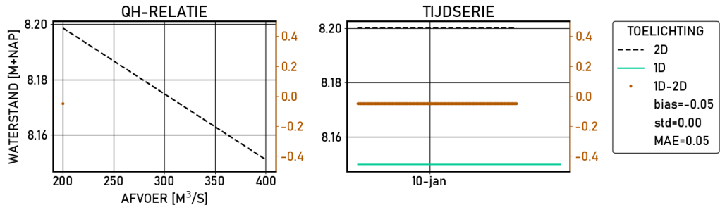
Figure 2.412 Driel-boven | figures | Validatie | S_2000 | stations
