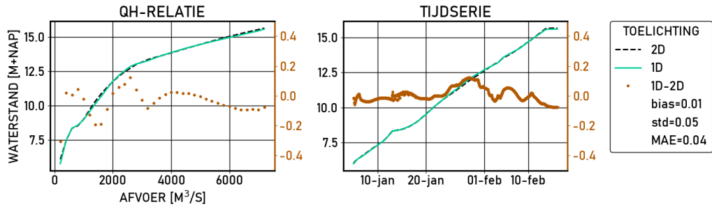
Figure 2.514 Looweer-g6 | figures | Kalibratie | stations
