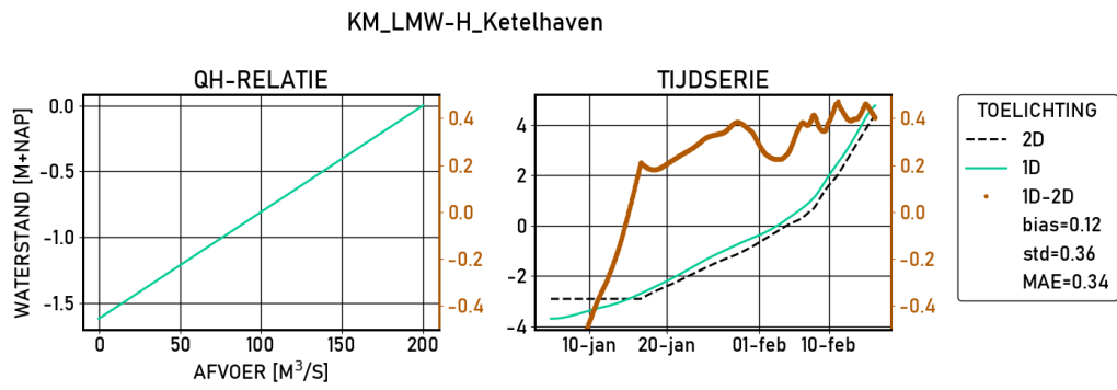
Figure 2.289 Ketelhaven | figures | Ongekalibreerd | stations
