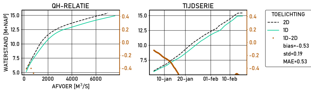
Figure 2.529 IJsselkop | figures | Ongekalibreerd | stations
