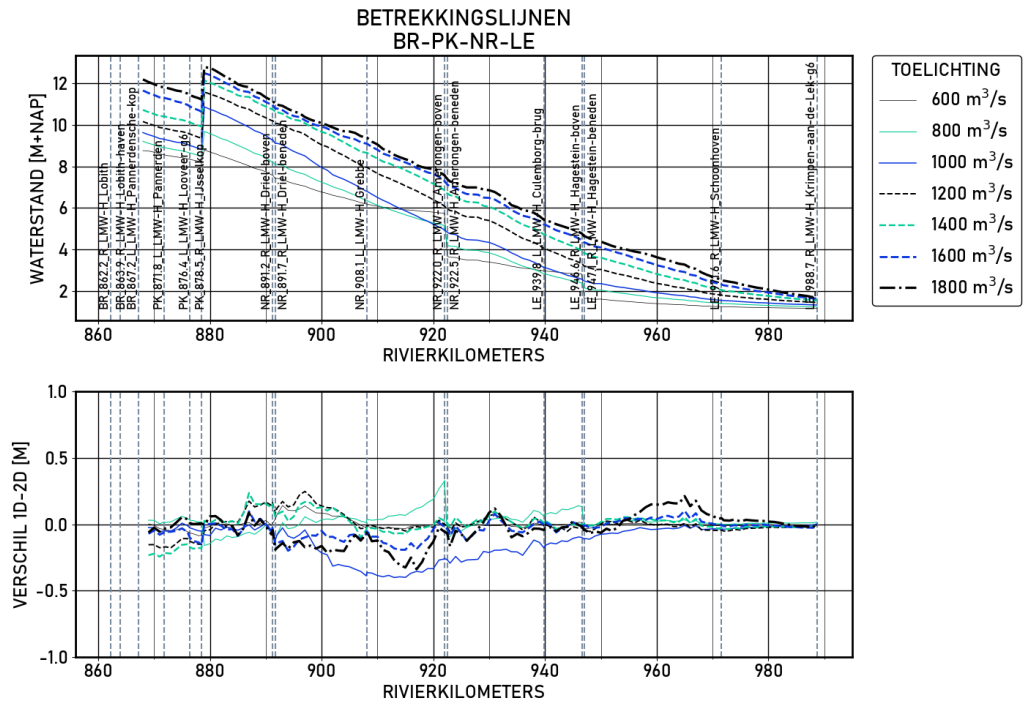
Figure 1.70 BR-PK-NR-LE | figures | Validatie | D1000 | Langsprofiel
