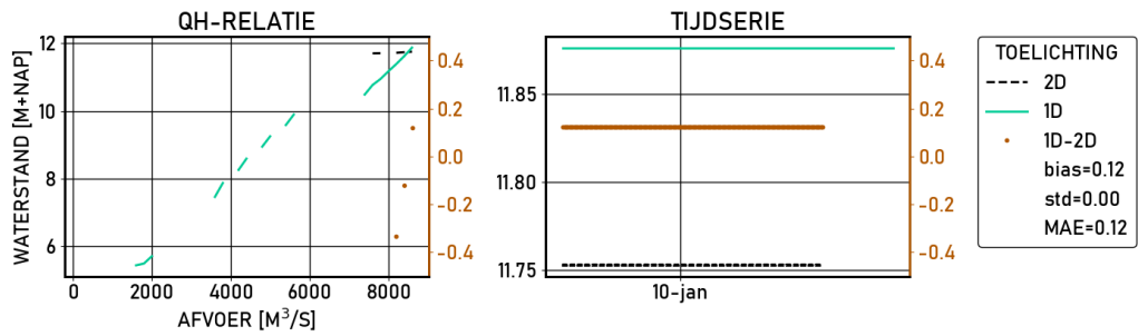
Figure 2.569 Dodewaard | figures | Validatie | S13000 | stations
