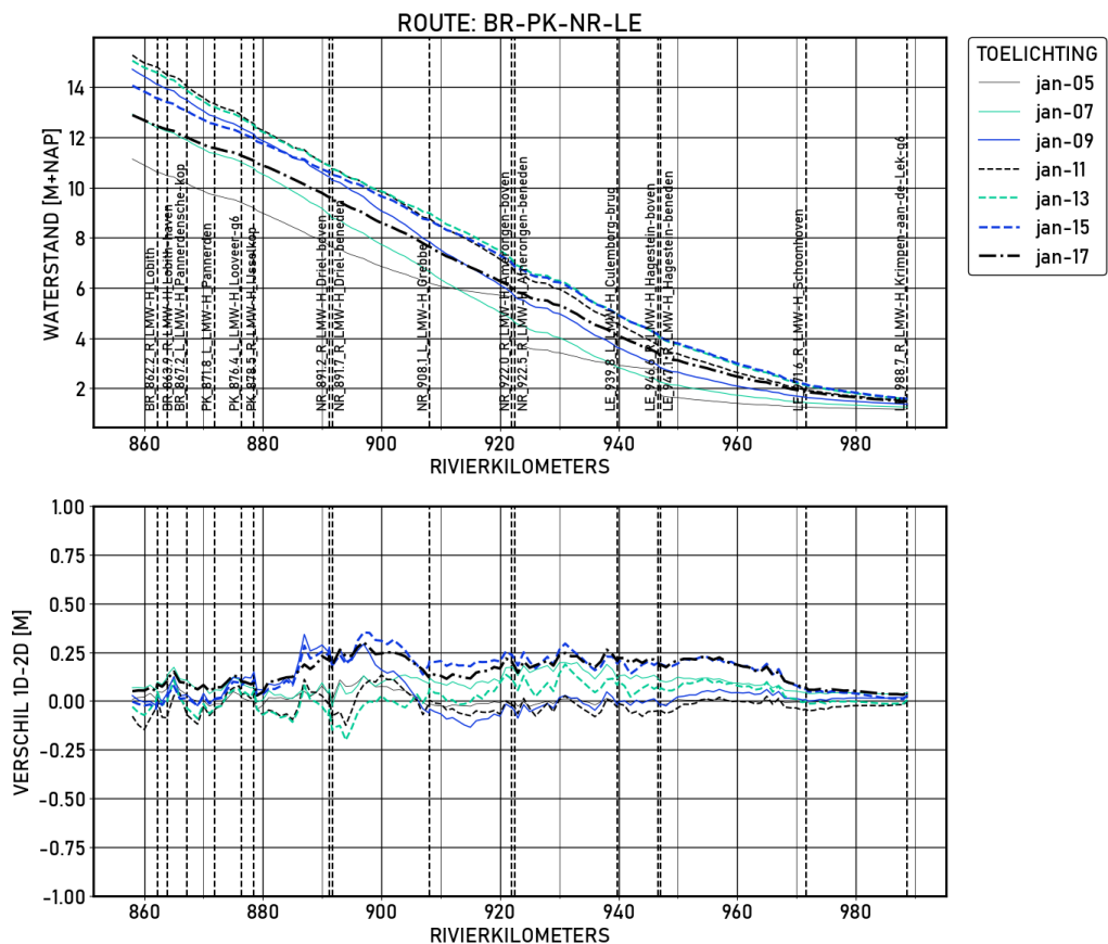
Figure 1.77 BR-PK-NR-LE | figures | Validatie | D_8000 | Langsprofiel
