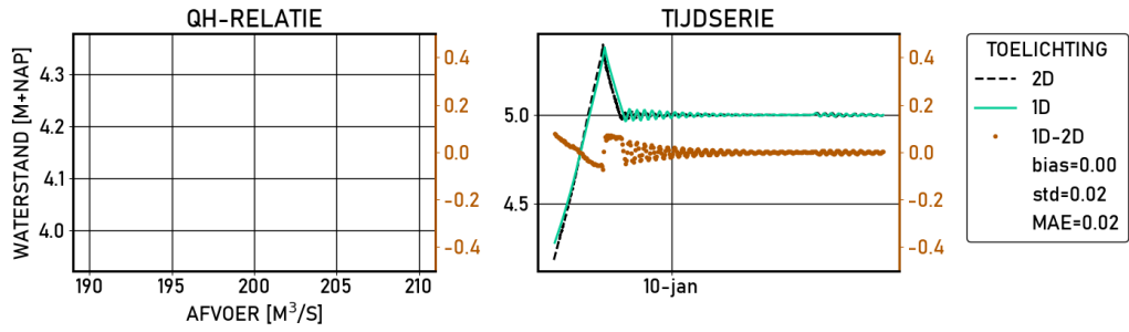
Figure 2.4 Tiel-Kanaal | figures | Validatie | D13000 | stations
