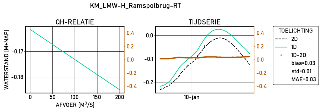
Figure 2.310 Ramspolbrug-RT | figures | Validatie | D_6000 | stations
