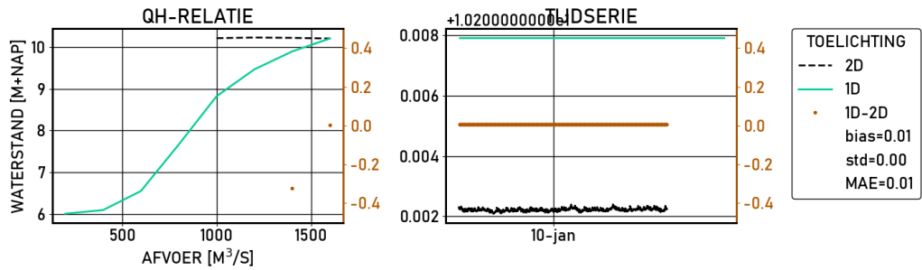
Figure 2.152 Doesburg-brug | figures | Validatie | S10000 | stations
