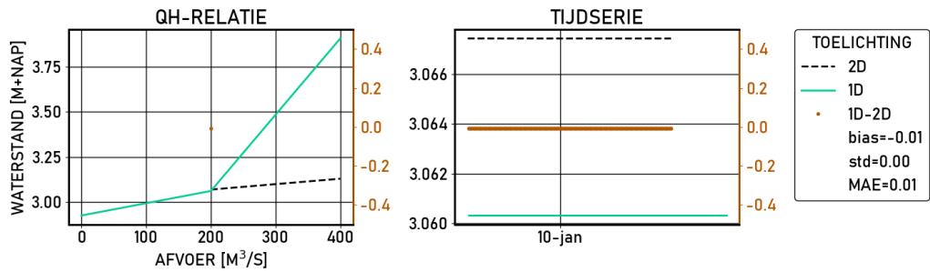
Figure 2.476 Amerongen-beneden | figures | Validatie | S_2000 | stations
