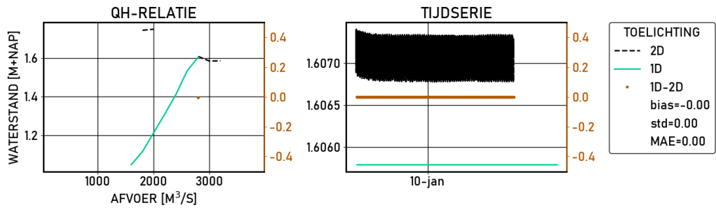
Figure 2.637 Vuren | figures | Validatie | S_4000 | stations
