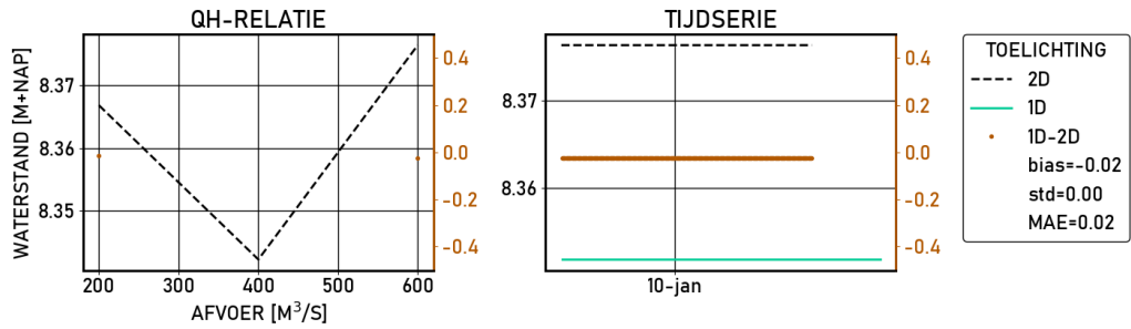
Figure 2.524 Looveer-g6 | figures | Validatie | S_2000 | stations
