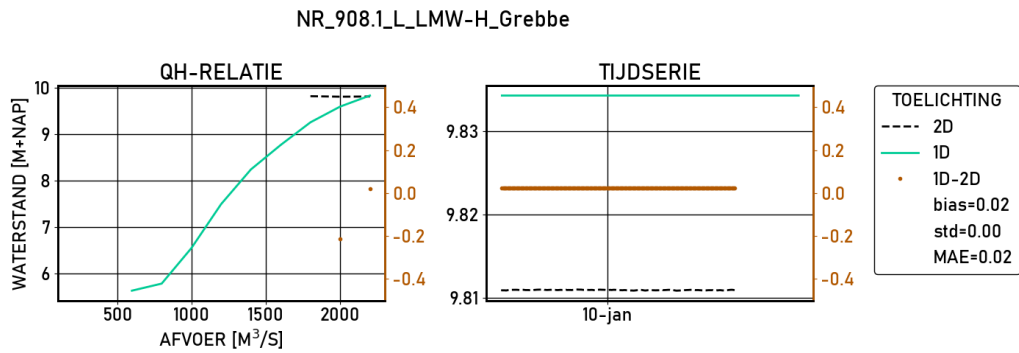
Figure 2.440 Grebbe | figures | Validatie | S10000 | stations
