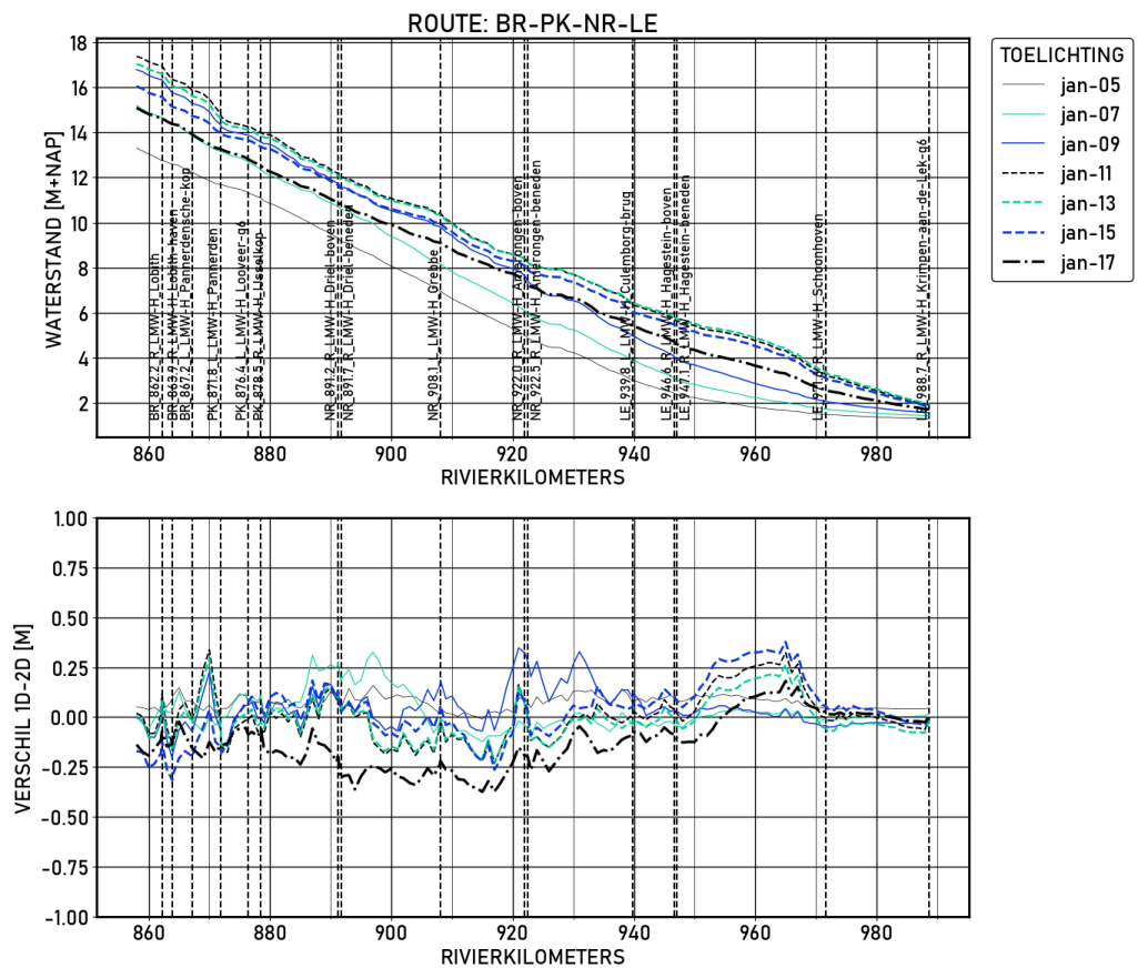
Figure 1.71 BR-PK-NR-LE | figures | Validatie | D13000 | Langsprofiel
