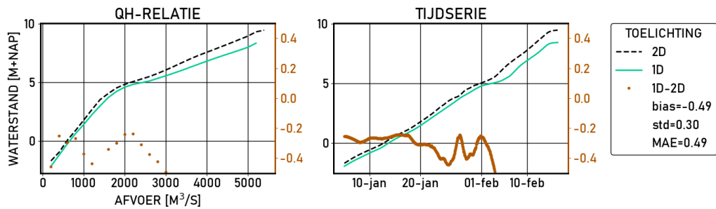
Figure 2.337 Hagestein-boven | figures | Ongekalibreerd | stations
