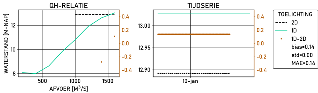
Figure 2.104 Hondsbroeksche-Pleij-IJ | figures | Validatie | S10000 | stations
