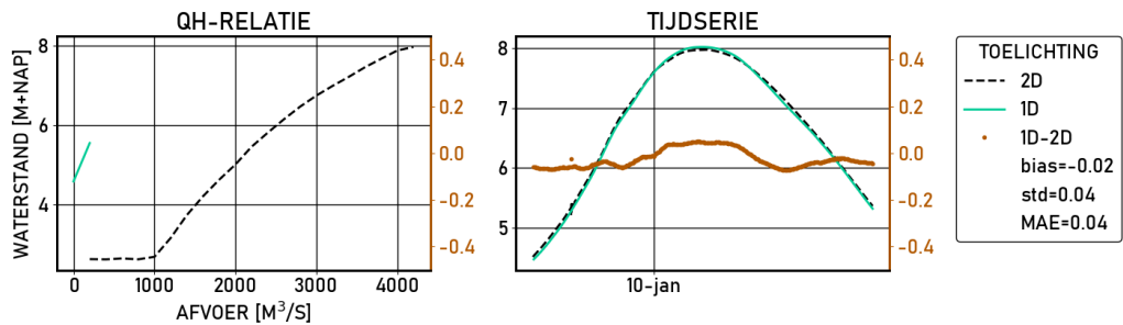
Figure 2.582 Tiel-Waal | figures | Validatie | D_6000 | stations
