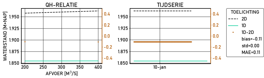
Figure 2.220 Olst | figures | Validatie | S_2000 | stations
