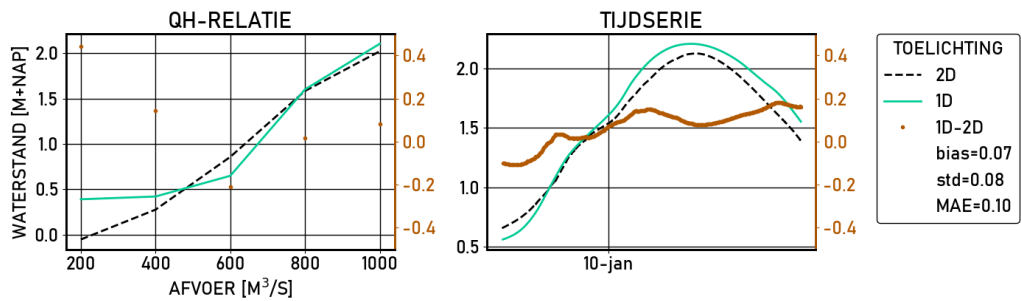
Figure 2.246 Katerveer | figures | Validatie | D_6000 | stations
