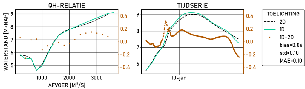
Figure 2.453 Amerongen-boven | figures | Validatie | D16000 | stations
