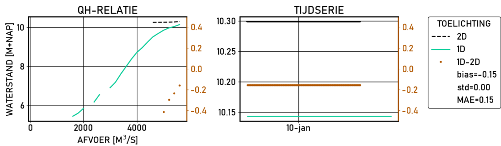
Figure 2.575 Dodewaard | figures | Validatie | S_8000 | stations
