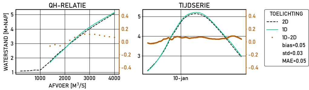
Figure 2.614 Zaltbommel | figures | Validatie | D_6000 | stations
