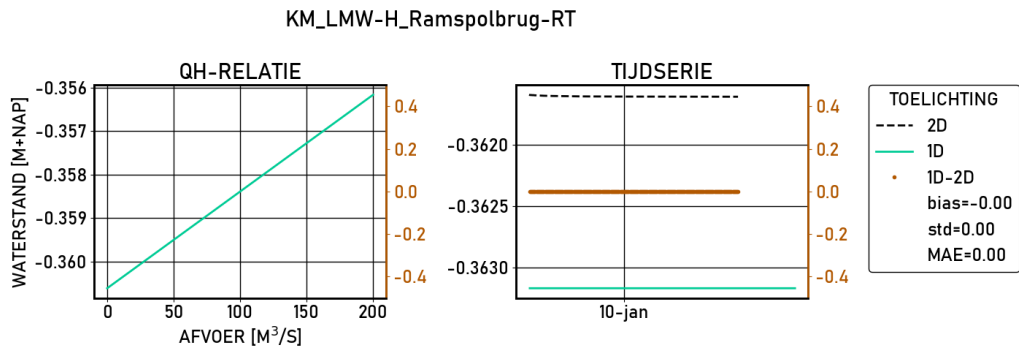
Figure 2.320 Ramspolbrug-RT | figures | Validatie | S__600 | stations
