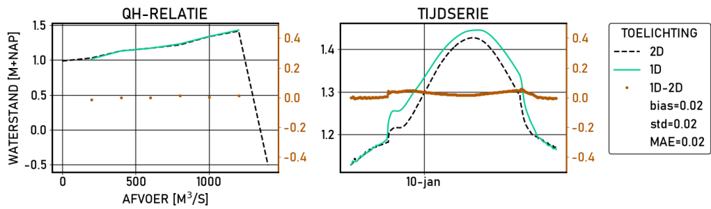
Figure 2.390 Krimpen-aan-de-Lek-g6 | figures | Validatie | D_6000 | stations
