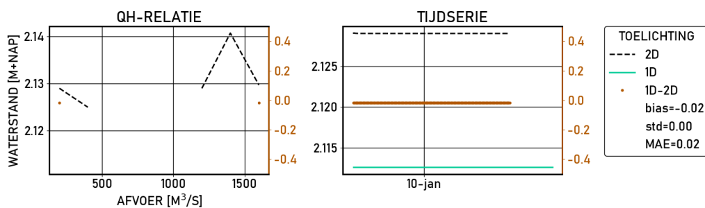
Figure 2.620 Zaltbommel | figures | Validatie | S_2000 | stations
