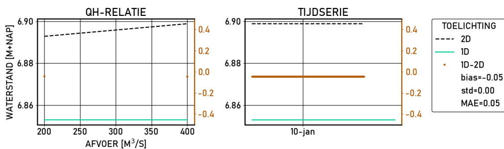
Figure 2.140 De-Steeg | figures | Validatie | S_2000 | stations
