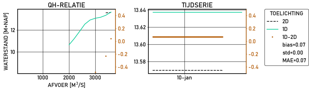
Figure 2.520 Looveer-g6 | figures | Validatie | S10000 | stations
