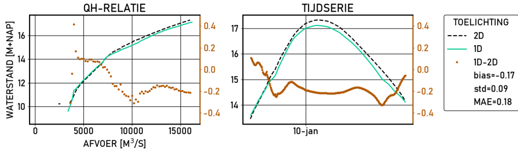
Figure 2.53 Lobith-haven | figures | Validatie | D16000 | stations
