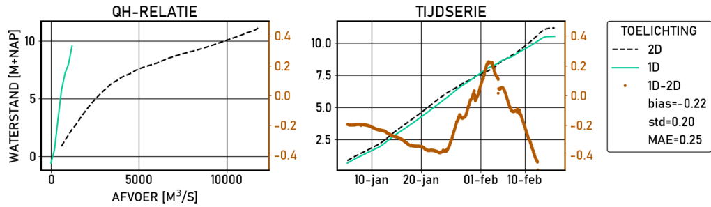
Figure 2.577 Tiel-Waal | figures | Ongekalibreerd | stations
