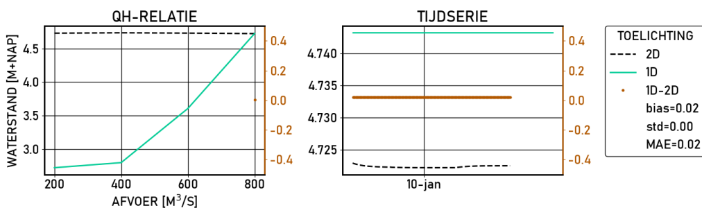
Figure 2.205 Deventer | figures | Validatie | S_4000 | stations
