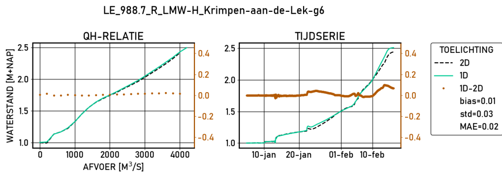
Figure 2.386 Krimpen-aan-de-Lek-g6 | figures | Kalibratie | stations
