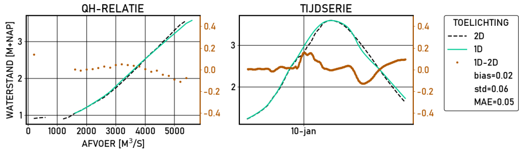
Figure 2.631 Vuren | figures | Validatie | D_8000 | stations
