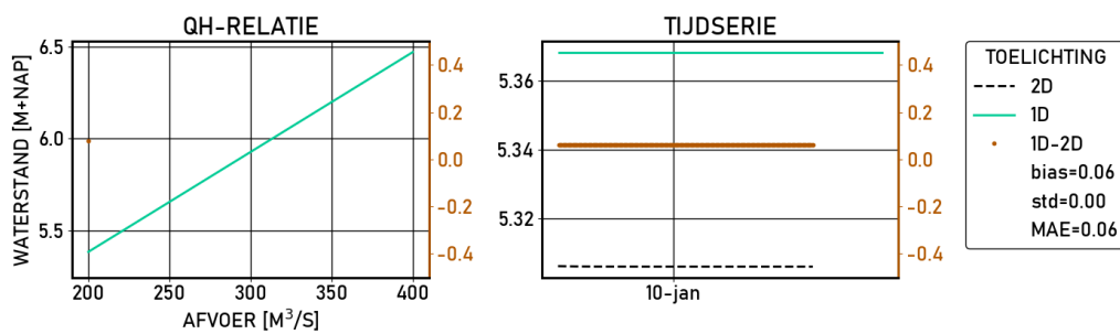
Figure 2.139 De-Steeg | figures | Validatie | S_1020 | stations
