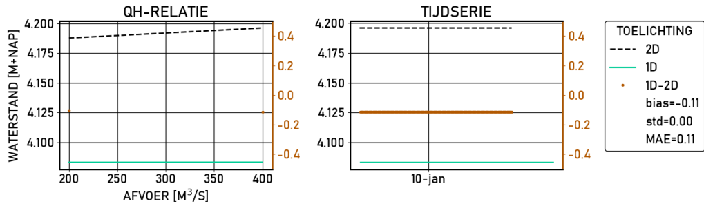
Figure 2.172 Zutphen-noord | figures | Validatie | S_2000 | stations
