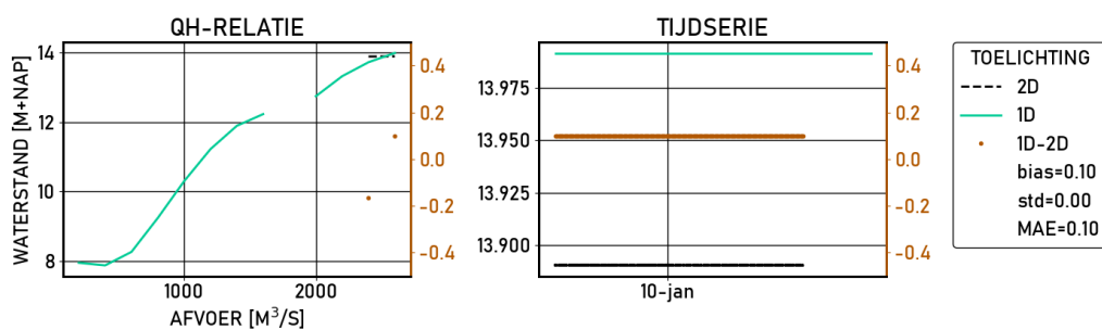
Figure 2.122 Westervoort-IJsseldijke | figures | Validatie | S16000 | stations
