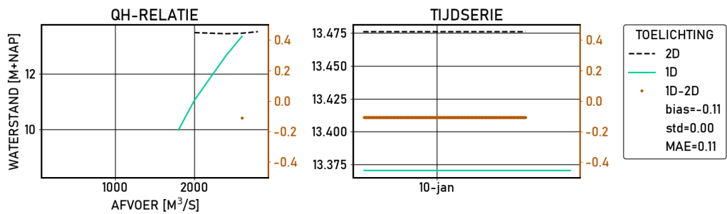
Figure 2.510 Pannerden | figures | Validatie | S_8000 | stations
