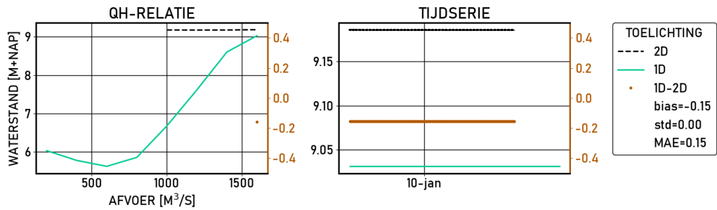
Figure 2.447 Grebbe | figures | Validatie | S_8000 | stations
