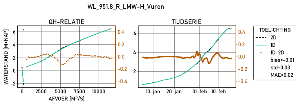
Figure 2.626 Vuren | figures | Kalibratie | stations
