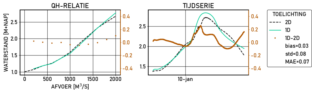
Figure 2.371 Schoonhoven | figures | Validatie | D10000 | stations
