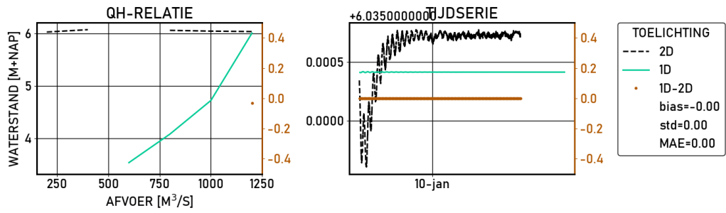
Figure 2.478 Amerongen-beneden | figures | Validatie | S_6000 | stations
