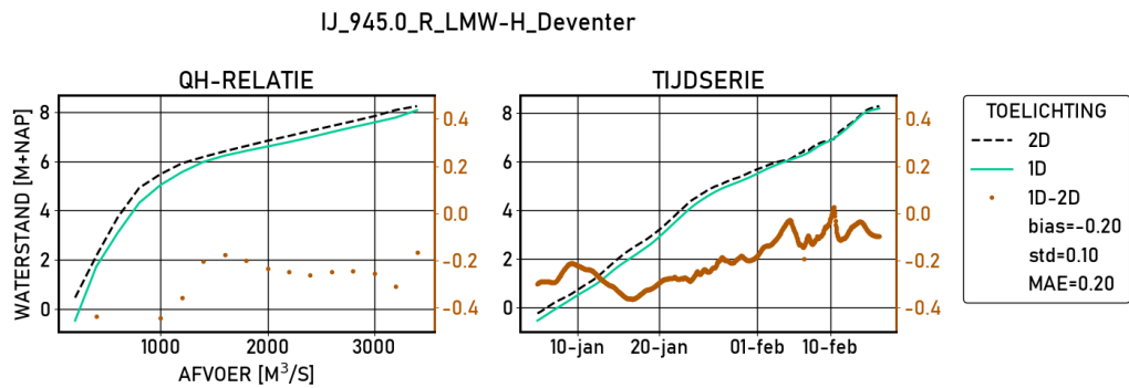
Figure 2.193 Deventer | figures | Ongekalibreerd | stations
