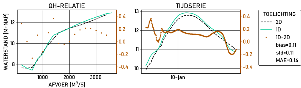
Figure 2.405 Driel-boven | figures | Validatie | D16000 | stations
