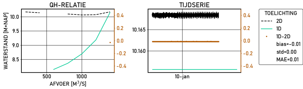
Figure 2.541 IJsselkop | figures | Validatie | S_4000 | stations
