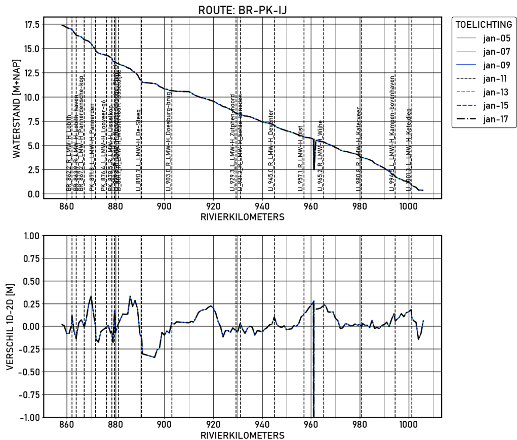
Figure 1.17 BR-PK-IJ | figures | Validatie | S13000 | Langsprofiel
