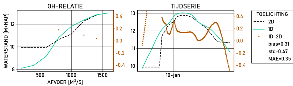
Figure 2.99 Hondsbroeksche-Pleij-IJ | figures | Validatie | D10000 | stations
