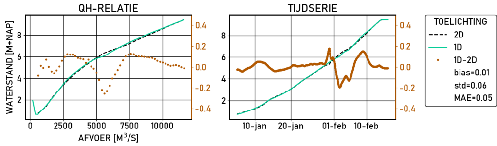
Figure 2.610 Zaltbommel | figures | Kalibratie | stations
