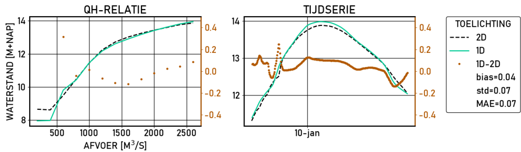
Figure 2.117 Westervoort-IJsseldijke | figures | Validatie | D16000 | stations
