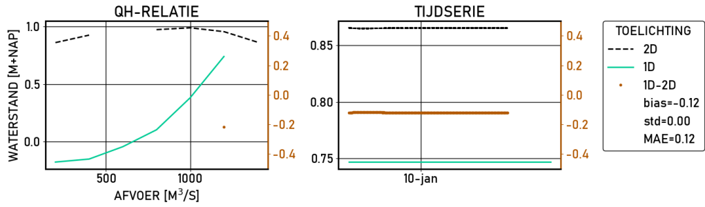
Figure 2.271 Kampen-bovenhaven | figures | Validatie | S_8000 | stations
