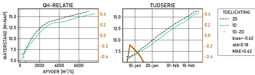
Figure 2.482 Pannerden | figures | Ongekalibreerd | stations
