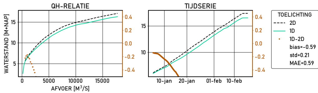
Figure 2.481 Pannerden | figures | Ongekalibreerd | stations
