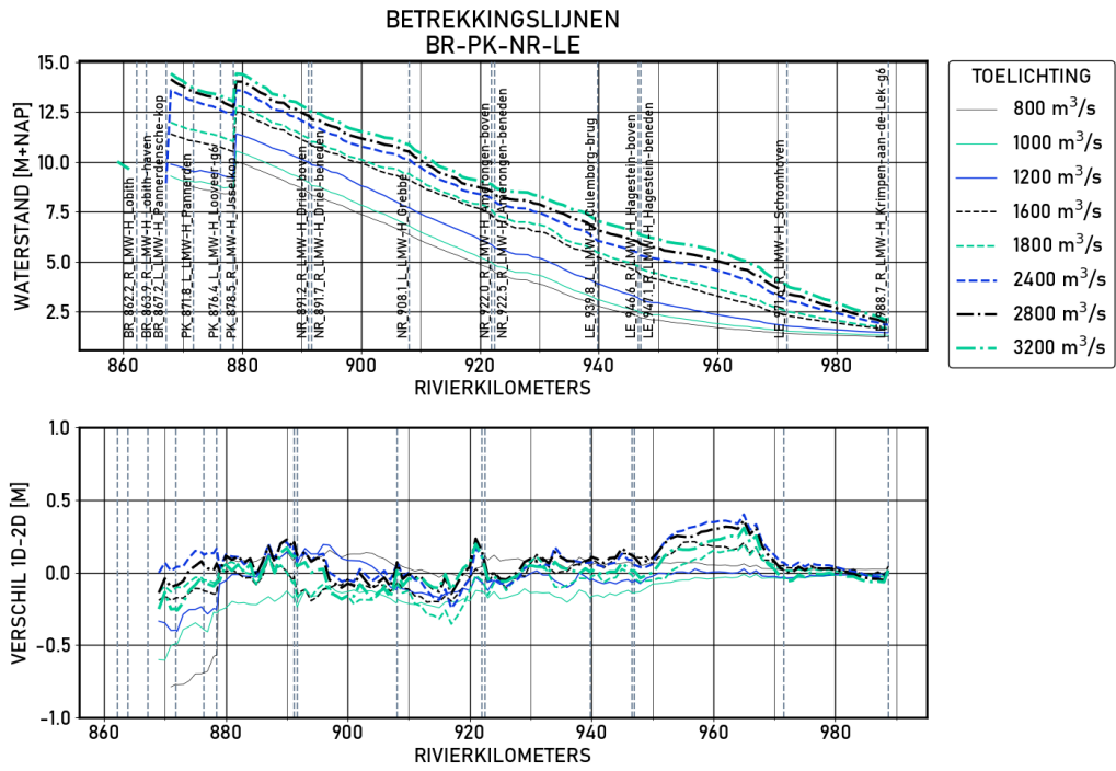
Figure 1.74 BR-PK-NR-LE | figures | Validatie | D16000 | Langsprofiel
