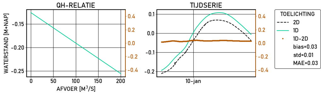
Figure 2.295 Ketelhaven | figures | Validatie | D_8000 | stations
