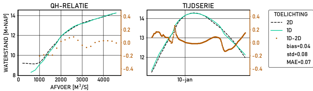
Figure 2.516 Looweer-g6 | figures | Validatie | D13000 | stations
