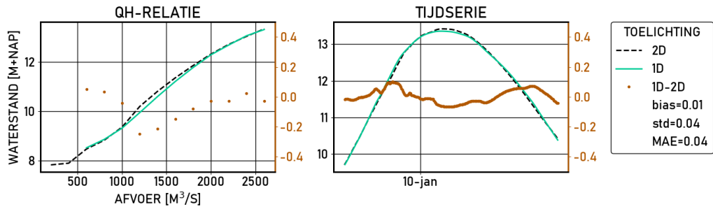
Figure 2.494 Pannerden | figures | Validatie | D_8000 | stations
