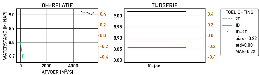
Figure 2.591 Tiel-Waal | figures | Validatie | S_8000 | stations
