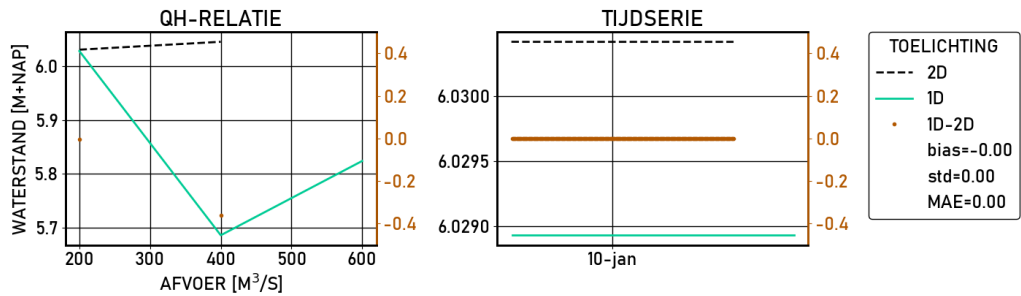
Figure 2.444 Grebbe | figures | Validatie | S_2000 | stations
