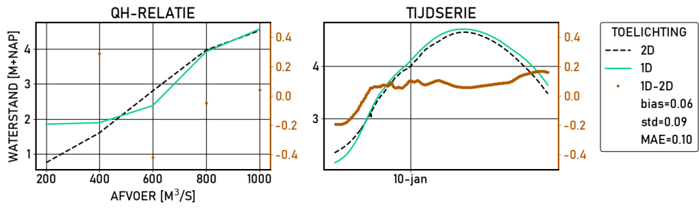
Figure 2.214 Olst | figures | Validatie | D_6000 | stations
