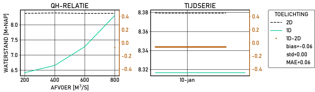
Figure 2.429 Driel-beneden | figures | Validatie | S_4000 | stations
