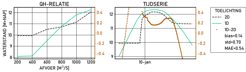
Figure 2.103 Hondsbroeksche-Pleij-IJ | figures | Validatie | D_8000 | stations
