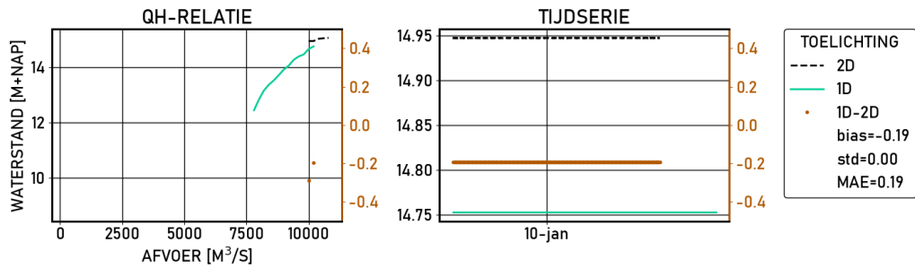
Figure 2.495 Pannerden | figures | Validatie | S10000 | stations
