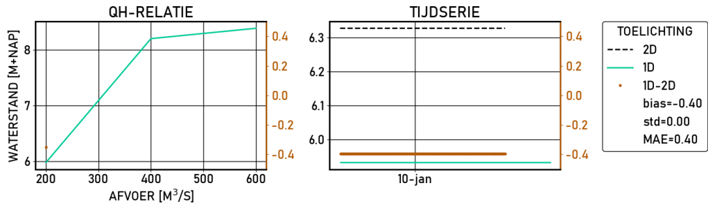
Figure 2.512 Pannerden | figures | Validatie | S__600 | stations
