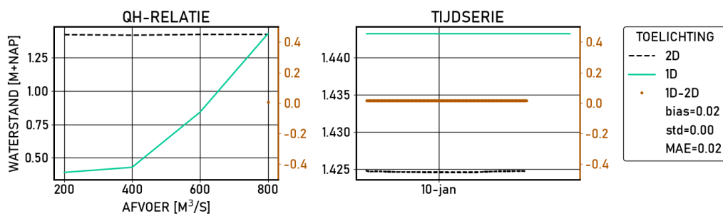
Figure 2.253 Katerveer | figures | Validatie | S_4000 | stations
