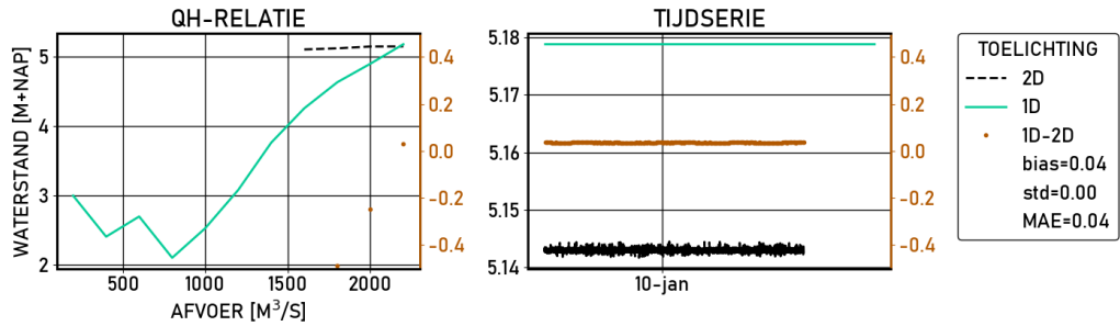
Figure 2.344 Hagestein-boven | figures | Validatie | S10000 | stations
