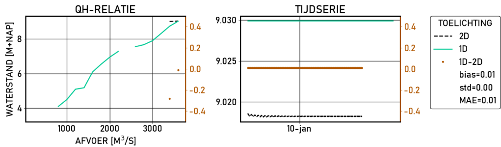
Figure 2.474 Amerongen-beneden | figures | Validatie | S1600 | stations
