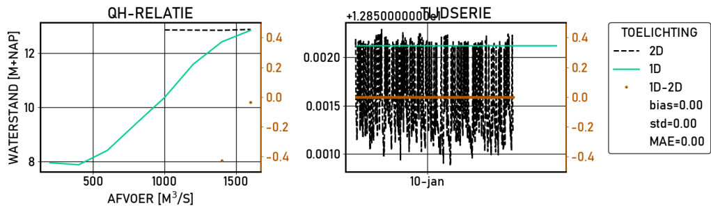
Figure 2.120 Westervoort-IJsseldijke | figures | Validatie | S10000 | stations
