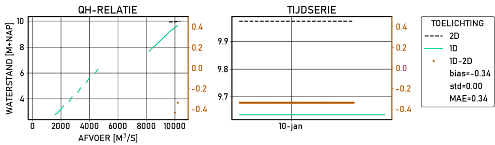
Figure 2.602 Sint-Andries-Waal-g6 | figures | Validatie | S16000 | stations
