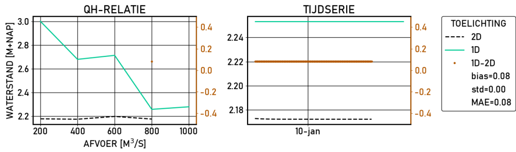
Figure 2.349 Hagestein-boven | figures | Validatie | S_4000 | stations
