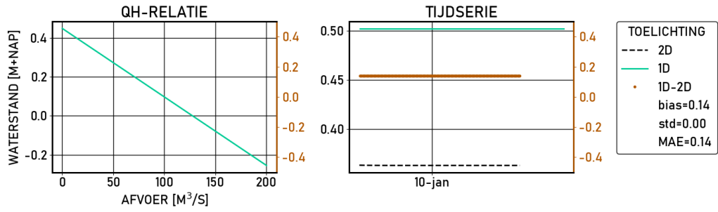
Figure 2.298 Ketelhaven | figures | Validatie | S16000 | stations
