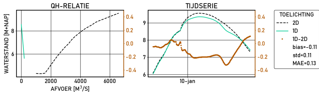
Figure 2.579 Tiel-Waal | figures | Validatie | D10000 | stations
