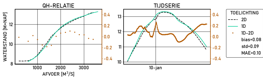
Figure 2.531 IJsselkop | figures | Validatie | D10000 | stations
