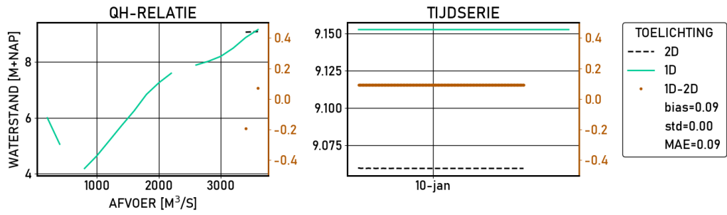
Figure 2.458 Amerongen-boven | figures | Validatie | S16000 | stations
