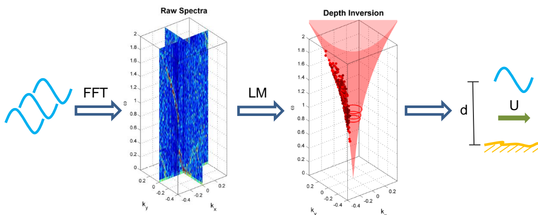
Figure 3.26 Workflow of XMFIt. The wave field in a computational cube is first decomposed into a spectrum via 3D-FFT (blue cross sections, 2 nd from the left). The energetic parts of the spectrum (red dots in red cone, 3 rd from the left) are then fitted to the Doppler shifted dispersion cone (red cone). This is done via a Levenberg-Marquard (LM) minimization. The best fit includes an estimate of the local depth and surface current vector.
