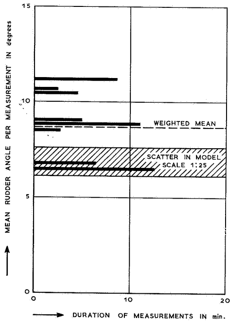
Figure 9. Mean rudder angle and duration of some prototype measurements with width of 100 m.
