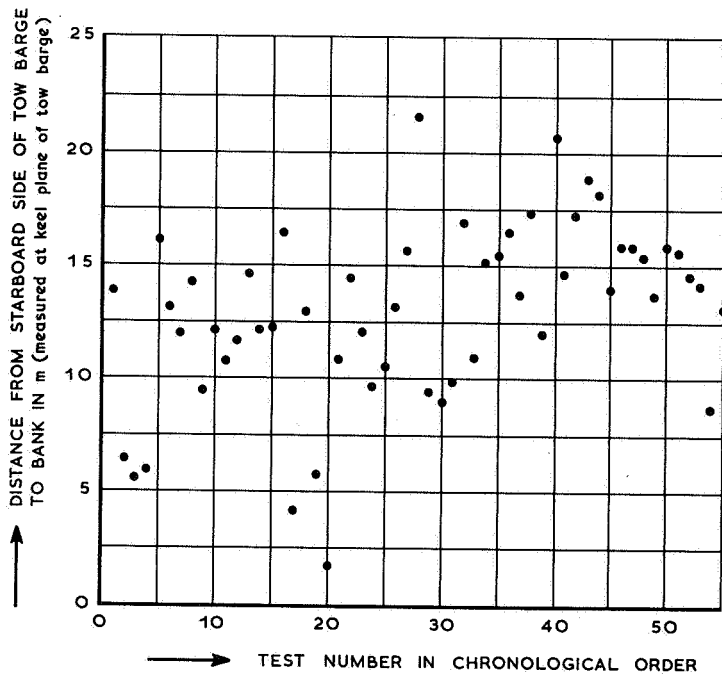
Figure 21. Passing manoeuvre in which tow barge is overtaken by push tow.
