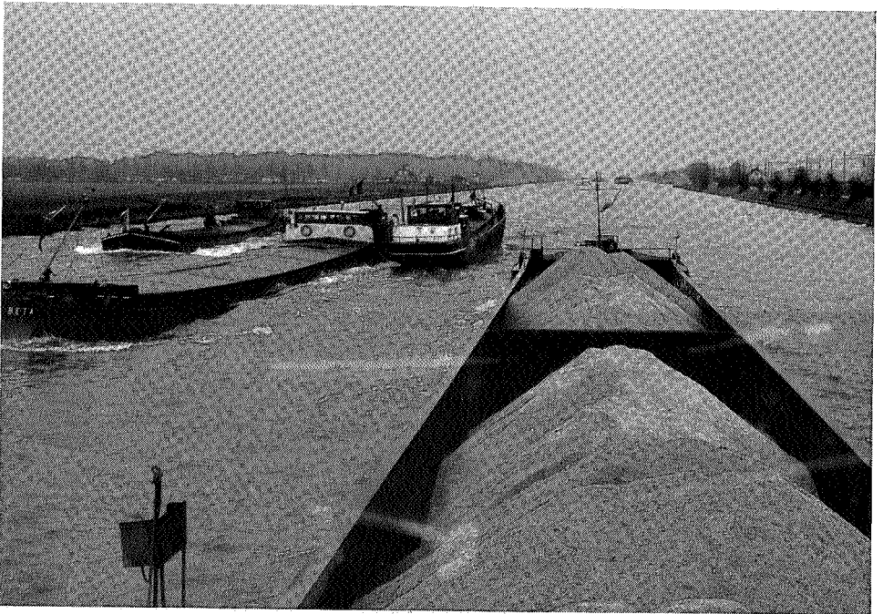
Photo 6. The space on either side of the fast vessel cannot be a norm for canal design.
