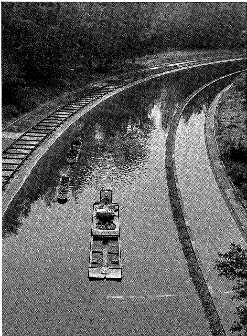
Photo 17. Overtaking manoeuvre of a push two and tow barge towed by a motor ship in the Eendracht bend of the Scheldt-Rhine Canal.
