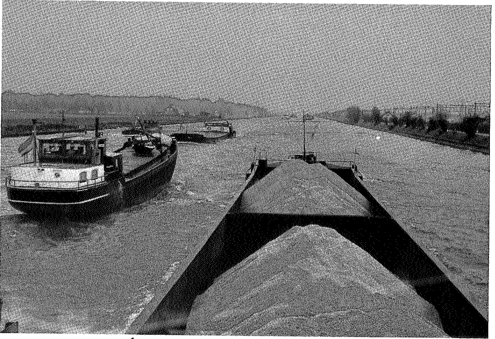
Photo 5. Single-barge push tow overtaken by an unladen fast ship, with two oncoming overtaking vessels.
