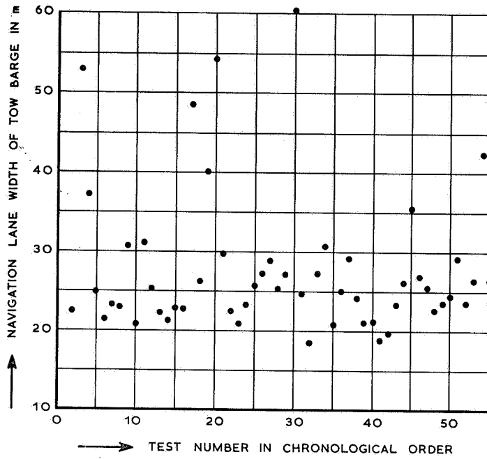
Figure 20. Passing manoeuvre in which tow barge is overtaken by push tow.
