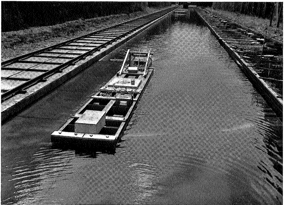
Photo 7. Automatically-steered push tow during study of directional stability in different canals, scale 1 : 25.
