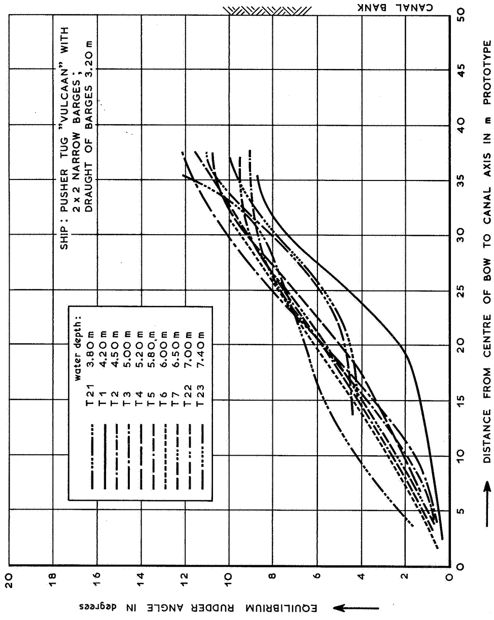
Figure 13. RUDDER ANGLE. Influence of depth (rectangular cross-section).
