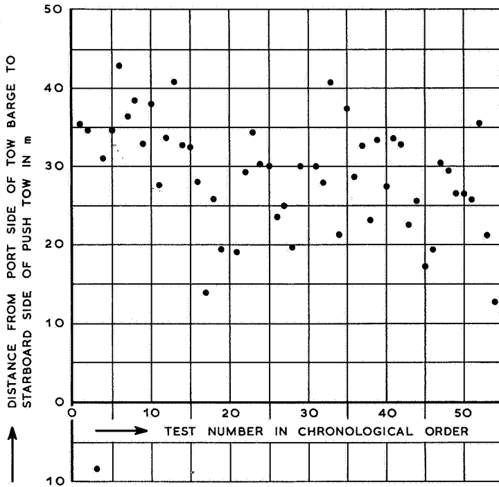
Figure 22. Passing manoeuvre in which tow barge is overtaken by push tow.
