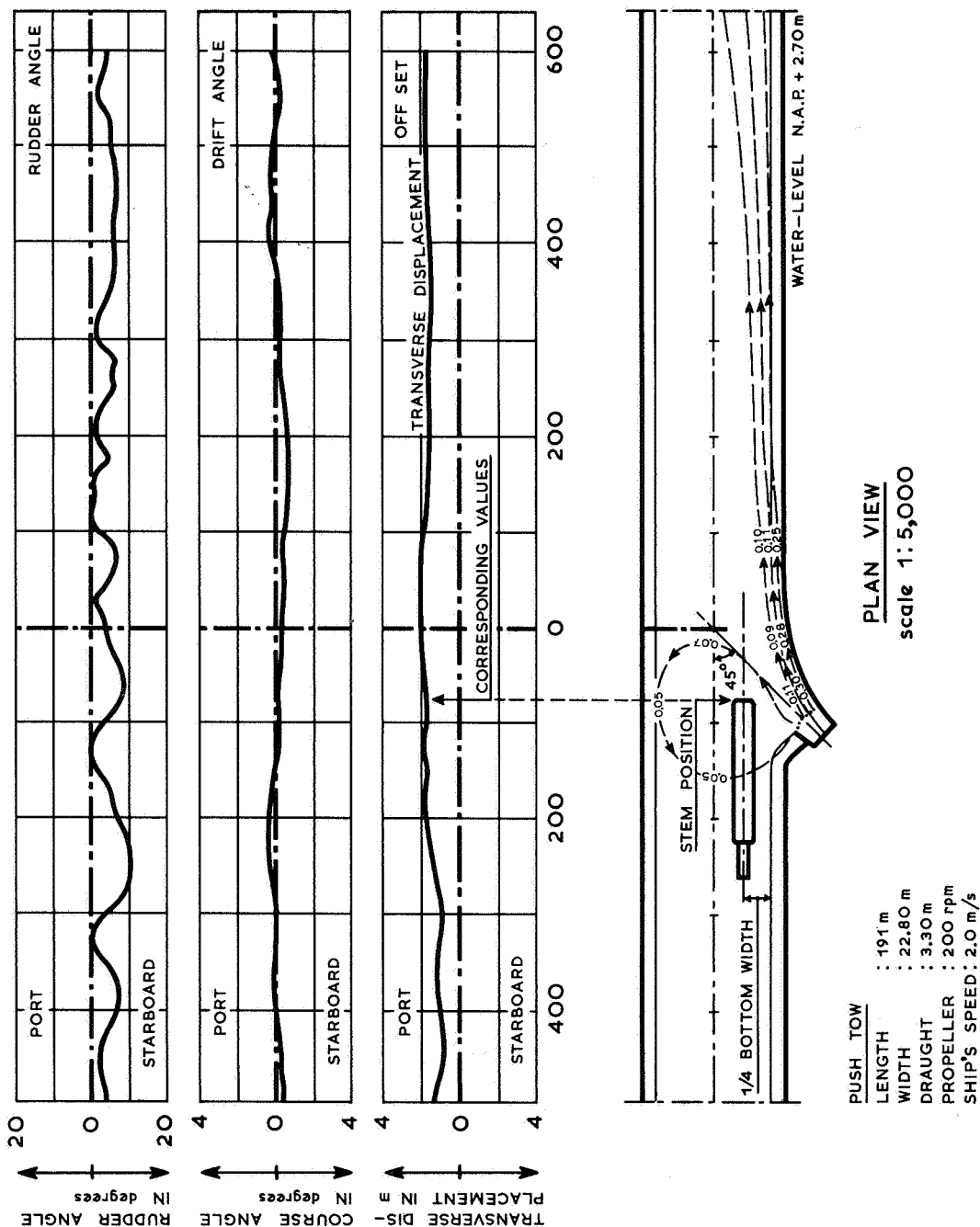
Figure 32. Behaviour of push tow near Beuningen outlet structure ( Q = 30 \text{ m}^3/\text{s} ).
