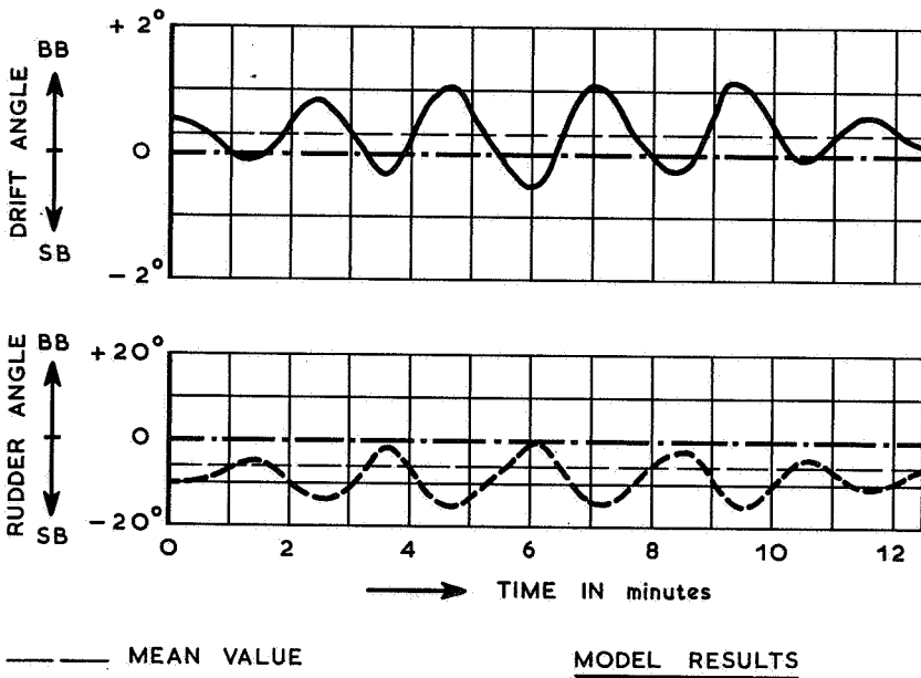
Figure 15. Behaviour of prototype push tow and model push tow with automatic steering.
