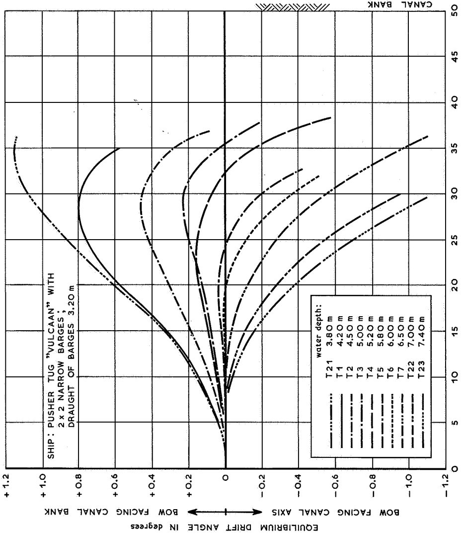
Figure 14. DRIFT ANGLE. Influence of depth (rectangular cross-section).
