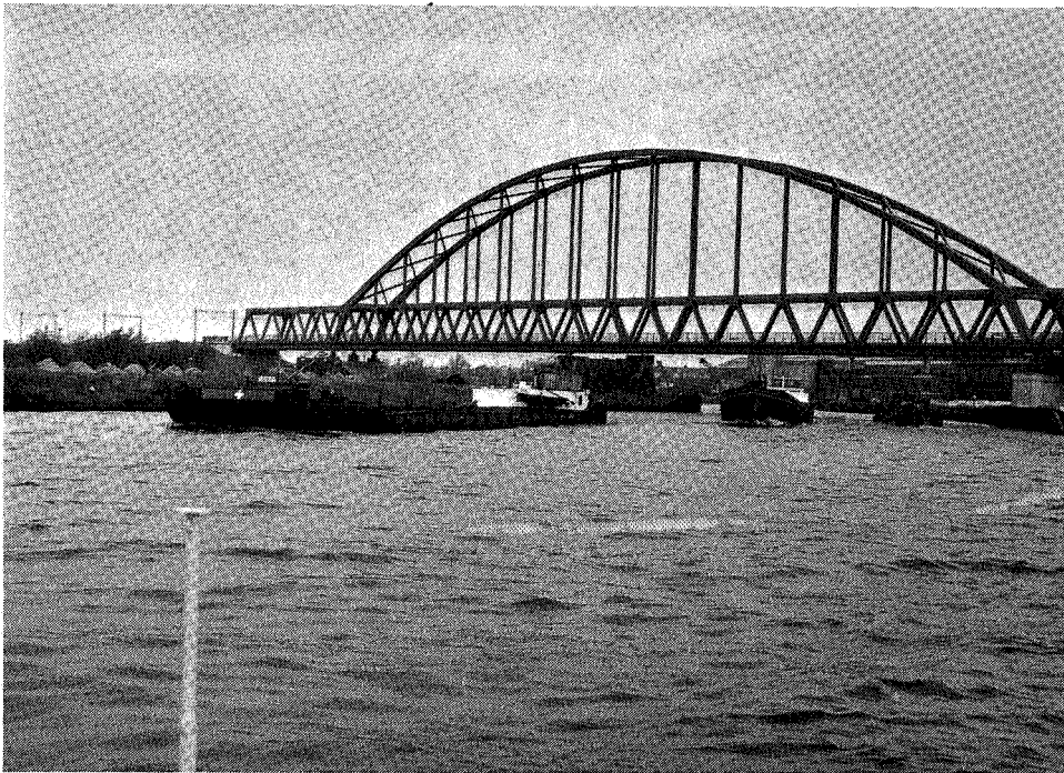
Photo 19. Demka bend — existing situation. An empty motor vessel and a push tow with one barge meet a laden motor ship.
