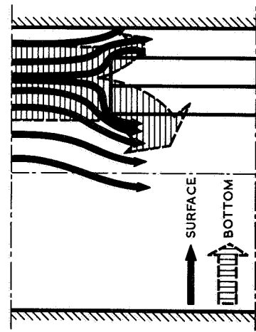
Figure 7. Flow pattern and water-level drop around a pusher tug in a canal.
