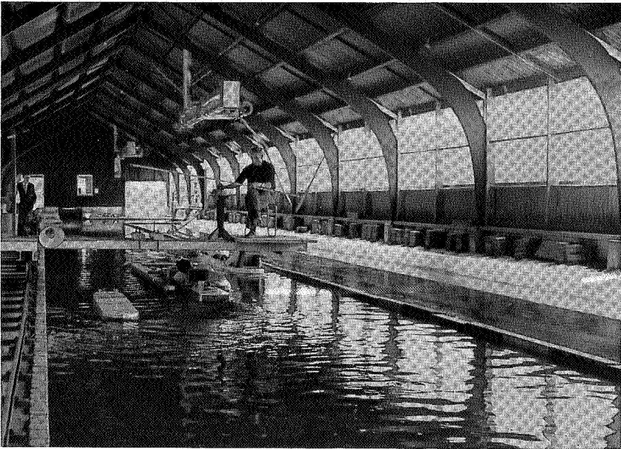
Photo 15. Model passing manoeuvre. The push tow and tow barge were steered by experienced skippers who determined the respective distances intuitively.
