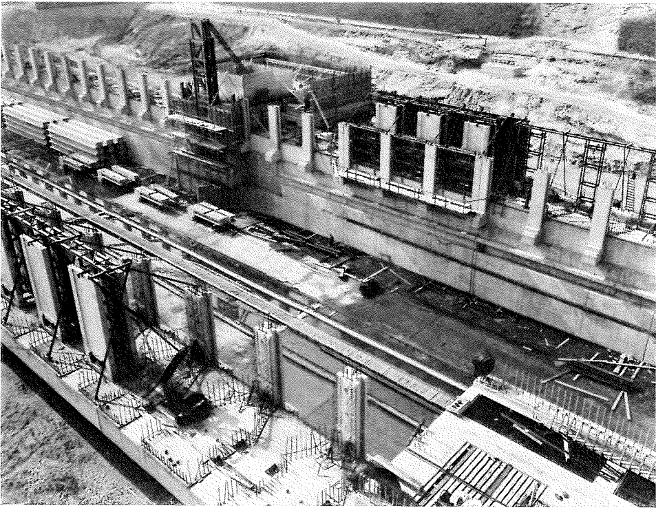
Photo 10. Wall construction using precast concrete components.
