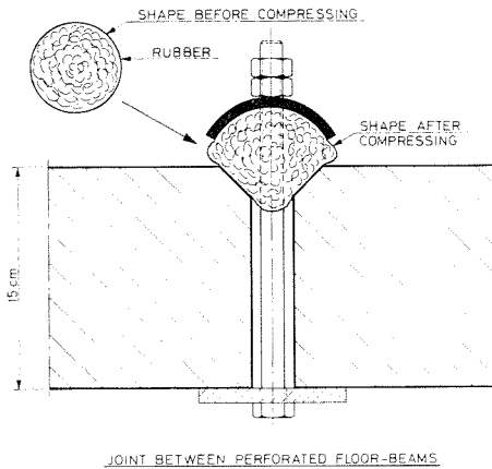
Figure 12. The joint between two beams.
