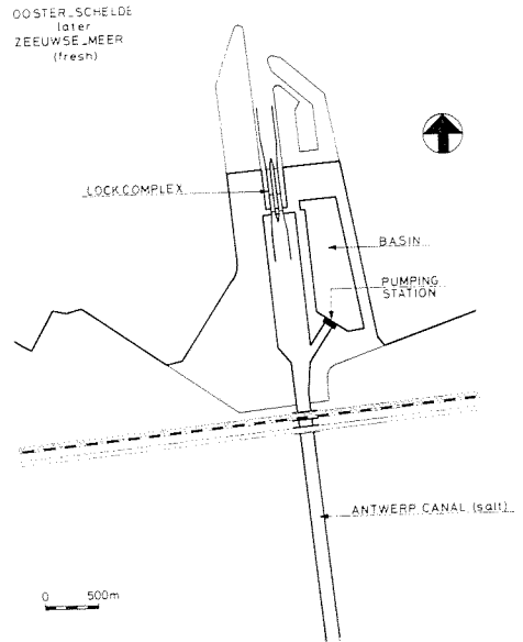
Figure 3. General view of the Kreekrak lock system.
