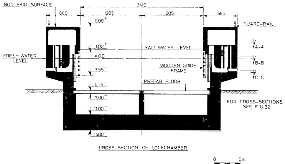
Figure 15. Cross-section of lock chamber.
