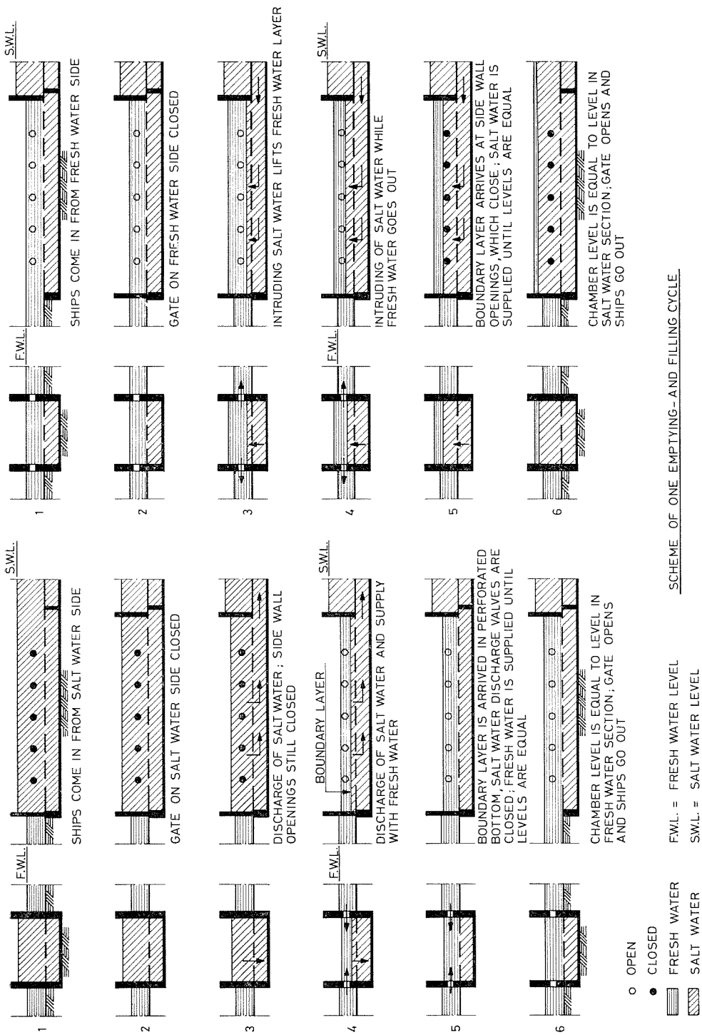
Figure 7. System of complete exchange of closed lock chamber.
