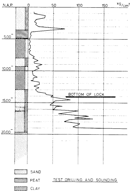
Figure 9. Results of test drilling.
