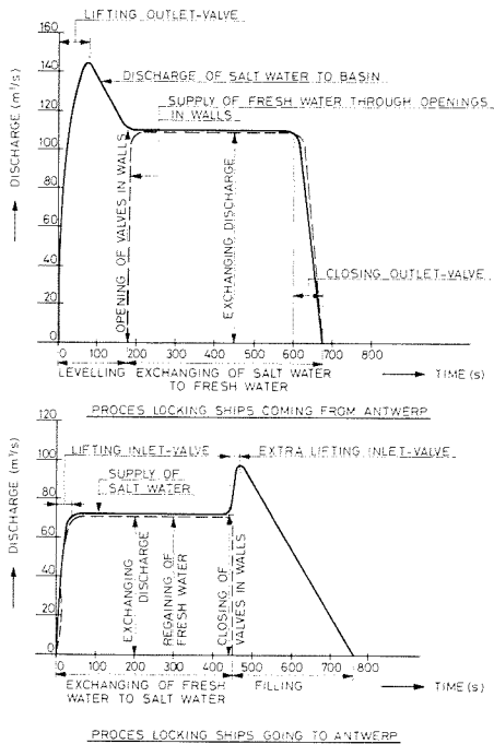
Figure 22. Locking procedure in the Kreekrak locks.
